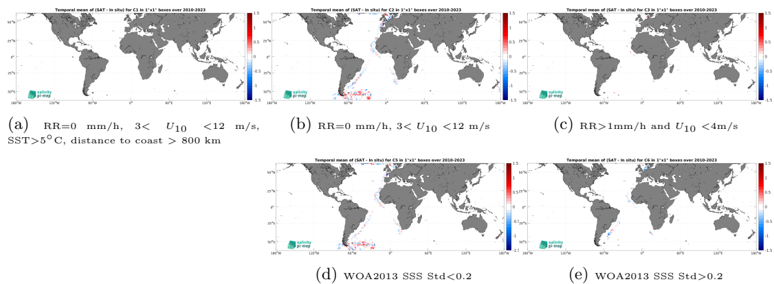
Figure 14: Temporal mean gridded over spatial boxes of size 1^\circ \times 1^\circ of \Delta SSS (SMOS SSS L3 v9 - 9 Days (CATDS-CEC-LOCEAN) - TSG (Polarstern)) for 5 different subdatasets corresponding to:RR=0 mm/h, 3 < U_{10} < 12 m/s, SST >5^\circ C, distance to coast > 800 km (a), RR=0 mm/h, 3 < U_{10} < 12 m/s (b), RR >1 mm/h and U_{10} < 4 m/s (c), WOA2013 SSS Std <0.2 (d), WOA2013 SSS Std >0.2 (e).
