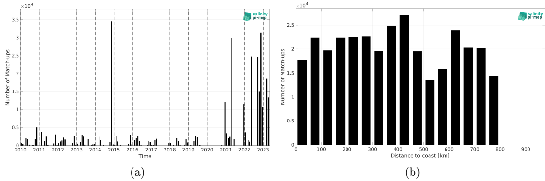
Figure 2: Number of match-ups between TSG (Polarstern) and SMOS SSS L3 v9 - 9 Days (CATDS-CEC-LOCEAN) SSS as a function of time (a) and as function of the distance to coast (b) over the SMOS coastal zone (<800km) 60N-60S Pi-MEP region and for the full satellite product period.
