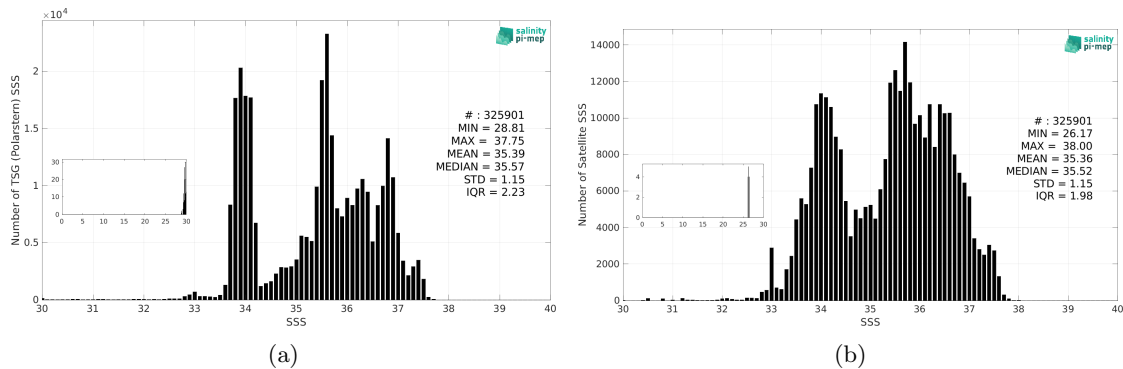
Figure 3: Histograms of SSS from TSG (Polarstern) (a) and SMOS SSS L3 v9 - 9 Days (CATDS-CEC-LOCEAN) (b) considering all match-up pairs per bins of 0.1 over the SMOS coastal zone (<800km) 60N-60S Pi-MEP region and for the full satellite product period.
