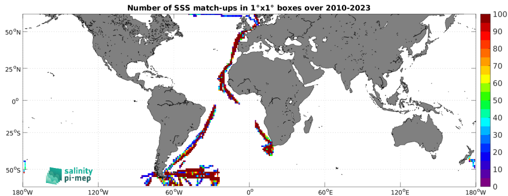
Figure 5: Number of SSS match-ups between TSG (Polarstern) SSS and the SMOS SSS L3 v9 - 9 Days (CATDS-CEC-LOCEAN) SSS product for the SMOS coastal zone (<800km) 60N-60S Pi-MEP region over 1^\circ \times 1^\circ boxes and for the full satellite product period.
