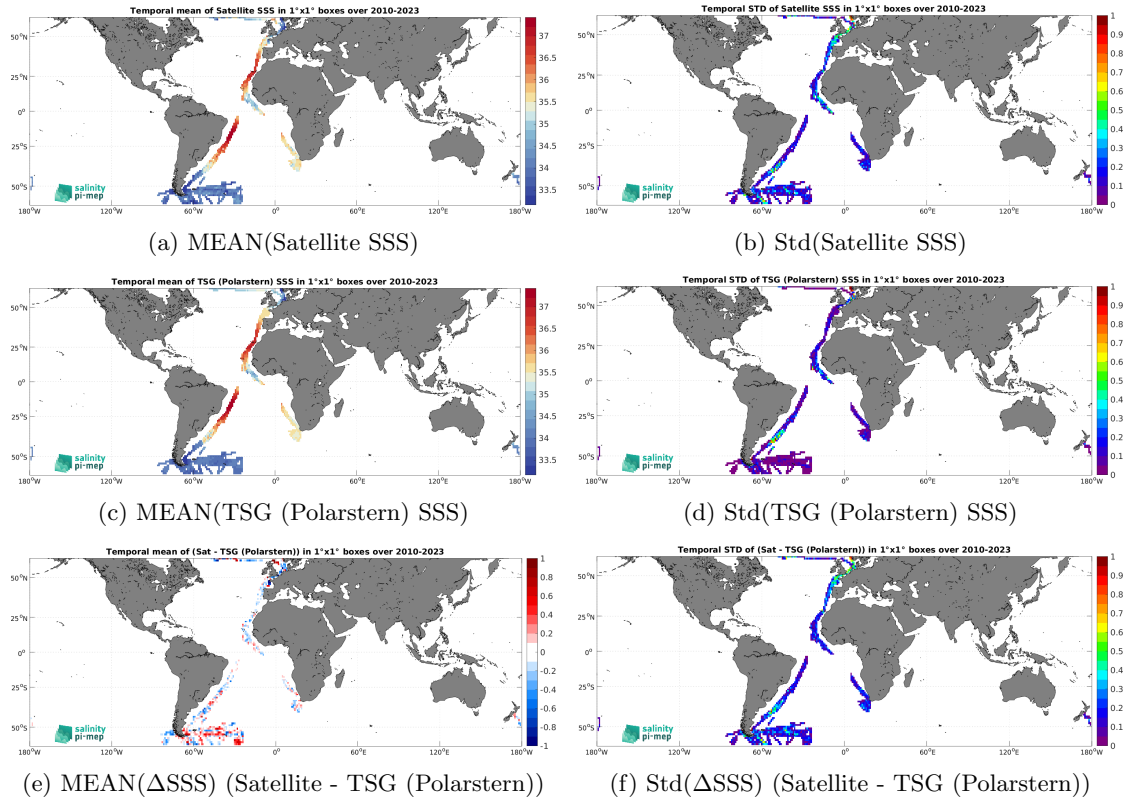
Figure 7: Temporal mean (left) and Std (right) of SSS from SMOS SSS L3 v9 - 9 Days (CATDS-CEC-LOCEAN) (top), TSG (Polarstern) (middle), and of \Delta SSS (Satellite - TSG (Polarstern)). Only match-up pairs are used to generate these maps.
