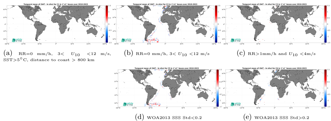
Figure 14: Temporal mean gridded over spatial boxes of size 1^\circ \times 1^\circ of \Delta\text{SSS} (SMOS SSS L3 v9 - 9 Days (CATDS-CEC-LOCEAN) - TSG (Polarstern)) for 5 different subdatasets corresponding to:RR=0 mm/h, 3 < U_{10} < 12 m/s, SST >5^\circ\text{C} , distance to coast > 800 km (a), RR=0 mm/h, 3 < U_{10} < 12 m/s (b), RR >1 mm/h and U_{10} < 4 m/s (c), WOA2013 SSS Std <0.2 (d), WOA2013 SSS Std >0.2 (e).
