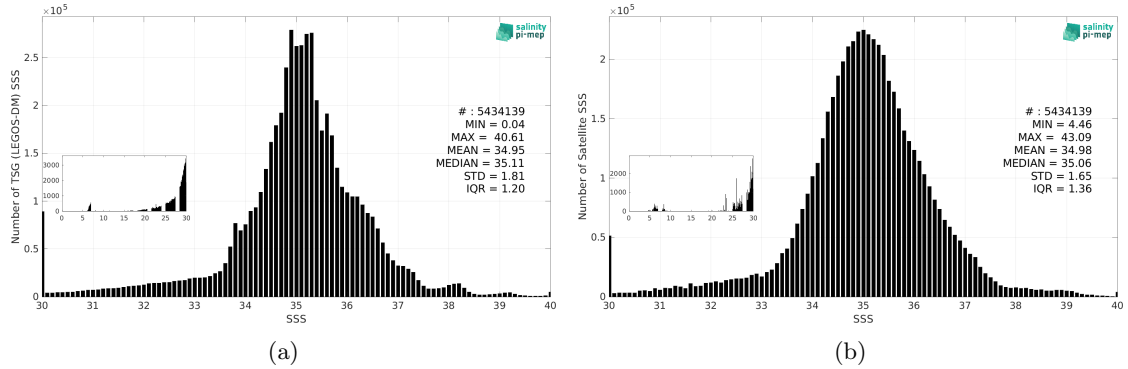
Figure 3: Histograms of SSS from TSG (LEGOS-DM) (a) and SMOS SSS L3 v9 - 9 Days (CATDS-CEC-LOCEAN) (b) considering all match-up pairs per bins of 0.1 over the SMOS coastal zone (<800km) 60N-60S Pi-MEP region and for the full satellite product period.
