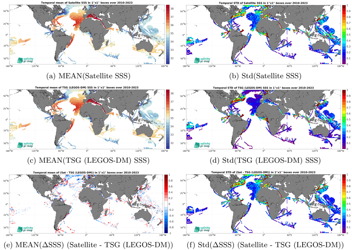
Figure 7: Temporal mean (left) and Std (right) of SSS from SMOS SSS L3 v9 - 9 Days (CATDS-CEC-LOCEAN) (top), TSG (LEGOS-DM) (middle), and of \Delta SSS (Satellite - TSG (LEGOS-DM)). Only match-up pairs are used to generate these maps.
