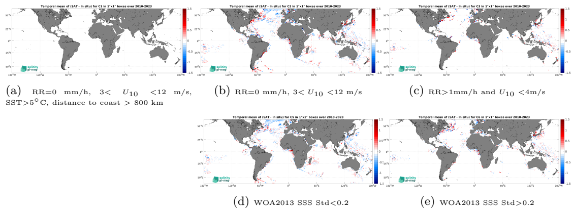
Figure 14: Temporal mean gridded over spatial boxes of size 1^\circ \times 1^\circ of \Delta\text{SSS} (SMOS SSS L3 v9 - 9 Days (CATDS-CEC-LOCEAN) - TSG (LEGOS-DM)) for 5 different subdatasets corresponding to:RR=0 mm/h, 3 < U_{10} < 12 m/s, SST > 5°C, distance to coast > 800 km (a), RR=0 mm/h, 3 < U_{10} < 12 m/s (b), RR > 1mm/h and U_{10} < 4 m/s (c), WOA2013 SSS Std < 0.2 (d), WOA2013 SSS Std > 0.2 (e).
