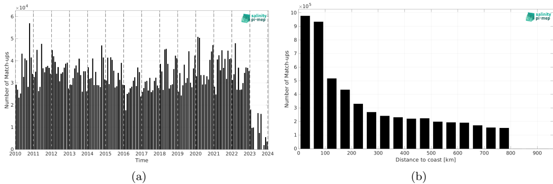
Figure 2: Number of match-ups between TSG (LEGOS-DM) and SMOS SSS L3 v9 - 9 Days (CATDS-CEC-LOCEAN) SSS as a function of time (a) and as function of the distance to coast (b) over the SMOS coastal zone (<800km) 60N-60S Pi-MEP region and for the full satellite product period.
