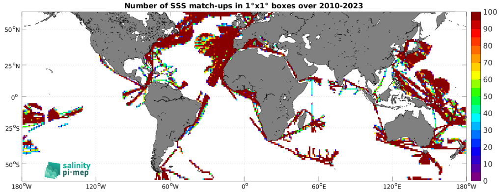
Figure 5: Number of SSS match-ups between TSG (LEGOS-DM) SSS and the SMOS SSS L3 v9 - 9 Days (CATDS-CEC-LOCEAN) SSS product for the SMOS coastal zone (<800km) 60N-60S Pi-MEP region over 1^\circ \times 1^\circ boxes and for the full satellite product period.
