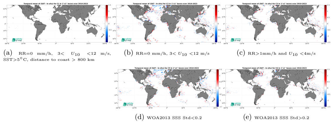
Figure 14: Temporal mean gridded over spatial boxes of size 1^\circ \times 1^\circ of \Delta SSS (SMOS SSS L3 v9 - 9 Days (CATDS-CEC-LOCEAN) - TSG (LEGOS-DM)) for 5 different subdatasets corresponding to:RR=0 mm/h, 3 < U_{10} < 12 m/s, SST >5^\circ C, distance to coast > 800 km (a), RR=0 mm/h, 3 < U_{10} < 12 m/s (b), RR >1 mm/h and U_{10} < 4 m/s (c), WOA2013 SSS Std <0.2 (d), WOA2013 SSS Std >0.2 (e).
