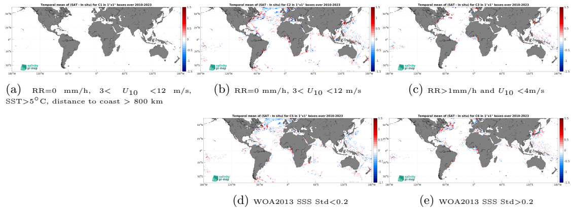
Figure 12: Temporal mean gridded over spatial boxes of size 1^\circ \times 1^\circ of \Delta SSS (SMOS SSS L3 v9 - 9 Days (CATDS-CEC-LOCEAN) - TSG (LEGOS-DM)) for 5 different subdatasets corresponding to:RR=0 mm/h, 3 < U_{10} < 12 m/s, SST >5^\circ C, distance to coast > 800 km (a), RR=0 mm/h, 3 < U_{10} < 12 m/s (b), RR >1 mm/h and U_{10} < 4 m/s (c), WOA2013 SSS Std <0.2 (d), WOA2013 SSS Std >0.2 (e).
