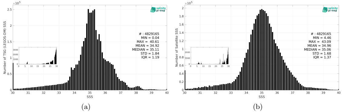
Figure 2: Histograms of SSS from TSG (LEGOS-DM) (a) and SMOS SSS L3 v9 - 9 Days (CATDS-CEC-LOCEAN) (b) considering all match-up pairs per bins of 0.1 over the SMOS coastal zone (<800km) 60N-60S Pi-MEP region and for the full satellite product period.
