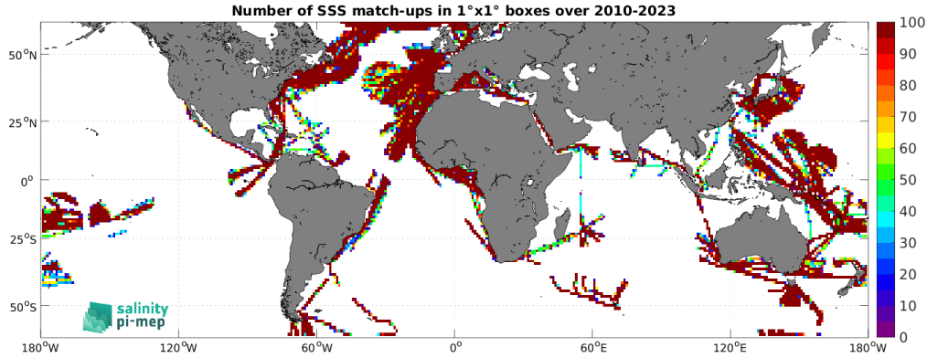
Figure 4: Number of SSS match-ups between TSG (LEGOS-DM) SSS and the SMOS SSS L3 v9 - 9 Days (CATDS-CEC-LOCEAN) SSS product for the SMOS coastal zone (<800km) 60N-60S Pi-MEP region over 1^\circ \times 1^\circ boxes and for the full satellite product period.
