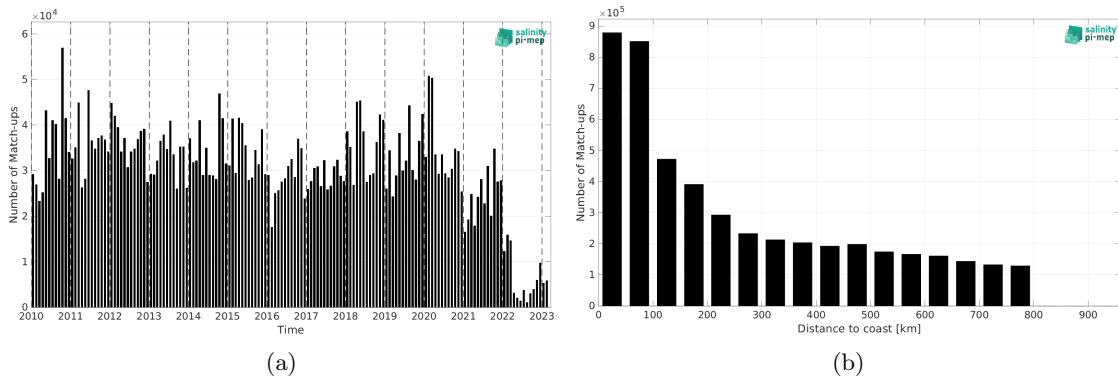
Figure 1: Number of match-ups between TSG (LEGOS-DM) and SMOS SSS L3 v9 - 9 Days (CATDS-CEC-LOCEAN) SSS as a function of time (a) and as function of the distance to coast (b) over the SMOS coastal zone (<800km) 60N-60S Pi-MEP region and for the full satellite product period.
