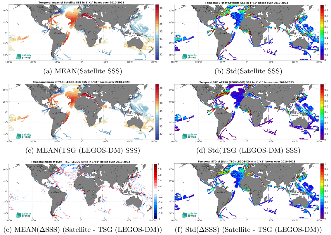
Figure 6: Temporal mean (left) and Std (right) of SSS from SMOS SSS L3 v9 - 9 Days (CATDS-CEC-LOCEAN) (top), TSG (LEGOS-DM) (middle), and of \Delta SSS (Satellite - TSG (LEGOS-DM)). Only match-up pairs are used to generate these maps.
