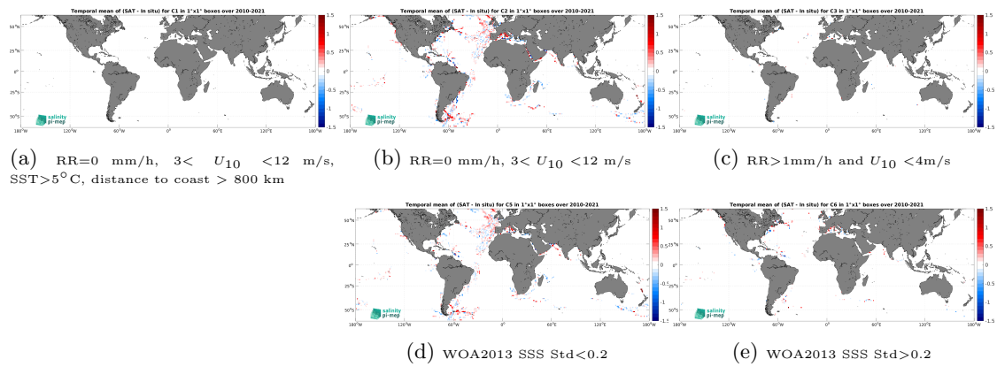
Figure 12: Temporal mean gridded over spatial boxes of size 1^\circ \times 1^\circ of \Delta SSS (SMOS SSS L3 v9 - 9 Days (CATDS-CEC-LOCEAN) - TSG (GOSUD-Sailing-ship)) for 5 different subdatasets corresponding to: RR=0 mm/h, 3 < U_{10} < 12 m/s, SST > 5^\circ\text{C} , distance to coast > 800 km (a), RR=0 mm/h, 3 < U_{10} < 12 m/s (b), RR > 1 mm/h and U_{10} < 4 m/s (c), WOA2013 SSS Std < 0.2 (d), WOA2013 SSS Std > 0.2 (e).
