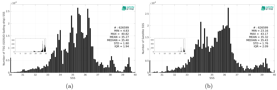
Figure 2: Histograms of SSS from TSG (GOSUD-Sailing-ship) (a) and SMOS SSS L3 v9 - 9 Days (CATDS-CEC-LOCEAN) (b) considering all match-up pairs per bins of 0.1 over the SMOS coastal zone (<800km) 60N-60S Pi-MEP region and for the full satellite product period.
