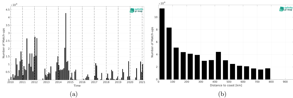
Figure 1: Number of match-ups between TSG (GOSUD-Sailing-ship) and SMOS SSS L3 v9 - 9 Days (CATDS-CEC-LOCEAN) SSS as a function of time (a) and as function of the distance to coast (b) over the SMOS coastal zone (<800km) 60N-60S Pi-MEP region and for the full satellite product period.
