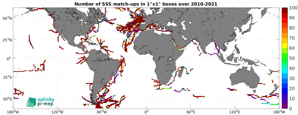
Figure 4: Number of SSS match-ups between TSG (GOSUD-Sailing-ship) SSS and the SMOS SSS L3 v9 - 9 Days (CATDS-CEC-LOCEAN) SSS product for the SMOS coastal zone ( <800\text{km} ) 60N-60S Pi-MEP region over 1^\circ \times 1^\circ boxes and for the full satellite product period.
