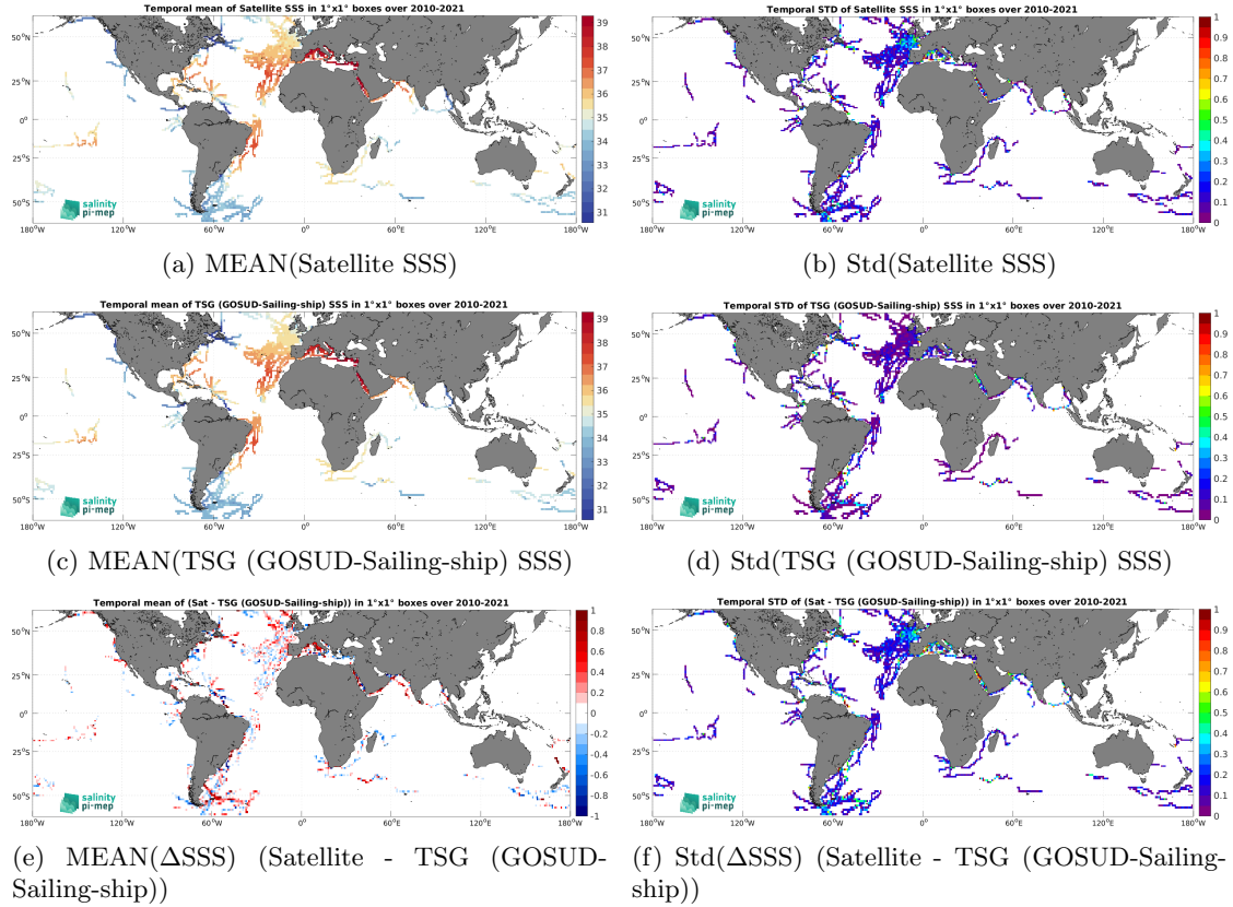
Figure 6: Temporal mean (left) and Std (right) of SSS from SMOS SSS L3 v9 - 9 Days (CATDS-CEC-LOCEAN) (top), TSG (GOSUD-Sailing-ship) (middle), and of \Delta\text{SSS} (Satellite - TSG (GOSUD-Sailing-ship)). Only match-up pairs are used to generate these maps.
