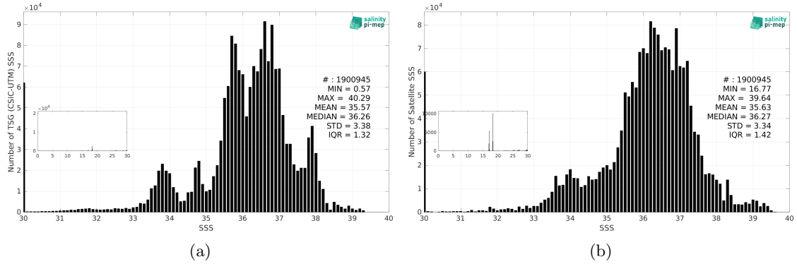
Figure 3: Histograms of SSS from TSG (CSIC-UTM) (a) and SMOS SSS L3 v9 - 9 Days (CATDS-CEC-LOCEAN) (b) considering all match-up pairs per bins of 0.1 over the SMOS coastal zone (<800km) 60N-60S Pi-MEP region and for the full satellite product period.
