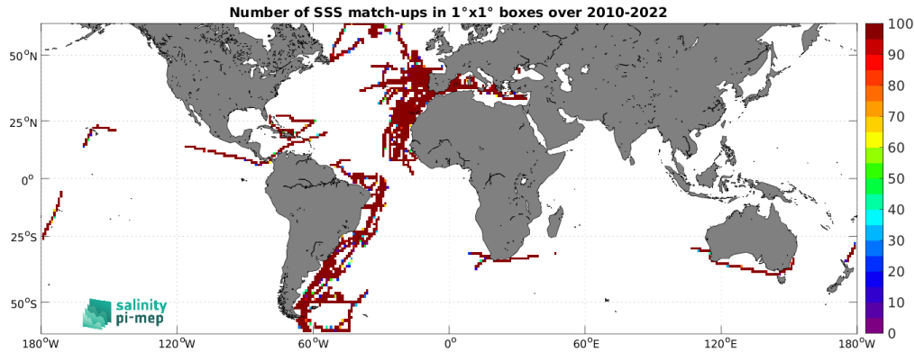
Figure 5: Number of SSS match-ups between TSG (CSIC-UTM) SSS and the SMOS SSS L3 v9 - 9 Days (CATDS-CEC-LOCEAN) SSS product for the SMOS coastal zone (<800km) 60N-60S Pi-MEP region over 1^\circ \times 1^\circ boxes and for the full satellite product period.
