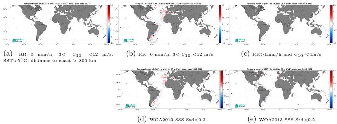
Figure 14: Temporal mean gridded over spatial boxes of size 1^\circ \times 1^\circ of \Delta\text{SSS} (SMOS SSS L3 v9 - 9 Days (CATDS-CEC-LOCEAN) - TSG (CSIC-UTM)) for 5 different subdatasets corresponding to:RR=0 mm/h, 3 < U_{10} < 12 m/s, SST >5^\circ\text{C} , distance to coast > 800 km (a), RR=0 mm/h, 3 < U_{10} < 12 m/s (b), RR >1 mm/h and U_{10} < 4 m/s (c), WOA2013 SSS Std <0.2 (d), WOA2013 SSS Std >0.2 (e).
