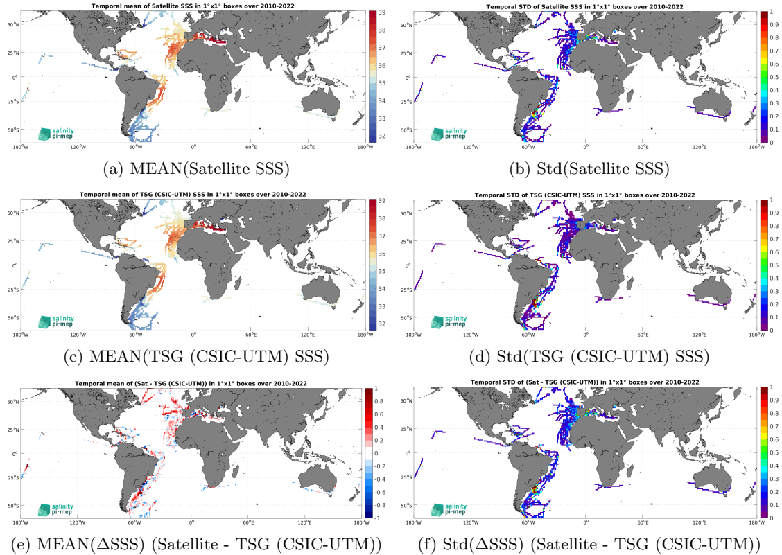
Figure 7: Temporal mean (left) and Std (right) of SSS from SMOS SSS L3 v9 - 9 Days (CATDS-CEC-LOCEAN) (top), TSG (CSIC-UTM) (middle), and of \Delta\text{SSS} (Satellite - TSG (CSIC-UTM)). Only match-up pairs are used to generate these maps.
