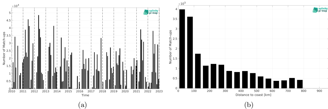
Figure 2: Number of match-ups between TSG (CSIC-UTM) and SMOS SSS L3 v9 - 9 Days (CATDS-CEC-LOCEAN) SSS as a function of time (a) and as function of the distance to coast (b) over the SMOS coastal zone (<800km) 60N-60S Pi-MEP region and for the full satellite product period.
