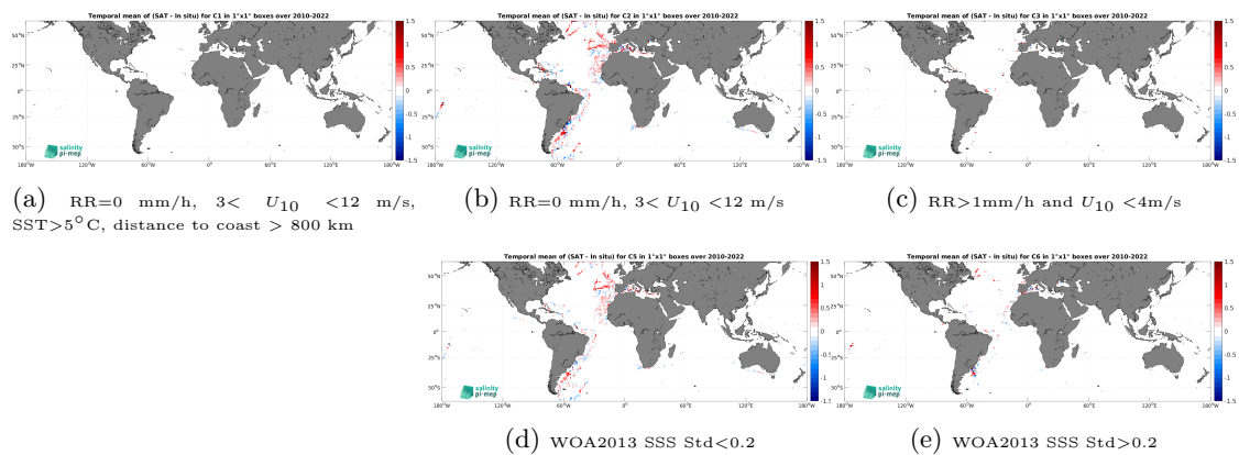
Figure 14: Temporal mean gridded over spatial boxes of size 1^\circ \times 1^\circ of \Delta SSS (SMOS SSS L3 v9 - 9 Days (CATDS-CEC-LOCEAN) - TSG (CSIC-UTM)) for 5 different subdatasets corresponding to:RR=0 mm/h, 3 < U_{10} < 12 m/s, SST > 5^\circ\text{C} , distance to coast > 800 km (a), RR=0 mm/h, 3 < U_{10} < 12 m/s (b), RR > 1 mm/h and U_{10} < 4 m/s (c), WOA2013 SSS Std < 0.2 (d), WOA2013 SSS Std > 0.2 (e).
