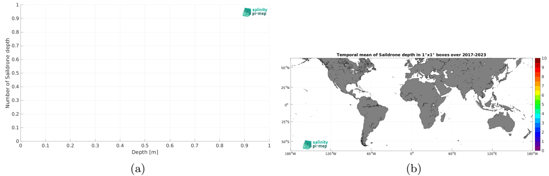
Figure 4: Histograms of the depth of the upper level SSS measurements from Sairdrone in the Match-up DataBase for the SMOS coastal zone (<800km) 60N-60S Pi-MEP region (a) and temporal mean spatial distribution of pressure of the in situ SSS data over 1^\circ \times 1^\circ boxes and for the full satellite product period (b).
