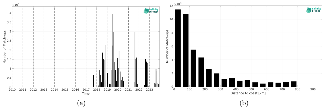
Figure 2: Number of match-ups between Saildrone and SMOS SSS L3 v9 - 9 Days (CATDS-CEC-LOCEAN) SSS as a function of time (a) and as function of the distance to coast (b) over the SMOS coastal zone (<800km) 60N-60S Pi-MEP region and for the full satellite product period.
