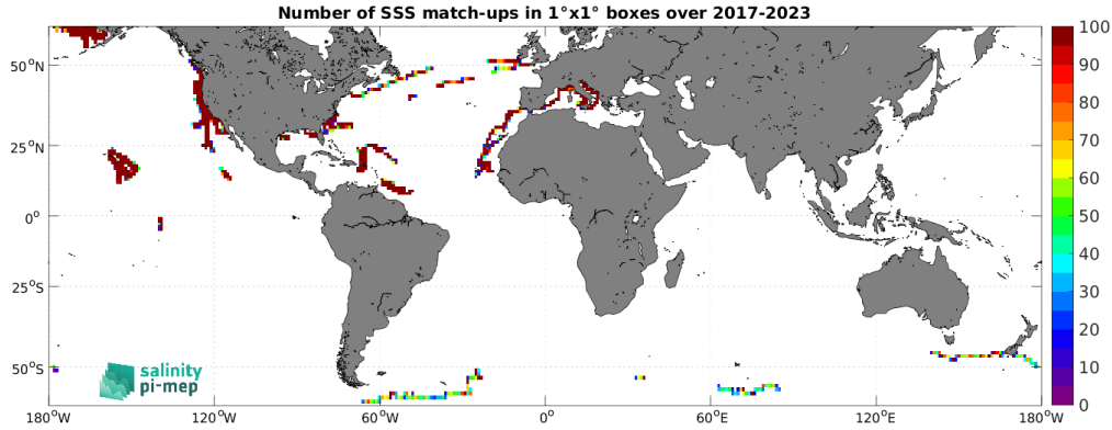
Figure 5: Number of SSS match-ups between Sairdrone SSS and the SMOS SSS L3 v9 - 9 Days (CATDS-CEC-LOCEAN) SSS product for the SMOS coastal zone (<800km) 60N-60S Pi-MEP region over 1^{\circ} \times 1^{\circ} boxes and for the full satellite product period.
