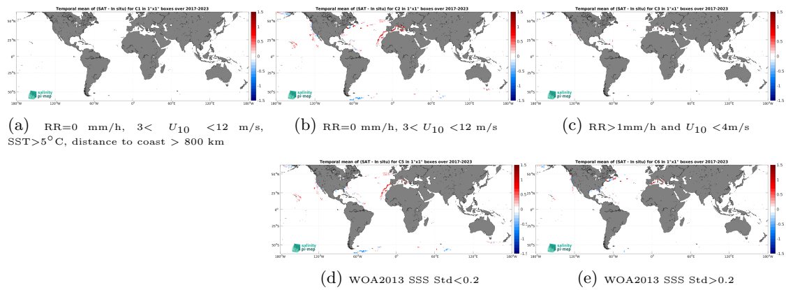
Figure 14: Temporal mean gridded over spatial boxes of size 1^\circ \times 1^\circ of \Delta\text{SSS} (SMOS SSS L3 v9 - 9 Days (CATDS-CEC-LOCEAN) - Saildrone) for 5 different subdatasets corresponding to:RR=0 mm/h, 3 < U_{10} < 12 m/s, SST>5°C, distance to coast > 800 km (a), RR=0 mm/h, 3 < U_{10} < 12 m/s (b), RR>1mm/h and U_{10} < 4 m/s (c), WOA2013 SSS Std<0.2 (d), WOA2013 SSS Std>0.2 (e).
