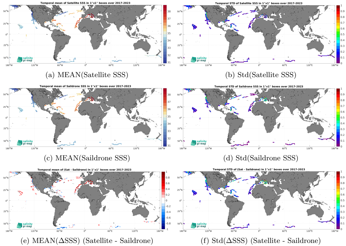
Figure 7: Temporal mean (left) and Std (right) of SSS from SMOS SSS L3 v9 - 9 Days (CATDS-CEC-LOCEAN) (top), Saildrone (middle), and of \Delta SSS (Satellite - Saildrone). Only match-up pairs are used to generate these maps.
