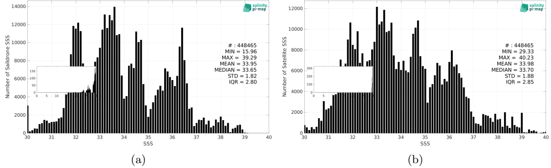
Figure 3: Histograms of SSS from Sairdrone (a) and SMOS SSS L3 v9 - 9 Days (CATDS-CEC-LOCEAN) (b) considering all match-up pairs per bins of 0.1 over the SMOS coastal zone (<800km) 60N-60S Pi-MEP region and for the full satellite product period.
