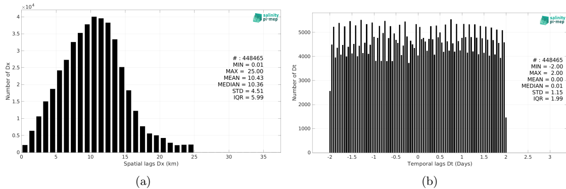
Figure 6: Histograms of the spatial (a) and temporal (b) lags between the location/time of the Sairdrone measurement and the date of the corresponding SMOS SSS L3 v9 - 9 Days (CATDS-CEC-LOCEAN) SSS pixel.
