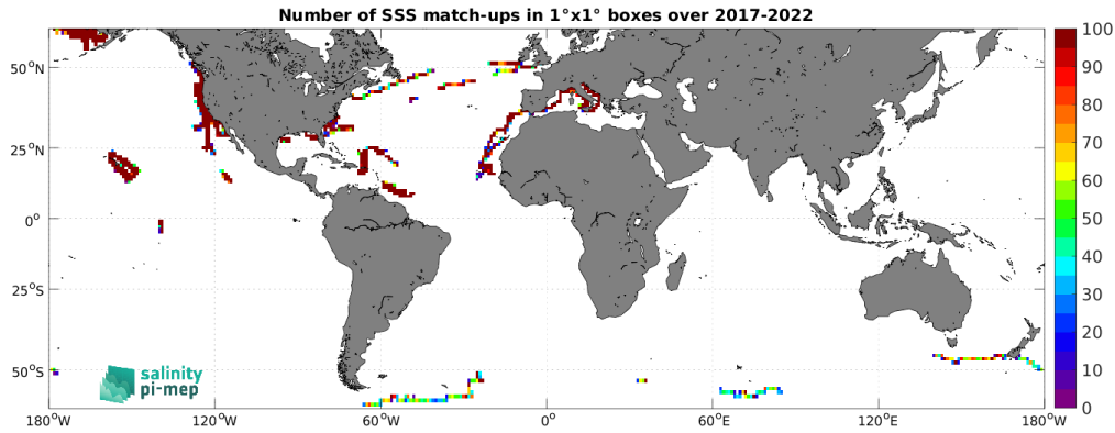
Figure 4: Number of SSS match-ups between Sairdrone SSS and the SMOS SSS L3 v9 - 9 Days (CATDS-CEC-LOCEAN) SSS product for the SMOS coastal zone (<800km) 60N-60S Pi-MEP region over 1^{\circ} \times 1^{\circ} boxes and for the full satellite product period.
