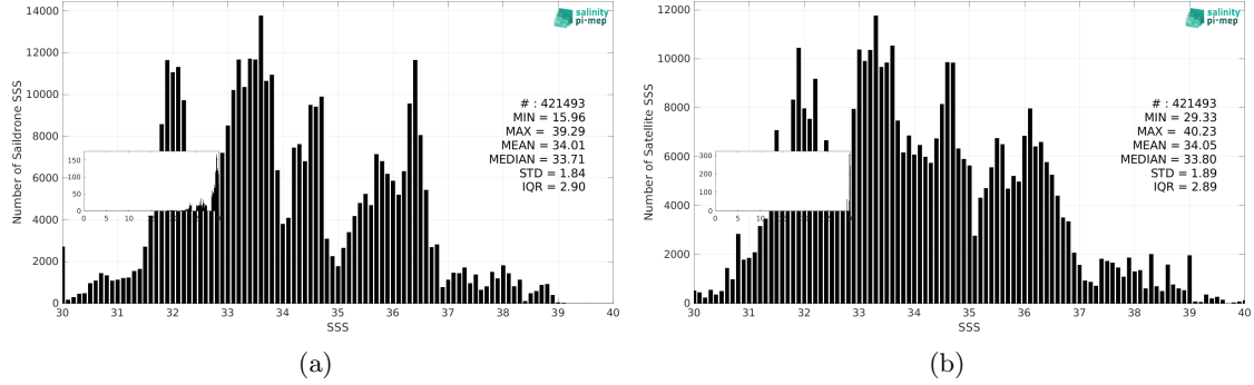
Figure 2: Histograms of SSS from Sairdrone (a) and SMOS SSS L3 v9 - 9 Days (CATDS-CEC-LOCEAN) (b) considering all match-up pairs per bins of 0.1 over the SMOS coastal zone (<800km) 60N-60S Pi-MEP region and for the full satellite product period.
