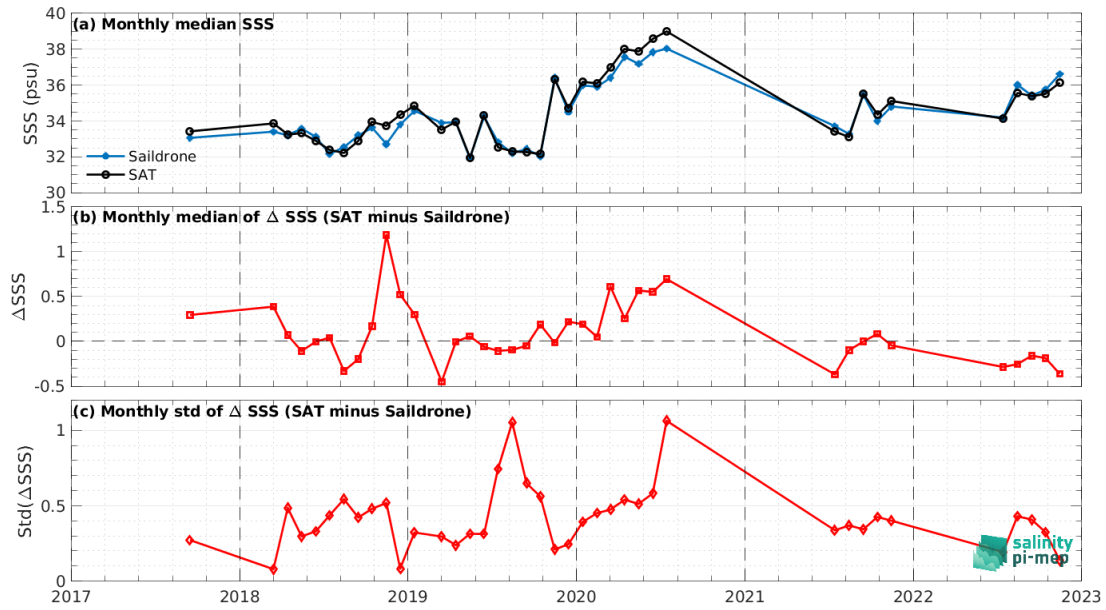
Figure 7: Time series of the monthly median SSS (top), median of \Delta SSS (Satellite - Sairdron) and Std of \Delta SSS (Satellite - Sairdron) over the SMOS coastal zone ( <800\text{km} ) 60\text{N} - 60\text{S} Pi-MEP region considering all match-ups collected by the Pi-MEP.
