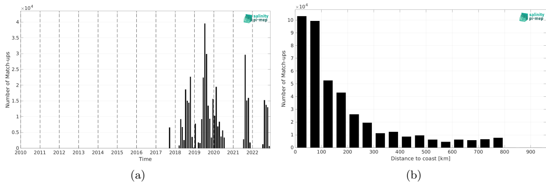
Figure 1: Number of match-ups between Saildrone and SMOS SSS L3 v9 - 9 Days (CATDS-CEC-LOCEAN) SSS as a function of time (a) and as function of the distance to coast (b) over the SMOS coastal zone (<800km) 60N-60S Pi-MEP region and for the full satellite product period.
