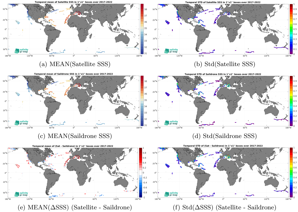
Figure 6: Temporal mean (left) and Std (right) of SSS from SMOS SSS L3 v9 - 9 Days (CATDS-CEC-LOCEAN) (top), Saildrone (middle), and of \Delta SSS (Satellite - Saildrone). Only match-up pairs are used to generate these maps.
