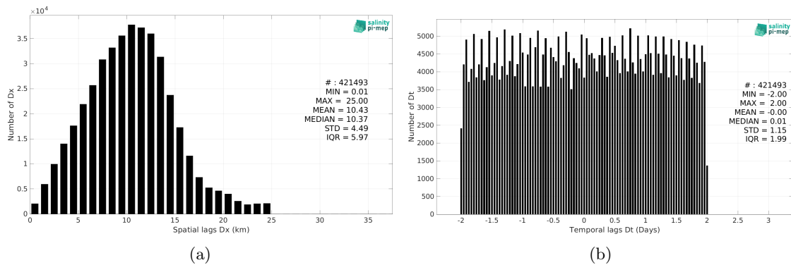
Figure 5: Histograms of the spatial (a) and temporal (b) lags between the location/time of the Sairdrone measurement and the date of the corresponding SMOS SSS L3 v9 - 9 Days (CATDS-CEC-LOCEAN) SSS pixel.
