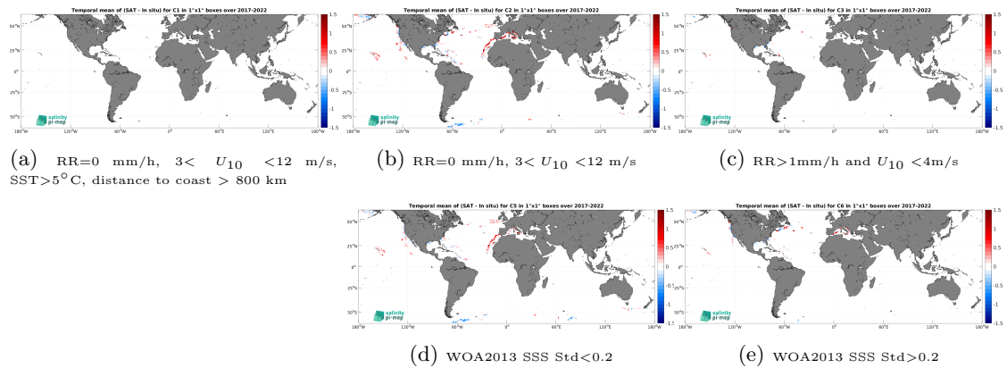
Figure 12: Temporal mean gridded over spatial boxes of size 1^\circ \times 1^\circ of \Delta SSS (SMOS SSS L3 v9 - 9 Days (CATDS-CEC-LOCEAN) - Saildrone) for 5 different subdatasets corresponding to:RR=0 mm/h, 3 < U_{10} < 12 m/s, SST >5^\circ\text{C} , distance to coast > 800 km (a), RR=0 mm/h, 3 < U_{10} < 12 m/s (b), RR >1 mm/h and U_{10} < 4 m/s (c), WOA2013 SSS Std <0.2 (d), WOA2013 SSS Std >0.2 (e).
