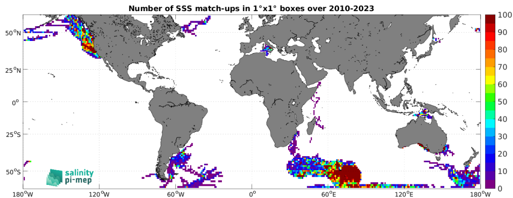
Figure 5: Number of SSS match-ups between Marine mammals SSS and the SMOS SSS L3 v9 - 9 Days (CATDS-CEC-LOCEAN) SSS product for the SMOS coastal zone (<800km) 60N-60S Pi-MEP region over 1^\circ \times 1^\circ boxes and for the full satellite product period.
