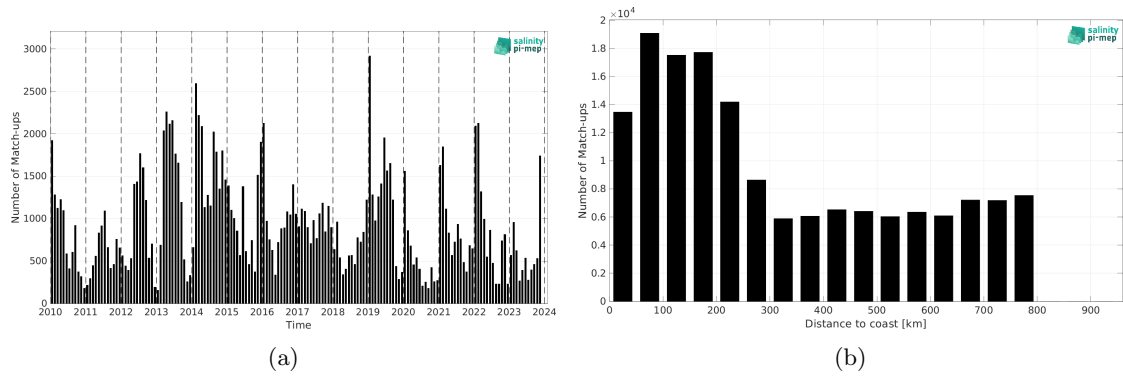
Figure 2: Number of match-ups between Marine mammals and SMOS SSS L3 v9 - 9 Days (CATDS-CEC-LOCEAN) SSS as a function of time (a) and as function of the distance to coast (b) over the SMOS coastal zone (<800km) 60N-60S Pi-MEP region and for the full satellite product period.
