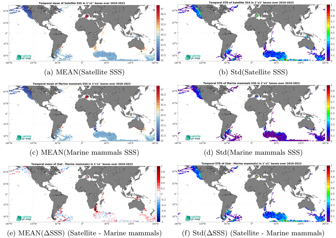
Figure 7: Temporal mean (left) and Std (right) of SSS from SMOS SSS L3 v9 - 9 Days (CATDS-CEC-LOCEAN) (top), Marine mammals (middle), and of \Delta SSS (Satellite - Marine mammals). Only match-up pairs are used to generate these maps.
