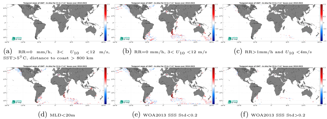
Figure 14: Temporal mean gridded over spatial boxes of size 1^\circ \times 1^\circ of \Delta\text{SSS} (SMOS SSS L3 v9 - 9 Days (CATDS-CEC-LOCEAN) - Marine mammals) for 6 different subdatasets corresponding to:RR=0 mm/h, 3 < U_{10} < 12 m/s, SST>5°C, distance to coast > 800 km (a), RR=0 mm/h, 3 < U_{10} < 12 m/s (b), RR>1mm/h and U_{10} < 4 m/s (c),MLD<20m (d),WOA2013 SSS Std<0.2 (e),WOA2013 SSS Std>0.2 (f).
