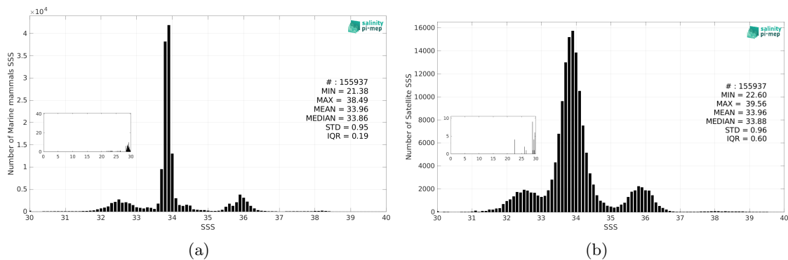
Figure 3: Histograms of SSS from Marine mammals (a) and SMOS SSS L3 v9 - 9 Days (CATDS-CEC-LOCEAN) (b) considering all match-up pairs per bins of 0.1 over the SMOS coastal zone (<800km) 60N-60S Pi-MEP region and for the full satellite product period.
