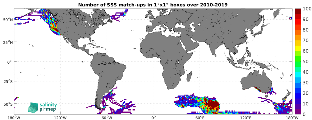
Figure 4: Number of SSS match-ups between Marine mammals SSS and the SMOS SSS L3 v9 - 9 Days (CATDS-CEC-LOCEAN) SSS product for the SMOS coastal zone (<800km) 60N-60S Pi-MEP region over 1^\circ \times 1^\circ boxes and for the full satellite product period.
