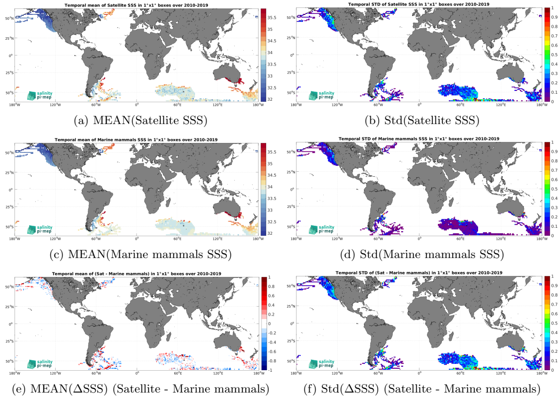
Figure 6: Temporal mean (left) and Std (right) of SSS from SMOS SSS L3 v9 - 9 Days (CATDS-CEC-LOCEAN) (top), Marine mammals (middle), and of \Delta SSS (Satellite - Marine mammals). Only match-up pairs are used to generate these maps.
