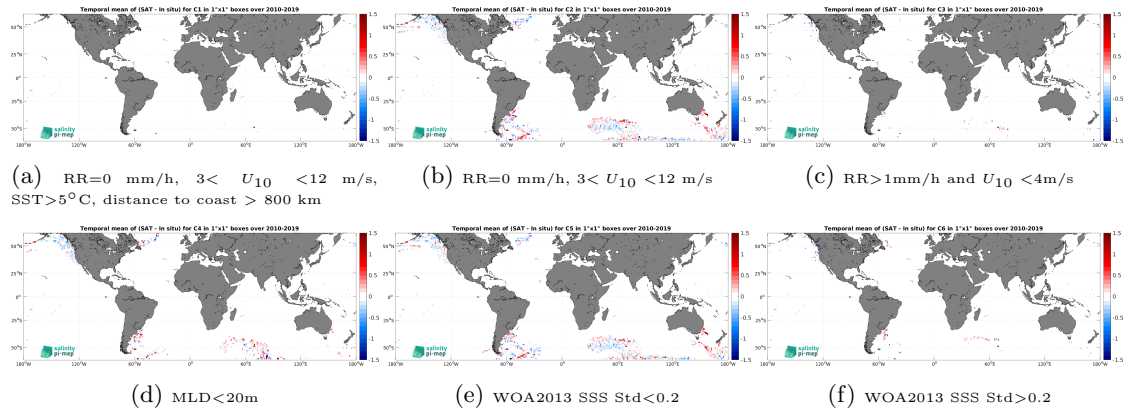
Figure 12: Temporal mean gridded over spatial boxes of size 1^{\circ}\times 1^{\circ} of \Delta\text{SSS} (SMOS SSS L3 v9 - 9 Days (CATDS-CEC-LOCEAN) - Marine mammals) for 6 different subdatasets corresponding to:RR=0 mm/h, 3 < U_{10} < 12 m/s, SST > 5^{\circ}\text{C} , distance to coast > 800 km (a), RR=0 mm/h, 3 < U_{10} < 12 m/s (b), RR > 1\text{mm/h} and U_{10} < 4\text{m/s} (c),MLD < 20\text{m} (d),WOA2013 SSS Std < 0.2 (e),WOA2013 SSS Std > 0.2 (f).
