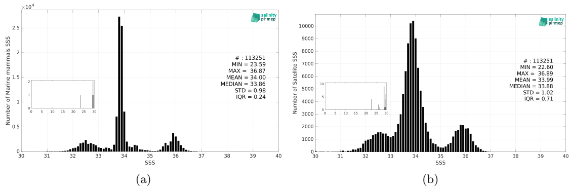
Figure 2: Histograms of SSS from Marine mammals (a) and SMOS SSS L3 v9 - 9 Days (CATDS-CEC-LOCEAN) (b) considering all match-up pairs per bins of 0.1 over the SMOS coastal zone (<800km) 60N-60S Pi-MEP region and for the full satellite product period.
