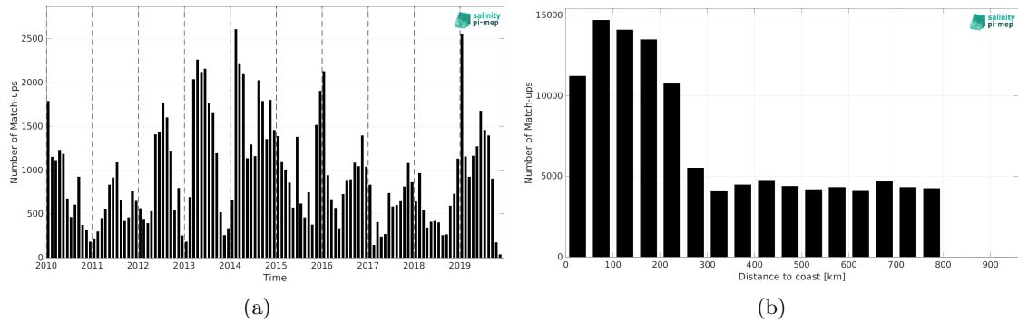
Figure 1: Number of match-ups between Marine mammals and SMOS SSS L3 v9 - 9 Days (CATDS-CEC-LOCEAN) SSS as a function of time (a) and as function of the distance to coast (b) over the SMOS coastal zone (<800km) 60N-60S Pi-MEP region and for the full satellite product period.
