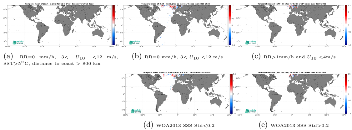
Figure 14: Temporal mean gridded over spatial boxes of size 1^\circ \times 1^\circ of \Delta SSS (SMOS SSS L3 v9 - 9 Days (CATDS-CEC-LOCEAN) - ICES) for 5 different subdatasets corresponding to:RR=0 mm/h, 3 < U_{10} < 12 m/s, SST >5^\circ C, distance to coast > 800 km (a), RR=0 mm/h, 3 < U_{10} < 12 m/s (b), RR >1 mm/h and U_{10} < 4 m/s (c), WOA2013 SSS Std <0.2 (d), WOA2013 SSS Std >0.2 (e).
