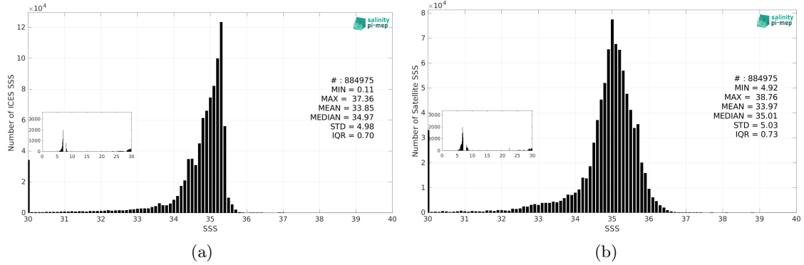
Figure 3: Histograms of SSS from ICES (a) and SMOS SSS L3 v9 - 9 Days (CATDS-CEC-LOCEAN) (b) considering all match-up pairs per bins of 0.1 over the SMOS coastal zone (<800km) 60N-60S Pi-MEP region and for the full satellite product period.
