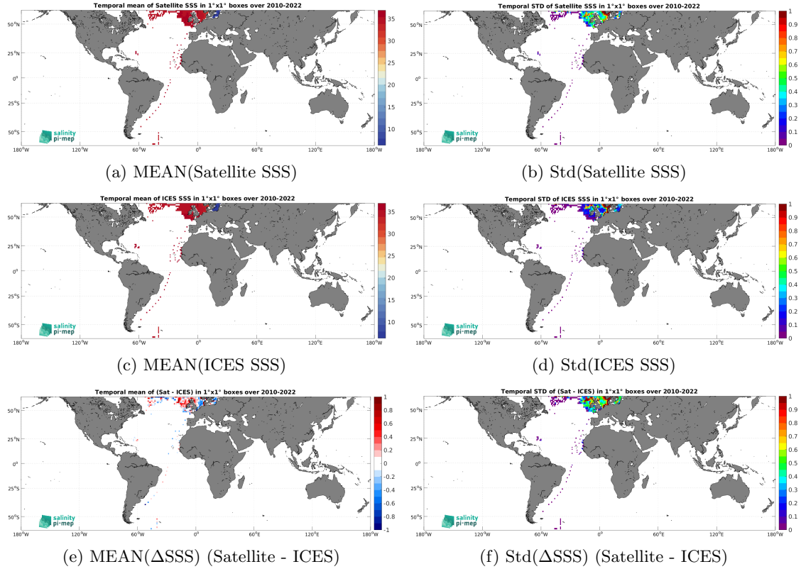
Figure 7: Temporal mean (left) and Std (right) of SSS from SMOS SSS L3 v9 - 9 Days (CATDS-CEC-LOCEAN) (top), ICES (middle), and of \Delta SSS (Satellite - ICES). Only match-up pairs are used to generate these maps.
