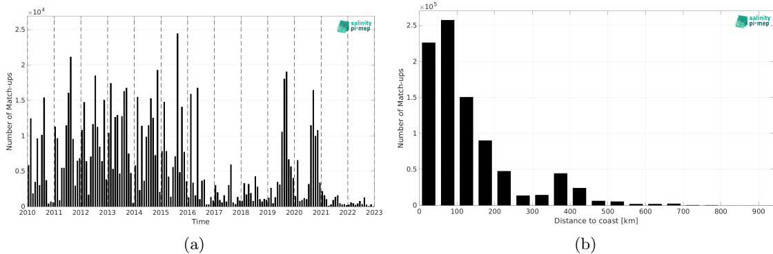
Figure 2: Number of match-ups between ICES and SMOS SSS L3 v9 - 9 Days (CATDS-CEC-LOCEAN) SSS as a function of time (a) and as function of the distance to coast (b) over the SMOS coastal zone (<800km) 60N-60S Pi-MEP region and for the full satellite product period.
