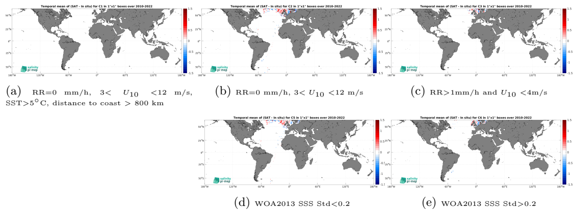
Figure 14: Temporal mean gridded over spatial boxes of size 1^\circ \times 1^\circ of \Delta\text{SSS} (SMOS SSS L3 v9 - 9 Days (CATDS-CEC-LOCEAN) - ICES) for 5 different subdatasets corresponding to:RR=0 mm/h, 3 < U_{10} < 12 m/s, SST > 5^\circ\text{C} , distance to coast > 800 km (a), RR=0 mm/h, 3 < U_{10} < 12 m/s (b), RR > 1 mm/h and U_{10} < 4 m/s (c), WOA2013 SSS Std < 0.2 (d), WOA2013 SSS Std > 0.2 (e).
