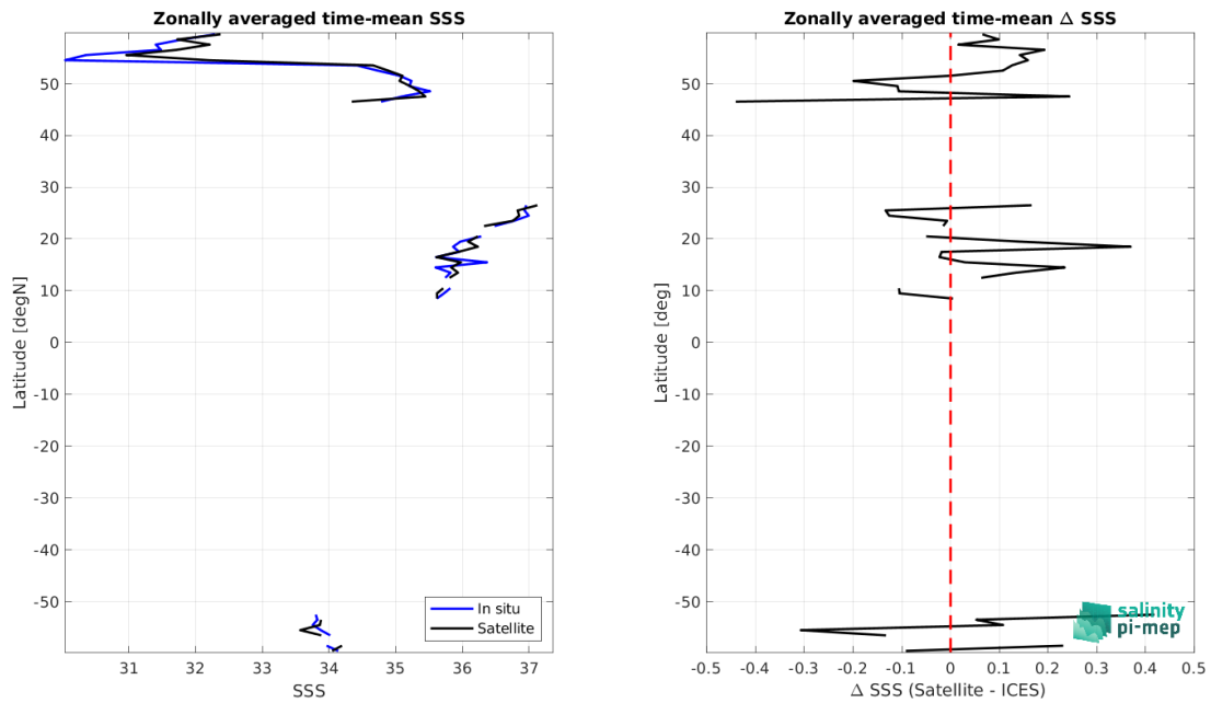
Figure 8: Left panel: Zonal mean SSS from SMOS SSS L3 v9 - 9 Days (CATDS-CEC-LOCEAN) satellite product (black) and from ICES (blue). Right panel: Zonal mean of \Delta SSS (Satellite - ICES) for all the collected Pi-MEP match-up pairs estimated over the full satellite product period.
