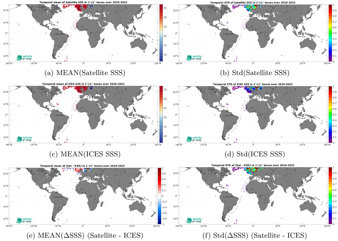
Figure 6: Temporal mean (left) and Std (right) of SSS from SMOS SSS L3 v9 - 9 Days (CATDS-CEC-LOCEAN) (top), ICES (middle), and of \Delta\text{SSS} (Satellite - ICES). Only match-up pairs are used to generate these maps.
