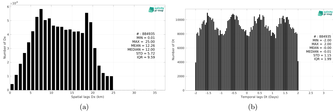
Figure 5: Histograms of the spatial (a) and temporal (b) lags between the location/time of the ICES measurement and the date of the corresponding SMOS SSS L3 v9 - 9 Days (CATDS-CEC-LOCEAN) SSS pixel.
