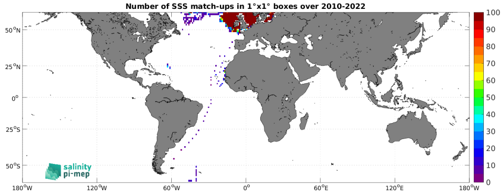
Figure 4: Number of SSS match-ups between ICES SSS and the SMOS SSS L3 v9 - 9 Days (CATDS-CEC-LOCEAN) SSS product for the SMOS coastal zone ( <800\text{km} ) 60N-60S Pi-MEP region over 1^\circ \times 1^\circ boxes and for the full satellite product period.
