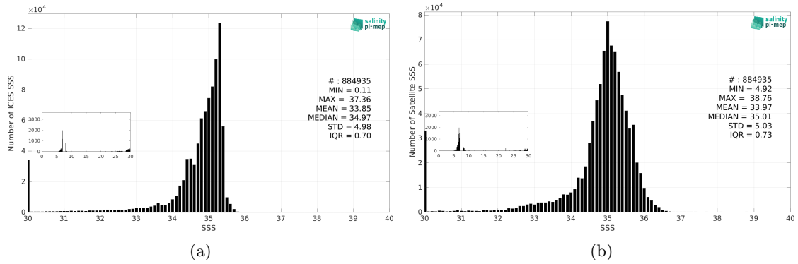
Figure 2: Histograms of SSS from ICES (a) and SMOS SSS L3 v9 - 9 Days (CATDS-CEC-LOCEAN) (b) considering all match-up pairs per bins of 0.1 over the SMOS coastal zone (<800km) 60N-60S Pi-MEP region and for the full satellite product period.
