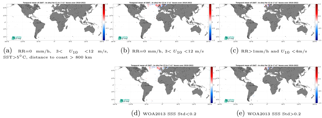
Figure 12: Temporal mean gridded over spatial boxes of size 1^\circ \times 1^\circ of \Delta SSS (SMOS SSS L3 v9 - 9 Days (CATDS-CEC-LOCEAN) - ICES) for 5 different subdatasets corresponding to:RR=0 mm/h, 3 < U_{10} < 12 m/s, SST >5^\circ C, distance to coast > 800 km (a), RR=0 mm/h, 3 < U_{10} < 12 m/s (b), RR >1 mm/h and U_{10} < 4 m/s (c), WOA2013 SSS Std <0.2 (d), WOA2013 SSS Std >0.2 (e).
