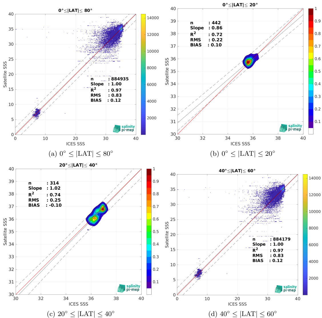
Figure 9: Contour maps of the concentration of SMOS SSS L3 v9 - 9 Days (CATDS-CEC-LOCEAN) SSS (y-axis) versus ICES SSS (x-axis) at match-up pairs for different latitude bands. For each plot, the red line shows x=y . The black thin and dashed lines indicate a linear fit through the data cloud and the \pm 95\% confidence levels, respectively. The number match-up pairs n , the slope and R^2 coefficient of the linear fit, the root mean square (RMS) and the mean bias between satellite and in situ data are indicated for each latitude band in each plots.
