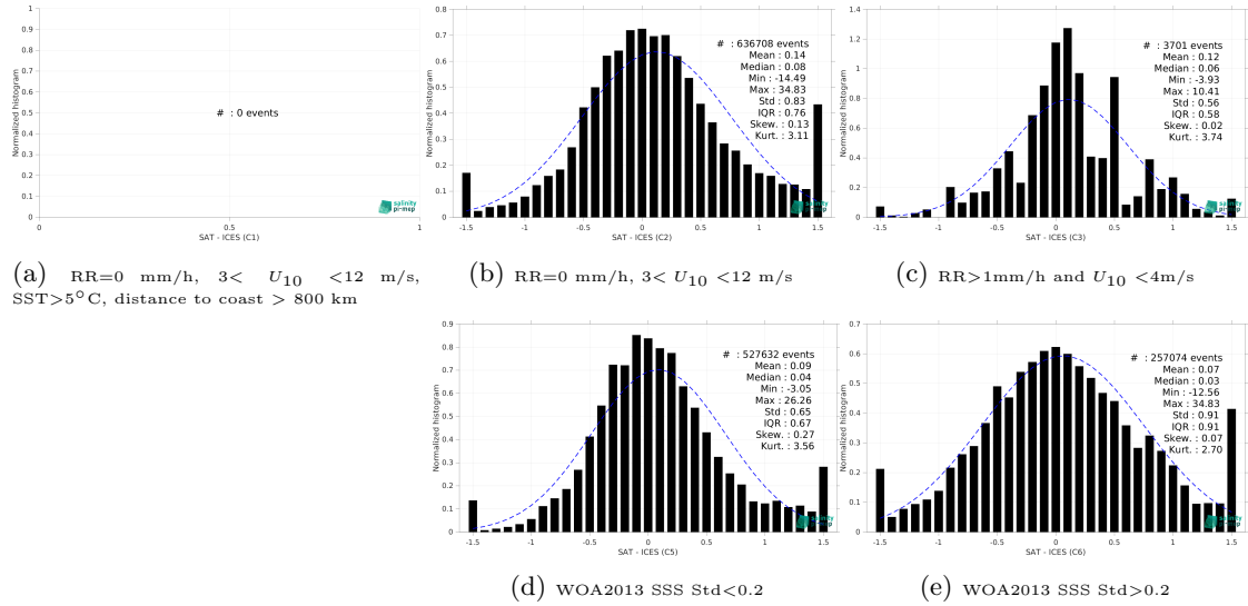
Figure 13: Normalized histogram of \Delta SSS (SMOS SSS L3 v9 - 9 Days (CATDS-CEC-LOCEAN) - ICES) for 5 different subdatasets corresponding to: RR=0 mm/h, 3 < U_{10} < 12 m/s, SST > 5°C, distance to coast > 800 km (a), RR=0 mm/h, 3 < U_{10} < 12 m/s (b), RR > 1mm/h and U_{10} < 4 m/s (c), WOA2013 SSS Std < 0.2 (d), WOA2013 SSS Std > 0.2 (e).
