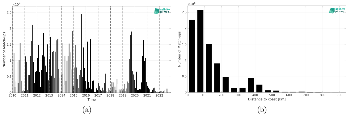
Figure 1: Number of match-ups between ICES and SMOS SSS L3 v9 - 9 Days (CATDS-CEC-LOCEAN) SSS as a function of time (a) and as function of the distance to coast (b) over the SMOS coastal zone (<800km) 60N-60S Pi-MEP region and for the full satellite product period.
