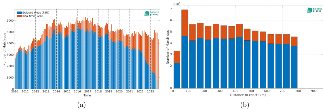
Figure 1: Number of match-ups between Argo and SMOS SSS L3 v9 - 9 Days (CATDS-CEC-LOCEAN) SSS as a function of time (a) and as function of the distance to coast (b) over the SMOS coastal zone (<800km) 60N-60S Pi-MEP region and for the full satellite product period.
