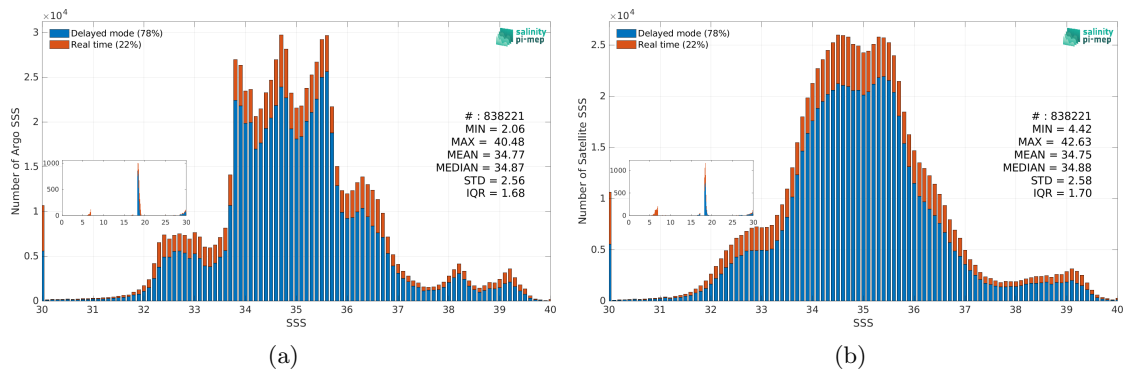
Figure 2: Histograms of SSS from Argo (a) and SMOS SSS L3 v9 - 9 Days (CATDS-CEC-LOCEAN) (b) considering all match-up pairs per bins of 0.1 over the SMOS coastal zone (<800km) 60N-60S Pi-MEP region and for the full satellite product period.
