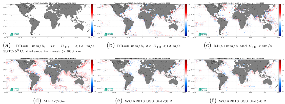
Figure 12: Temporal mean gridded over spatial boxes of size 1^\circ \times 1^\circ of \Delta SSS (SMOS SSS L3 v9 - 9 Days (CATDS-CEC-LOCEAN) - Argo) for 6 different subdatasets corresponding to:RR=0 mm/h, 3 < U_{10} < 12 m/s, SST > 5^\circ C, distance to coast > 800 km (a), RR=0 mm/h, 3 < U_{10} < 12 m/s (b), RR > 1 mm/h and U_{10} < 4 m/s (c),MLD < 20 m (d),WOA2013 SSS Std < 0.2 (e),WOA2013 SSS Std > 0.2 (f).
