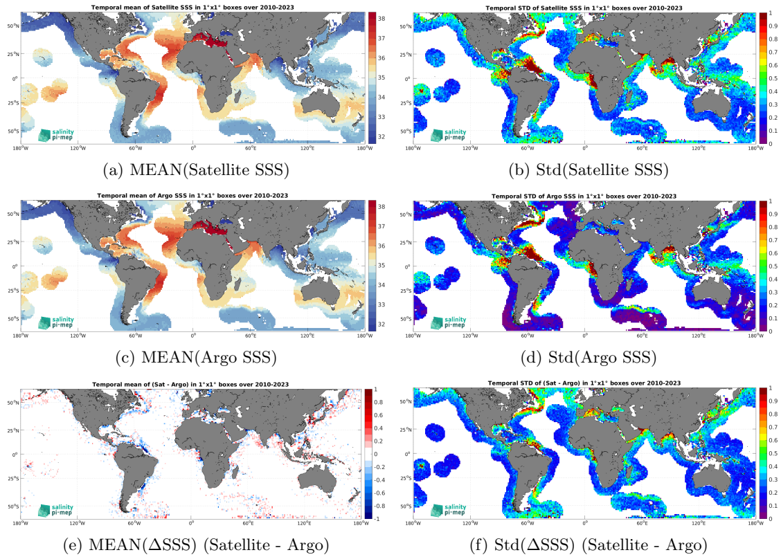
Figure 6: Temporal mean (left) and Std (right) of SSS from SMOS SSS L3 v9 - 9 Days (CATDS-CEC-LOCEAN) (top), Argo (middle), and of \Delta SSS (Satellite - Argo). Only match-up pairs are used to generate these maps.
