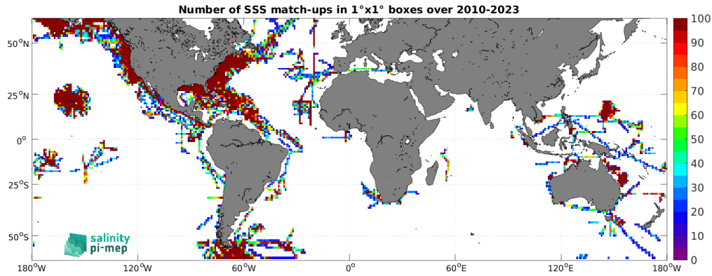
Figure 5: Number of SSS match-ups between TSG (SAMOS) SSS and the SMOS SSS L3 v9 - 18 Days (CATDS-CEC-LOCEAN) SSS product for the SMOS coastal zone (<800km) 60N-60S Pi-MEP region over 1^\circ \times 1^\circ boxes and for the full satellite product period.
