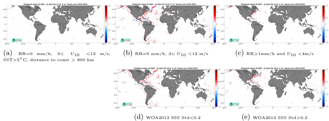
Figure 14: Temporal mean gridded over spatial boxes of size 1^\circ \times 1^\circ of \Delta SSS (SMOS SSS L3 v9 - 18 Days (CATDS-CEC-LOCEAN) - TSG (SAMOS)) for 5 different subdatasets corresponding to:RR=0 mm/h, 3 < U_{10} < 12 m/s, SST >5^\circ C, distance to coast > 800 km (a), RR=0 mm/h, 3 < U_{10} < 12 m/s (b), RR >1 mm/h and U_{10} < 4 m/s (c), WOA2013 SSS Std <0.2 (d), WOA2013 SSS Std >0.2 (e).
