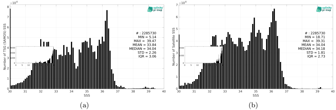
Figure 3: Histograms of SSS from TSG (SAMOS) (a) and SMOS SSS L3 v9 - 18 Days (CATDS-CEC-LOCEAN) (b) considering all match-up pairs per bins of 0.1 over the SMOS coastal zone (<800km) 60N-60S Pi-MEP region and for the full satellite product period.
