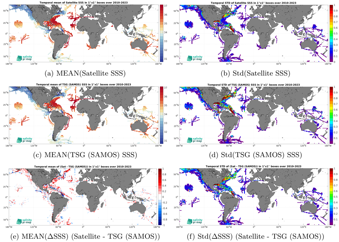
Figure 7: Temporal mean (left) and Std (right) of SSS from SMOS SSS L3 v9 - 18 Days (CATDS-CEC-LOCEAN) (top), TSG (SAMOS) (middle), and of \Delta SSS (Satellite - TSG (SAMOS)). Only match-up pairs are used to generate these maps.
