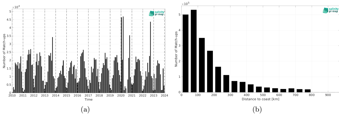
Figure 2: Number of match-ups between TSG (SAMOS) and SMOS SSS L3 v9 - 18 Days (CATDS-CEC-LOCEAN) SSS as a function of time (a) and as function of the distance to the coast (b) over the SMOS coastal zone (<800km) 60N-60S Pi-MEP region and for the full satellite product period.
