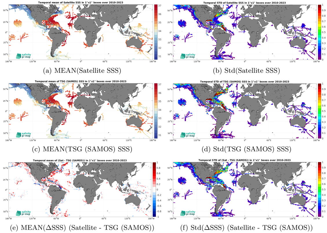
Figure 6: Temporal mean (left) and Std (right) of SSS from SMOS SSS L3 v9 - 18 Days (CATDS-CEC-LOCEAN) (top), TSG (SAMOS) (middle), and of \Delta SSS (Satellite - TSG (SAMOS)). Only match-up pairs are used to generate these maps.
