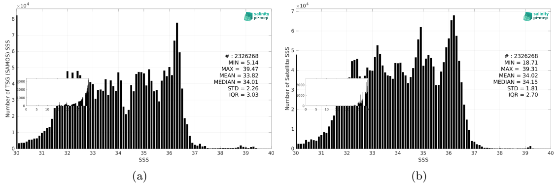
Figure 2: Histograms of SSS from TSG (SAMOS) (a) and SMOS SSS L3 v9 - 18 Days (CATDS-CEC-LOCEAN) (b) considering all match-up pairs per bins of 0.1 over the SMOS coastal zone (<800km) 60N-60S Pi-MEP region and for the full satellite product period.
