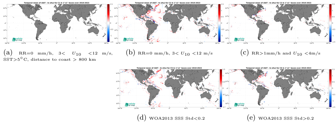
Figure 12: Temporal mean gridded over spatial boxes of size 1^\circ \times 1^\circ of \Delta\text{SSS} (SMOS SSS L3 v9 - 18 Days (CATDS-CEC-LOCEAN) - TSG (SAMOS)) for 5 different subdatasets corresponding to:RR=0 mm/h, 3 < U_{10} < 12 m/s, SST >5^\circ\text{C} , distance to coast > 800 km (a), RR=0 mm/h, 3 < U_{10} < 12 m/s (b), RR >1 mm/h and U_{10} < 4 m/s (c), WOA2013 SSS Std <0.2 (d), WOA2013 SSS Std >0.2 (e).
