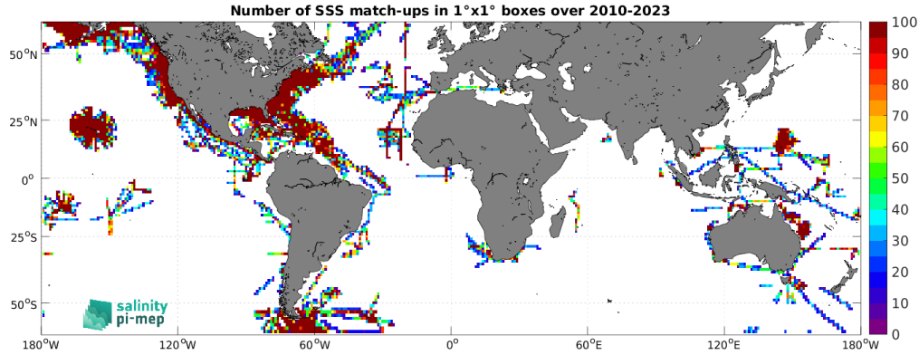
Figure 4: Number of SSS match-ups between TSG (SAMOS) SSS and the SMOS SSS L3 v9 - 18 Days (CATDS-CEC-LOCEAN) SSS product for the SMOS coastal zone (<800km) 60N-60S Pi-MEP region over 1^\circ \times 1^\circ boxes and for the full satellite product period.
