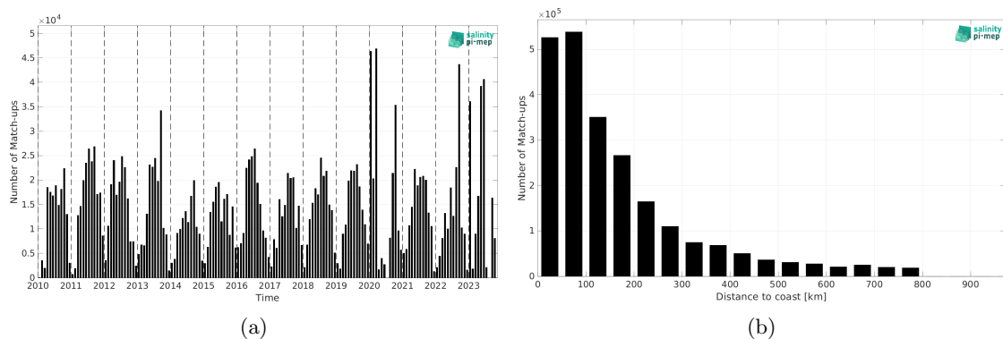
Figure 1: Number of match-ups between TSG (SAMOS) and SMOS SSS L3 v9 - 18 Days (CATDS-CEC-LOCEAN) SSS as a function of time (a) and as function of the distance to the coast (b) over the SMOS coastal zone (<800km) 60N-60S Pi-MEP region and for the full satellite product period.
