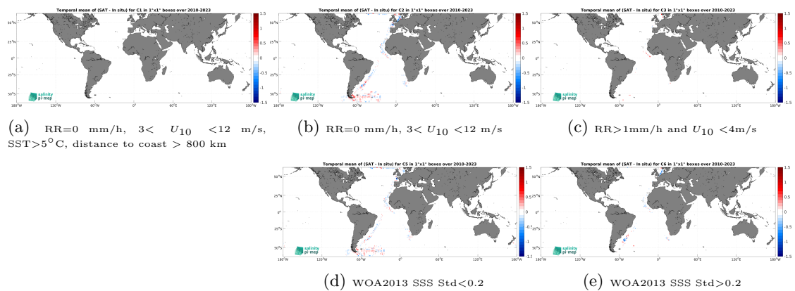
Figure 14: Temporal mean gridded over spatial boxes of size 1^\circ \times 1^\circ of \Delta\text{SSS} (SMOS SSS L3 v9 - 18 Days (CATDS-CEC-LOCEAN) - TSG (Polarstern)) for 5 different subdatasets corresponding to:RR=0 mm/h, 3 < U_{10} < 12 m/s, SST >5^\circ\text{C} , distance to coast > 800 km (a), RR=0 mm/h, 3 < U_{10} < 12 m/s (b), RR >1 mm/h and U_{10} < 4 m/s (c), WOA2013 SSS Std <0.2 (d), WOA2013 SSS Std >0.2 (e).
