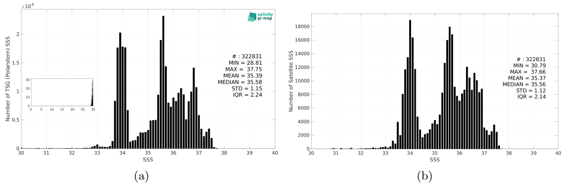
Figure 3: Histograms of SSS from TSG (Polarstern) (a) and SMOS SSS L3 v9 - 18 Days (CATDS-CEC-LOCEAN) (b) considering all match-up pairs per bins of 0.1 over the SMOS coastal zone (<800km) 60N-60S Pi-MEP region and for the full satellite product period.
