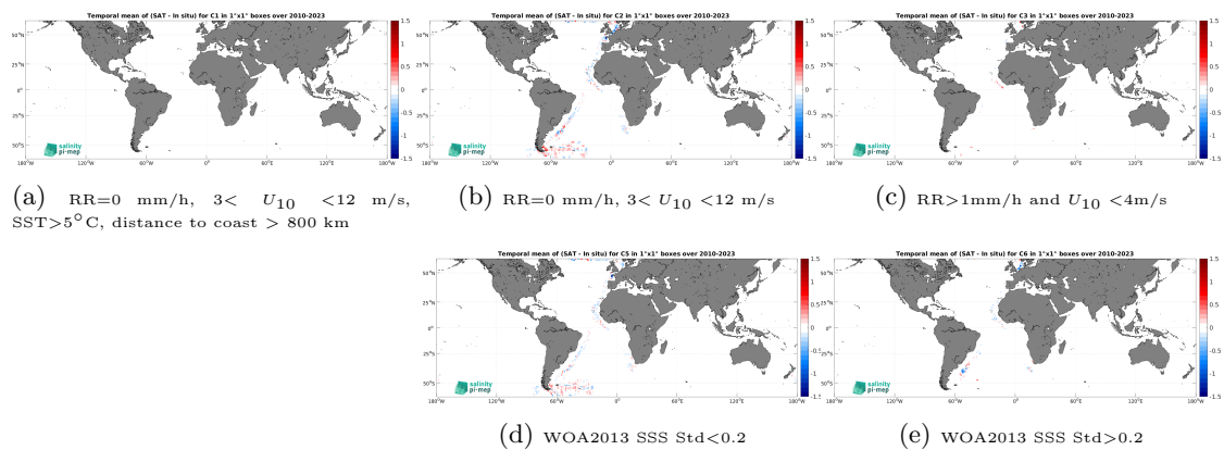
Figure 14: Temporal mean gridded over spatial boxes of size 1^\circ \times 1^\circ of \Delta SSS (SMOS SSS L3 v9 - 18 Days (CATDS-CEC-LOCEAN) - TSG (Polarstern)) for 5 different subdatasets corresponding to:RR=0 mm/h, 3 < U_{10} < 12 m/s, SST >5^\circ C, distance to coast > 800 km (a), RR=0 mm/h, 3 < U_{10} < 12 m/s (b), RR >1 mm/h and U_{10} < 4 m/s (c), WOA2013 SSS Std <0.2 (d), WOA2013 SSS Std >0.2 (e).
