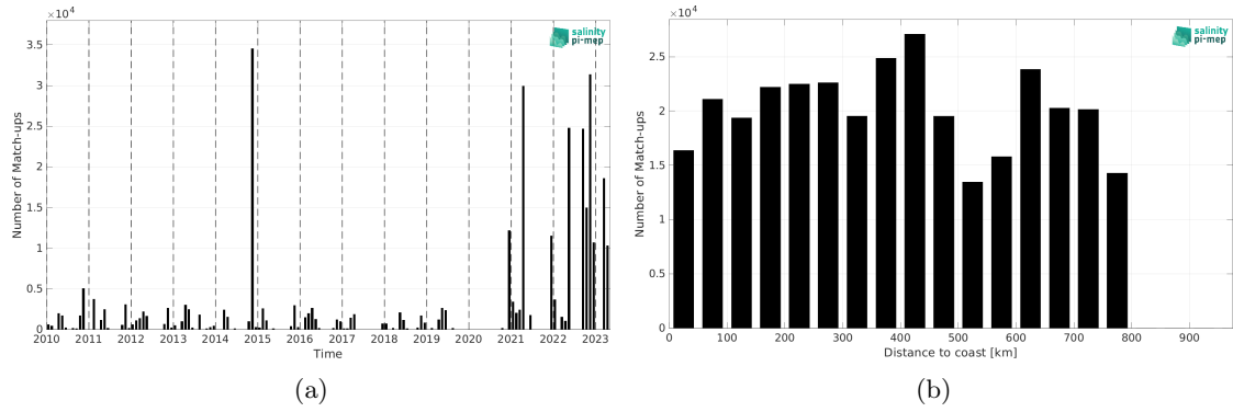
Figure 2: Number of match-ups between TSG (Polarstern) and SMOS SSS L3 v9 - 18 Days (CATDS-CEC-LOCEAN) SSS as a function of time (a) and as function of the distance to coast (b) over the SMOS coastal zone (<800km) 60N-60S Pi-MEP region and for the full satellite product period.
