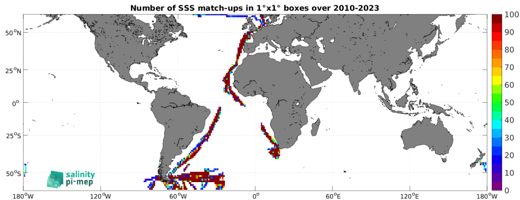
Figure 5: Number of SSS match-ups between TSG (Polarstern) SSS and the SMOS SSS L3 v9 - 18 Days (CATDS-CEC-LOCEAN) SSS product for the SMOS coastal zone (<800km) 60N-60S Pi-MEP region over 1^\circ \times 1^\circ boxes and for the full satellite product period.
