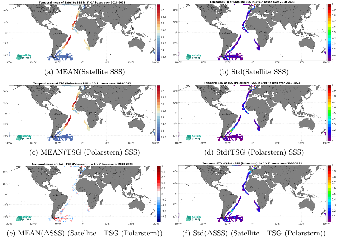
Figure 7: Temporal mean (left) and Std (right) of SSS from SMOS SSS L3 v9 - 18 Days (CATDS-CEC-LOCEAN) (top), TSG (Polarstern) (middle), and of \Delta SSS (Satellite - TSG (Polarstern)). Only match-up pairs are used to generate these maps.
