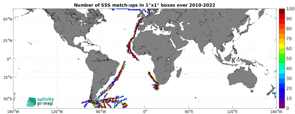
Figure 4: Number of SSS match-ups between TSG (Polarstern) SSS and the SMOS SSS L3 v9 - 18 Days (CATDS-CEC-LOCEAN) SSS product for the SMOS coastal zone (<800km) 60N-60S Pi-MEP region over 1^\circ \times 1^\circ boxes and for the full satellite product period.
