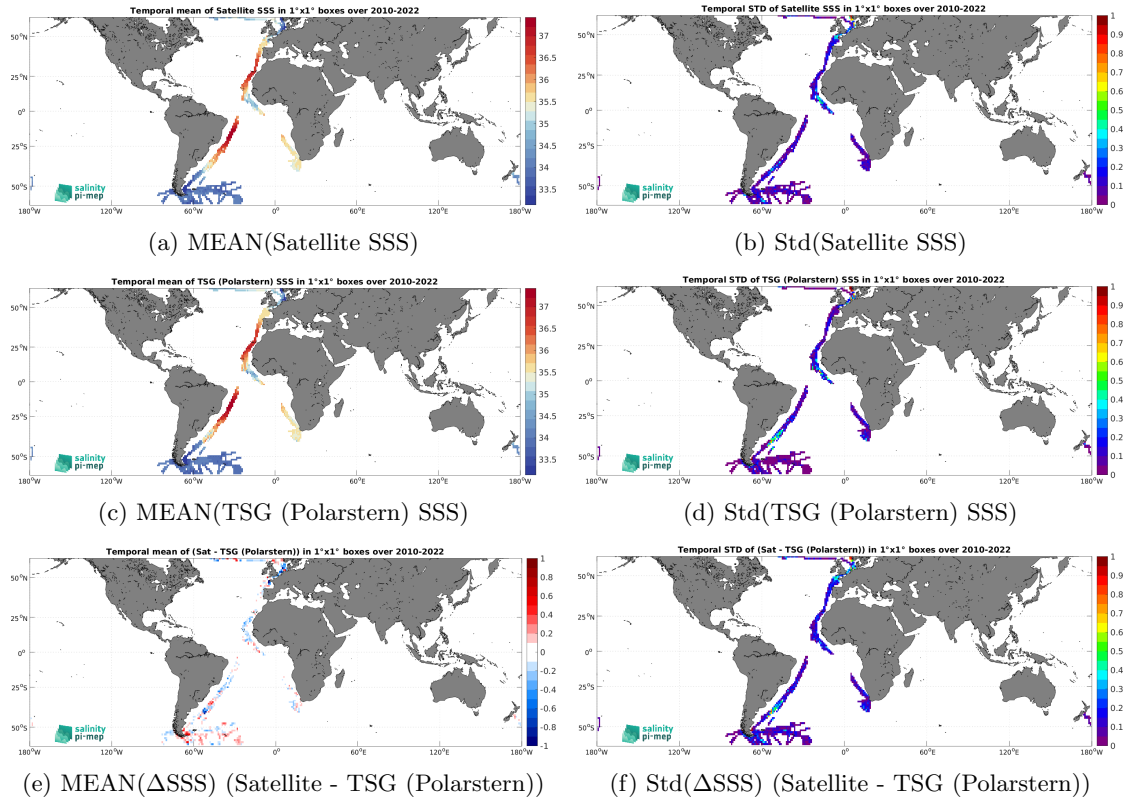
Figure 6: Temporal mean (left) and Std (right) of SSS from SMOS SSS L3 v9 - 18 Days (CATDS-CEC-LOCEAN) (top), TSG (Polarstern) (middle), and of \Delta SSS (Satellite - TSG (Polarstern)). Only match-up pairs are used to generate these maps.
