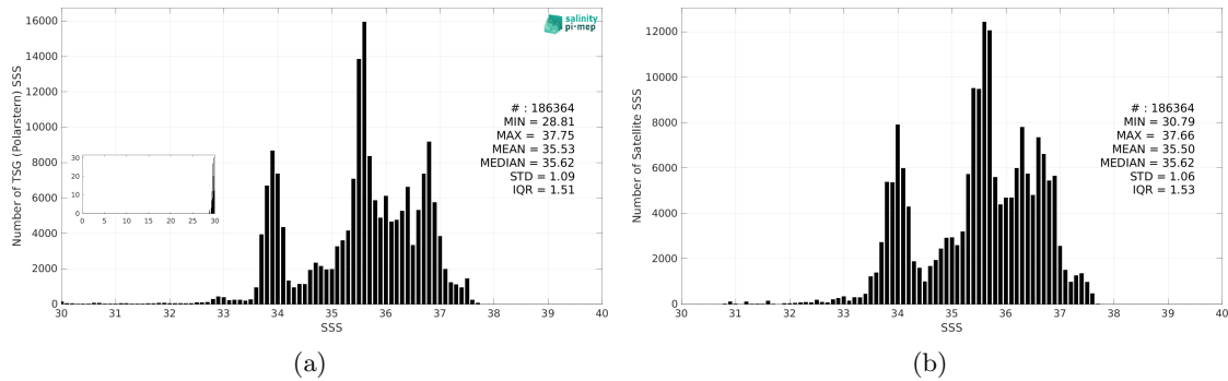
Figure 2: Histograms of SSS from TSG (Polarstern) (a) and SMOS SSS L3 v9 - 18 Days (CATDS-CEC-LOCEAN) (b) considering all match-up pairs per bins of 0.1 over the SMOS coastal zone (<800km) 60N-60S Pi-MEP region and for the full satellite product period.
