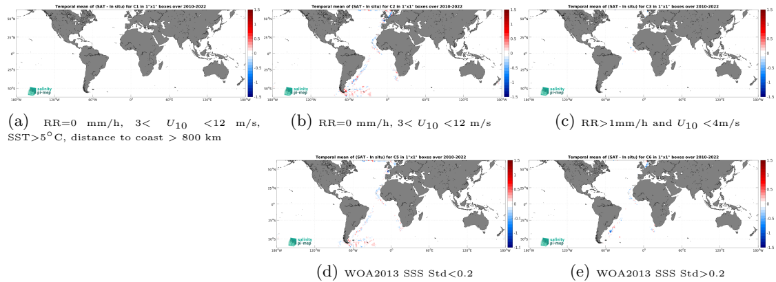
Figure 12: Temporal mean gridded over spatial boxes of size 1^\circ \times 1^\circ of \Delta SSS (SMOS SSS L3 v9 - 18 Days (CATDS-CEC-LOCEAN) - TSG (Polarstern)) for 5 different subdatasets corresponding to:RR=0 mm/h, 3 < U_{10} < 12 m/s, SST >5^\circ C, distance to coast > 800 km (a), RR=0 mm/h, 3 < U_{10} < 12 m/s (b), RR >1 mm/h and U_{10} < 4 m/s (c), WOA2013 SSS Std <0.2 (d), WOA2013 SSS Std >0.2 (e).
