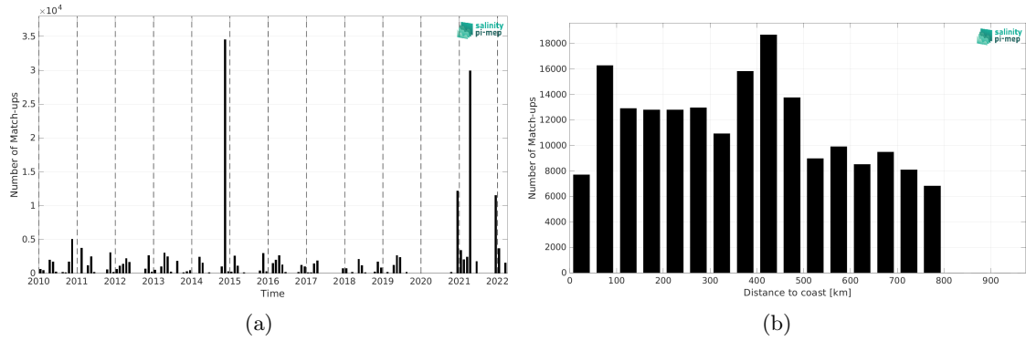
Figure 1: Number of match-ups between TSG (Polarstern) and SMOS SSS L3 v9 - 18 Days (CATDS-CEC-LOCEAN) SSS as a function of time (a) and as function of the distance to coast (b) over the SMOS coastal zone (<800km) 60N-60S Pi-MEP region and for the full satellite product period.
