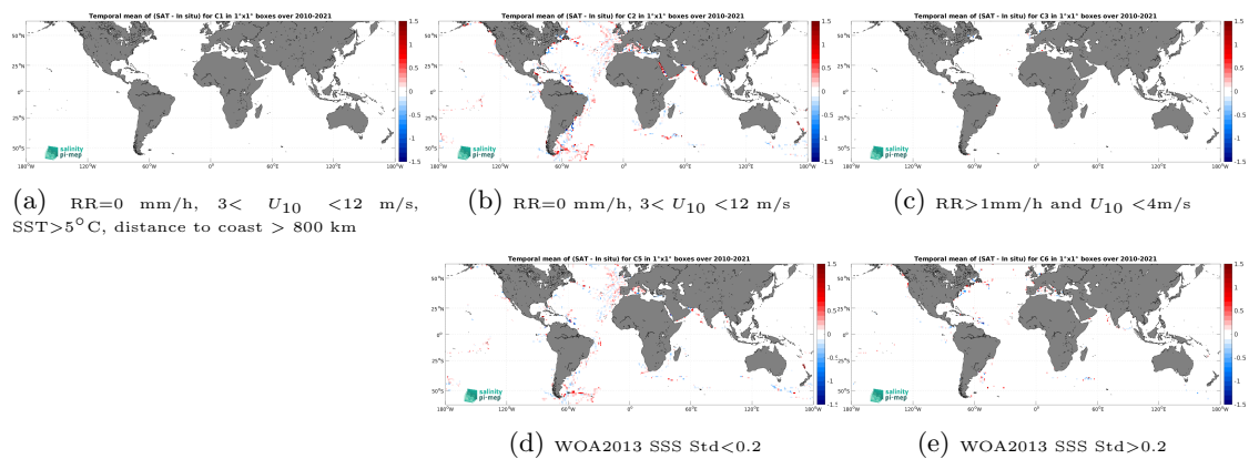
Figure 14: Temporal mean gridded over spatial boxes of size 1^\circ \times 1^\circ of \Delta\text{SSS} (SMOS SSS L3 v9 - 18 Days (CATDS-CEC-LOCEAN) - TSG (GOSUD-Sailing-ship)) for 5 different subdatasets corresponding to: RR=0 mm/h, 3 < U_{10} < 12 m/s, SST > 5°C, distance to coast > 800 km (a), RR=0 mm/h, 3 < U_{10} < 12 m/s (b), RR > 1mm/h and U_{10} < 4 m/s (c), WOA2013 SSS Std < 0.2 (d), WOA2013 SSS Std > 0.2 (e).
