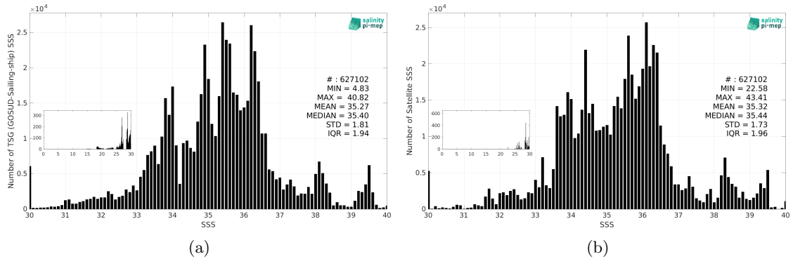
Figure 3: Histograms of SSS from TSG (GOSUD-Sailing-ship) (a) and SMOS SSS L3 v9 - 18 Days (CATDS-CEC-LOCEAN) (b) considering all match-up pairs per bins of 0.1 over the SMOS coastal zone (<800km) 60N-60S Pi-MEP region and for the full satellite product period.
