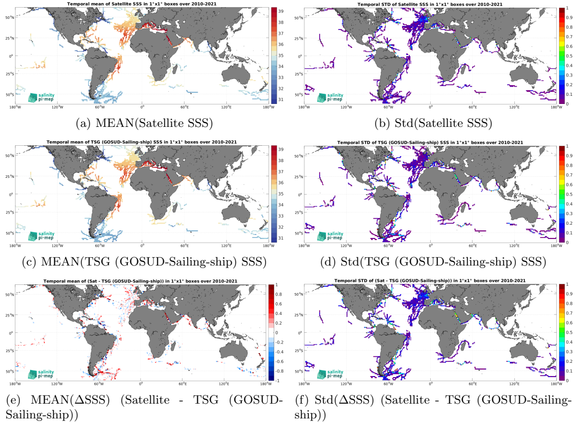
Figure 7: Temporal mean (left) and Std (right) of SSS from SMOS SSS L3 v9 - 18 Days (CATDS-CEC-LOCEAN) (top), TSG (GOSUD-Sailing-ship) (middle), and of \Delta\text{SSS} (Satellite - TSG (GOSUD-Sailing-ship)). Only match-up pairs are used to generate these maps.
