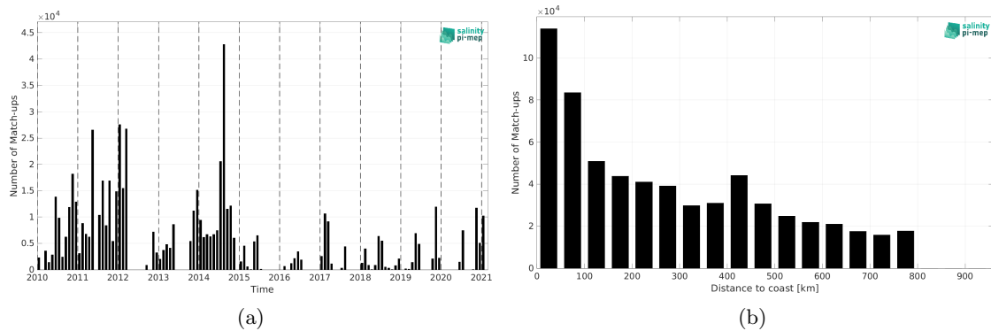
Figure 2: Number of match-ups between TSG (GOSUD-Sailing-ship) and SMOS SSS L3 v9 - 18 Days (CATDS-CEC-LOCEAN) SSS as a function of time (a) and as function of the distance to coast (b) over the SMOS coastal zone ( < 800\text{km} ) 60N-60S Pi-MEP region and for the full satellite product period.
