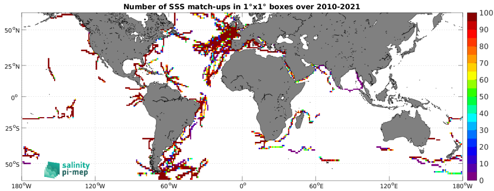
Figure 5: Number of SSS match-ups between TSG (GOSUD-Sailing-ship) SSS and the SMOS SSS L3 v9 - 18 Days (CATDS-CEC-LOCEAN) SSS product for the SMOS coastal zone ( <800\text{km} ) 60N-60S Pi-MEP region over 1^\circ \times 1^\circ boxes and for the full satellite product period.
