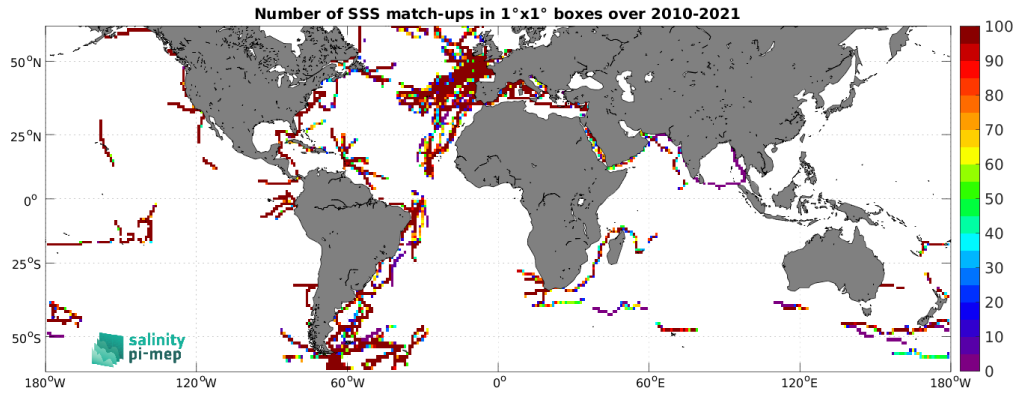
Figure 5: Number of SSS match-ups between TSG (GOSUD-Sailing-ship) SSS and the SMOS SSS L3 v9 - 18 Days (CATDS-CEC-LOCEAN) SSS product for the SMOS coastal zone (<800km) 60N-60S Pi-MEP region over 1^\circ \times 1^\circ boxes and for the full satellite product period.
