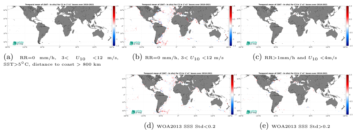
Figure 14: Temporal mean gridded over spatial boxes of size 1^\circ \times 1^\circ of \Delta SSS (SMOS SSS L3 v9 - 18 Days (CATDS-CEC-LOCEAN) - TSG (GOSUD-Sailing-ship)) for 5 different subdatasets corresponding to: RR=0 mm/h, 3 < U_{10} < 12 m/s, SST > 5^\circ\text{C} , distance to coast > 800 km (a), RR=0 mm/h, 3 < U_{10} < 12 m/s (b), RR > 1 mm/h and U_{10} < 4 m/s (c), WOA2013 SSS Std < 0.2 (d), WOA2013 SSS Std > 0.2 (e).
