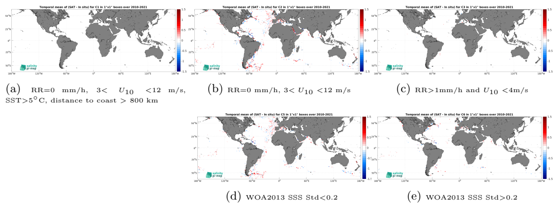
Figure 12: Temporal mean gridded over spatial boxes of size 1^\circ \times 1^\circ of \Delta\text{SSS} (SMOS SSS L3 v9 - 18 Days (CATDS-CEC-LOCEAN) - TSG (GOSUD-Sailing-ship)) for 5 different subdatasets corresponding to: RR=0 mm/h, 3 < U_{10} < 12 m/s, SST > 5°C, distance to coast > 800 km (a), RR=0 mm/h, 3 < U_{10} < 12 m/s (b), RR > 1mm/h and U_{10} < 4 m/s (c), WOA2013 SSS Std < 0.2 (d), WOA2013 SSS Std > 0.2 (e).
