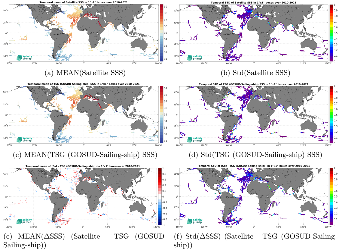
Figure 6: Temporal mean (left) and Std (right) of SSS from SMOS SSS L3 v9 - 18 Days (CATDS-CEC-LOCEAN) (top), TSG (GOSUD-Sailing-ship) (middle), and of \Delta\text{SSS} (Satellite - TSG (GOSUD-Sailing-ship)). Only match-up pairs are used to generate these maps.
