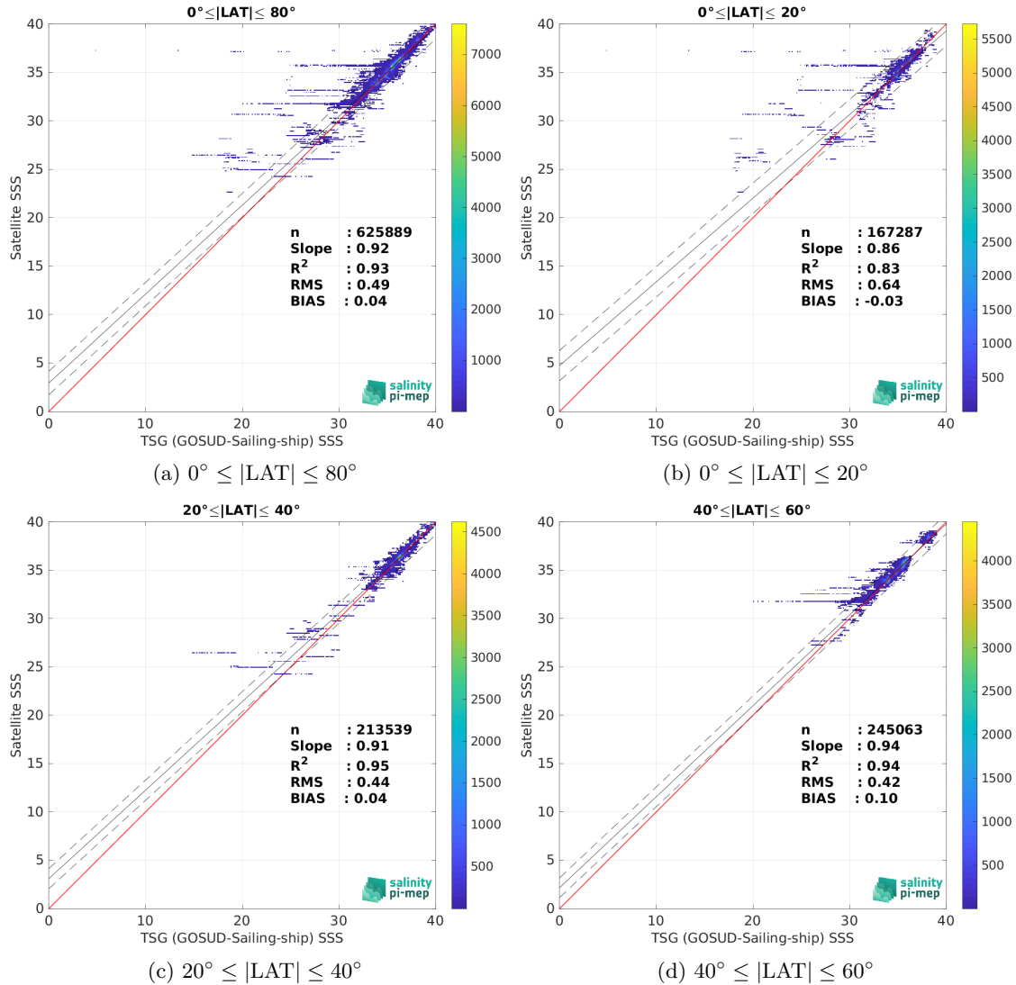
Figure 9: Contour maps of the concentration of SMOS SSS L3 v9 - 18 Days (CATDS-CEC-LOCEAN) SSS (y-axis) versus TSG (GOSUD-Sailing-ship) SSS (x-axis) at match-up pairs for different latitude bands. For each plot, the red line shows x=y . The black thin and dashed lines indicate a linear fit through the data cloud and the \pm 95\% confidence levels, respectively. The number match-up pairs n , the slope and R^2 coefficient of the linear fit, the root mean square (RMS) and the mean bias between satellite and in situ data are indicated for each latitude band in each plots.
