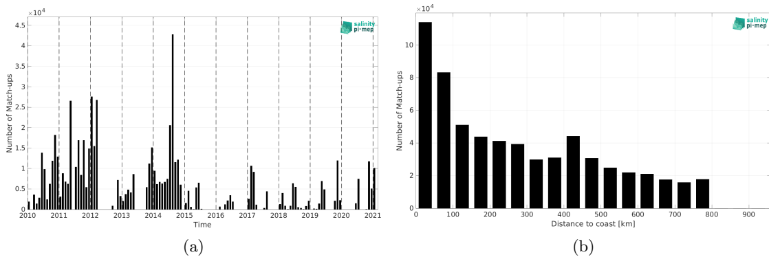
Figure 1: Number of match-ups between TSG (GOSUD-Sailing-ship) and SMOS SSS L3 v9 - 18 Days (CATDS-CEC-LOCEAN) SSS as a function of time (a) and as function of the distance to coast (b) over the SMOS coastal zone (<800km) 60N-60S Pi-MEP region and for the full satellite product period.
