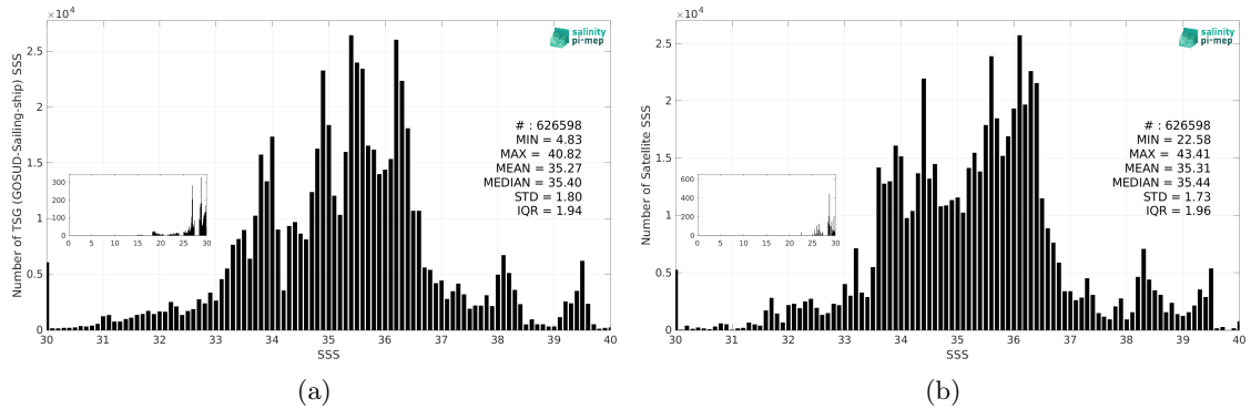
Figure 2: Histograms of SSS from TSG (GOSUD-Sailing-ship) (a) and SMOS SSS L3 v9 - 18 Days (CATDS-CEC-LOCEAN) (b) considering all match-up pairs per bins of 0.1 over the SMOS coastal zone (<800km) 60N-60S Pi-MEP region and for the full satellite product period.
