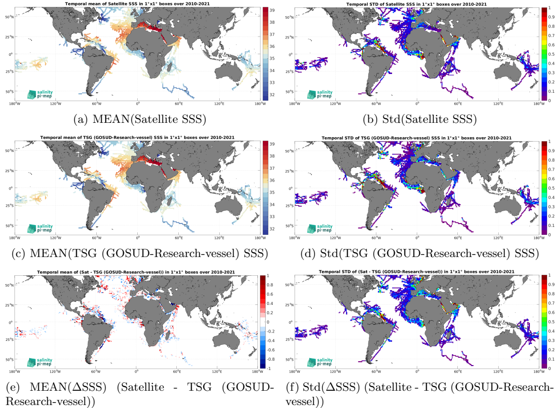
Figure 7: Temporal mean (left) and Std (right) of SSS from SMOS SSS L3 v9 - 18 Days (CATDS-CEC-LOCEAN) (top), TSG (GOSUD-Research-vessel) (middle), and of \Delta\text{SSS} (Satellite - TSG (GOSUD-Research-vessel)). Only match-up pairs are used to generate these maps.
