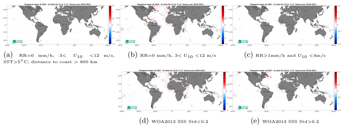
Figure 14: Temporal mean gridded over spatial boxes of size 1^\circ \times 1^\circ of \Delta\text{SSS} (SMOS SSS L3 v9 - 18 Days (CATDS-CEC-LOCEAN) - TSG (GOSUD-Research-vessel)) for 5 different subdatasets corresponding to:RR=0 mm/h, 3 < U_{10} < 12 m/s, SST >5^\circ\text{C} , distance to coast > 800 km (a), RR=0 mm/h, 3 < U_{10} < 12 m/s (b), RR >1 mm/h and U_{10} < 4 m/s (c), WOA2013 SSS Std <0.2 (d), WOA2013 SSS Std >0.2 (e).
