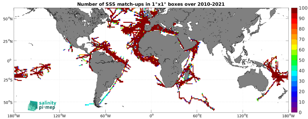
Figure 5: Number of SSS match-ups between TSG (GOSUD-Research-vessel) SSS and the SMOS SSS L3 v9 - 18 Days (CATDS-CEC-LOCEAN) SSS product for the SMOS coastal zone ( <800\text{km} ) 60N-60S Pi-MEP region over 1^\circ \times 1^\circ boxes and for the full satellite product period.
