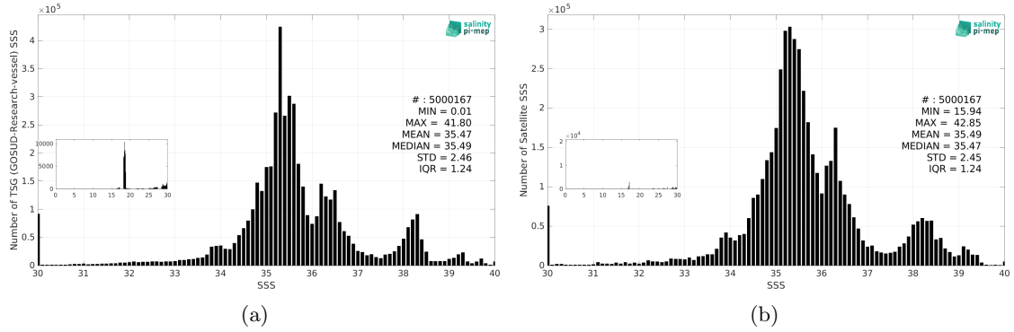
Figure 3: Histograms of SSS from TSG (GOSUD-Research-vessel) (a) and SMOS SSS L3 v9 - 18 Days (CATDS-CEC-LOCEAN) (b) considering all match-up pairs per bins of 0.1 over the SMOS coastal zone (<800km) 60N-60S Pi-MEP region and for the full satellite product period.
