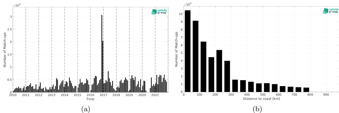
Figure 2: Number of match-ups between TSG (GOSUD-Research-vessel) and SMOS SSS L3 v9 - 18 Days (CATDS-CEC-LOCEAN) SSS as a function of time (a) and as function of the distance to coast (b) over the SMOS coastal zone (<800km) 60N-60S Pi-MEP region and for the full satellite product period.
