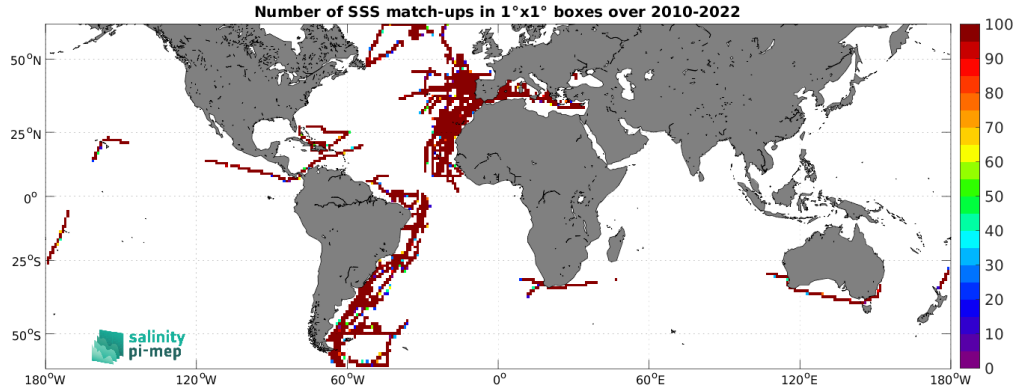
Figure 5: Number of SSS match-ups between TSG (CSIC-UTM) SSS and the SMOS SSS L3 v9 - 18 Days (CATDS-CEC-LOCEAN) SSS product for the SMOS coastal zone (<800km) 60N-60S Pi-MEP region over 1^\circ \times 1^\circ boxes and for the full satellite product period.
