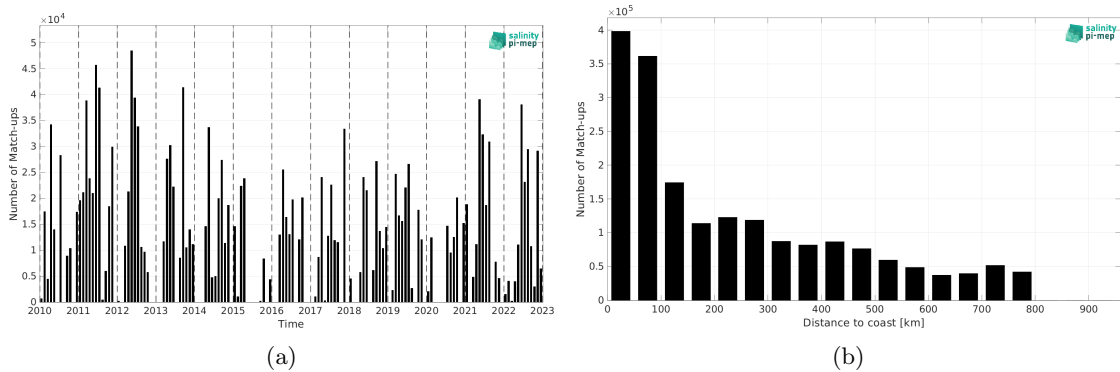
Figure 2: Number of match-ups between TSG (CSIC-UTM) and SMOS SSS L3 v9 - 18 Days (CATDS-CEC-LOCEAN) SSS as a function of time (a) and as function of the distance to coast (b) over the SMOS coastal zone (<800km) 60N-60S Pi-MEP region and for the full satellite product period.
