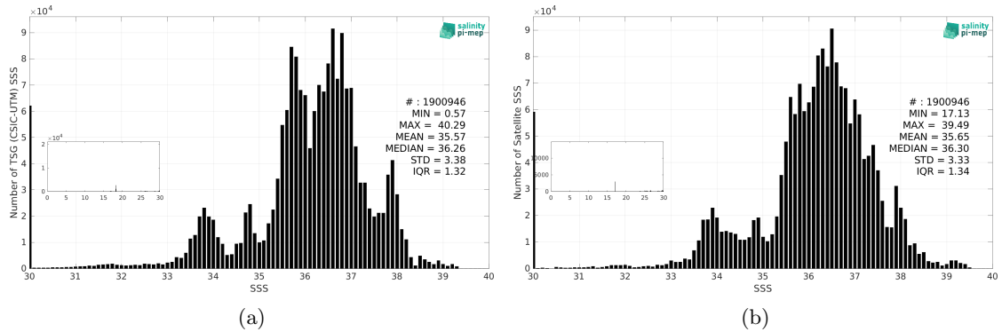
Figure 3: Histograms of SSS from TSG (CSIC-UTM) (a) and SMOS SSS L3 v9 - 18 Days (CATDS-CEC-LOCEAN) (b) considering all match-up pairs per bins of 0.1 over the SMOS coastal zone (<800km) 60N-60S Pi-MEP region and for the full satellite product period.
