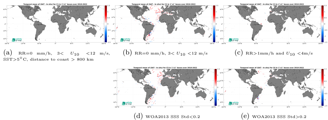
Figure 14: Temporal mean gridded over spatial boxes of size 1^\circ \times 1^\circ of \Delta SSS (SMOS SSS L3 v9 - 18 Days (CATDS-CEC-LOCEAN) - TSG (CSIC-UTM)) for 5 different subdatasets corresponding to:RR=0 mm/h, 3 < U_{10} < 12 m/s, SST >5^\circ\text{C} , distance to coast > 800 km (a), RR=0 mm/h, 3 < U_{10} < 12 m/s (b), RR >1 mm/h and U_{10} < 4 m/s (c), WOA2013 SSS Std <0.2 (d), WOA2013 SSS Std >0.2 (e).
