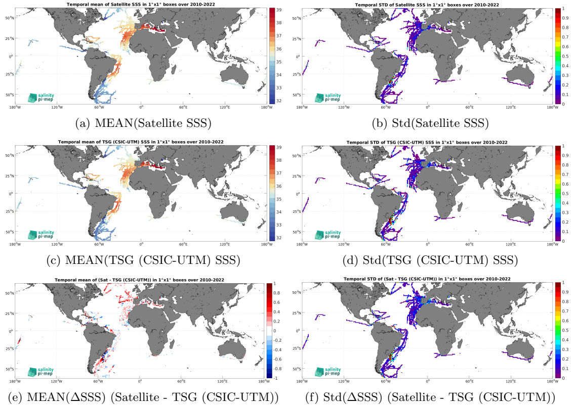
Figure 7: Temporal mean (left) and Std (right) of SSS from SMOS SSS L3 v9 - 18 Days (CATDS-CEC-LOCEAN) (top), TSG (CSIC-UTM) (middle), and of \Delta\text{SSS} (Satellite - TSG (CSIC-UTM)). Only match-up pairs are used to generate these maps.
