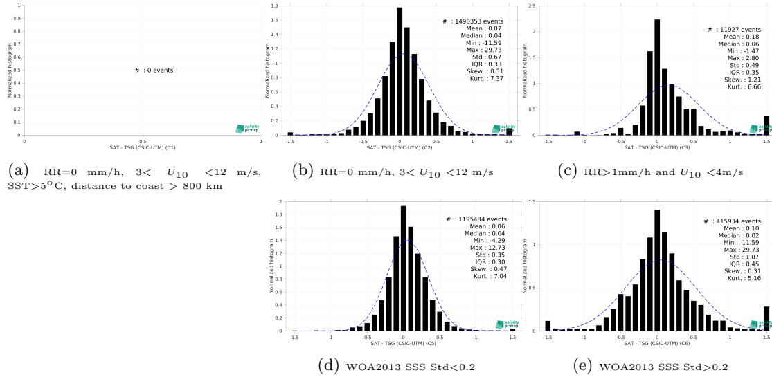
Figure 13: Normalized histogram of \Delta SSS (SMOS SSS L3 v9 - 18 Days (CATDS-CEC-LOCEAN) - TSG (CSIC-UTM)) for 5 different subdatasets corresponding to: RR=0 mm/h, 3 < U_{10} < 12 m/s, SST >5^{\circ} C, distance to coast > 800 km (a), RR=0 mm/h, 3 < U_{10} < 12 m/s (b), RR >1 mm/h and U_{10} < 4 m/s (c), WOA2013 SSS Std <0.2 (d), WOA2013 SSS Std >0.2 (e).
