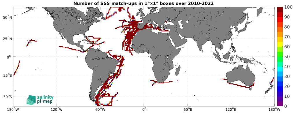
Figure 4: Number of SSS match-ups between TSG (CSIC-UTM) SSS and the SMOS SSS L3 v9 - 18 Days (CATDS-CEC-LOCEAN) SSS product for the SMOS coastal zone (<800km) 60N-60S Pi-MEP region over 1^\circ \times 1^\circ boxes and for the full satellite product period.
