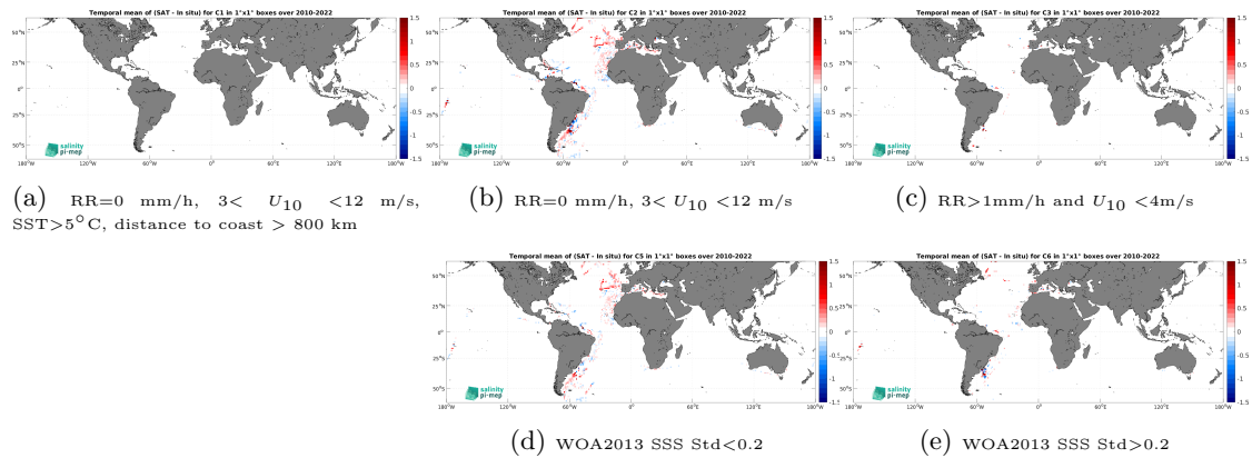
Figure 12: Temporal mean gridded over spatial boxes of size 1^\circ \times 1^\circ of \Delta SSS (SMOS SSS L3 v9 - 18 Days (CATDS-CEC-LOCEAN) - TSG (CSIC-UTM)) for 5 different subdatasets corresponding to:RR=0 mm/h, 3 < U_{10} < 12 m/s, SST >5^\circ C, distance to coast > 800 km (a), RR=0 mm/h, 3 < U_{10} < 12 m/s (b), RR >1 mm/h and U_{10} < 4 m/s (c), WOA2013 SSS Std <0.2 (d), WOA2013 SSS Std >0.2 (e).
