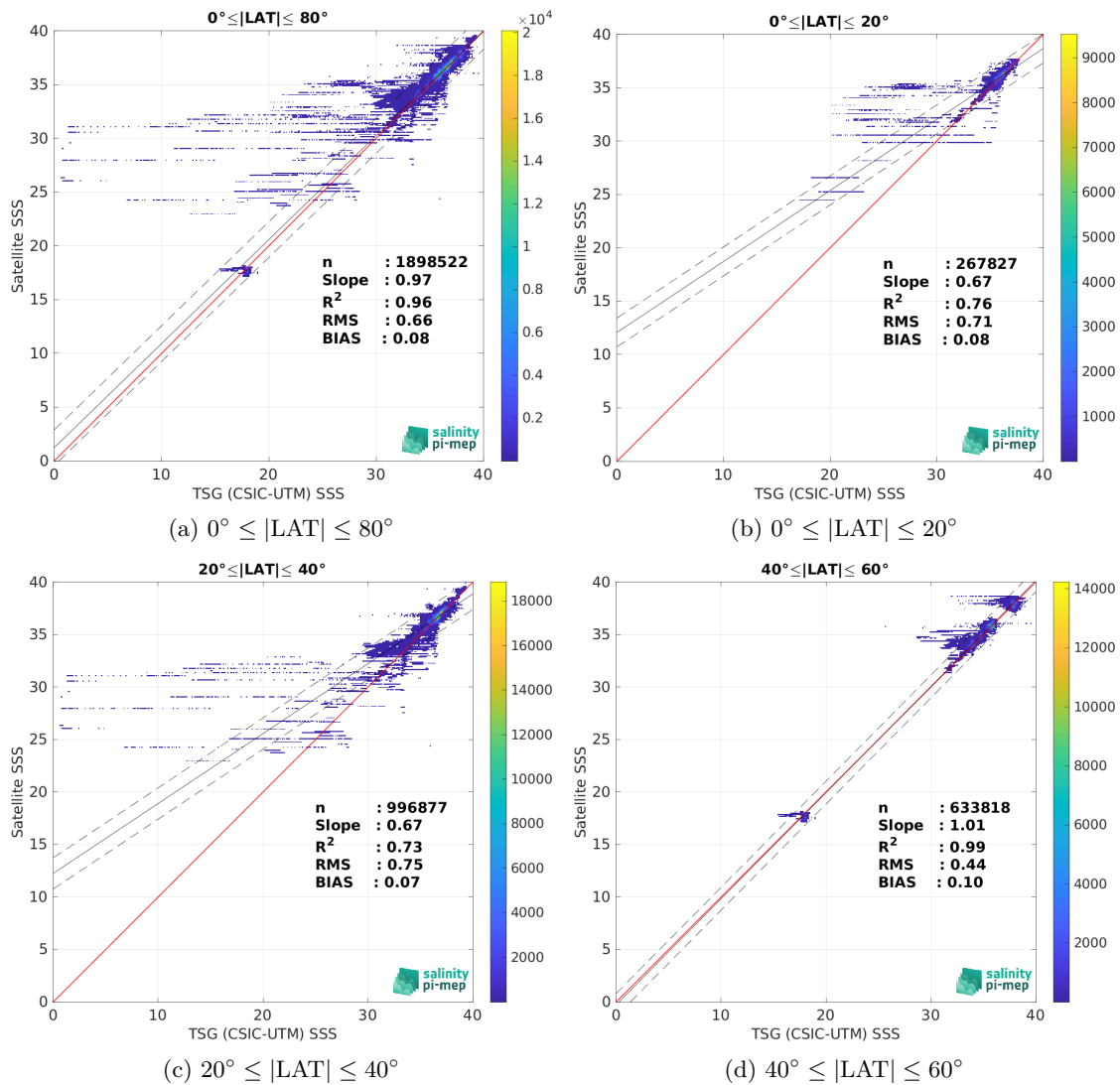
Figure 9: Contour maps of the concentration of SMOS SSS L3 v9 - 18 Days (CATDS-CEC-LOCEAN) SSS (y-axis) versus TSG (CSIC-UTM) SSS (x-axis) at match-up pairs for different latitude bands. For each plot, the red line shows x=y . The black thin and dashed lines indicate a linear fit through the data cloud and the \pm 95\% confidence levels, respectively. The number match-up pairs n , the slope and R^2 coefficient of the linear fit, the root mean square (RMS) and the mean bias between satellite and in situ data are indicated for each latitude band in each plots.
