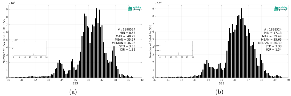
Figure 2: Histograms of SSS from TSG (CSIC-UTM) (a) and SMOS SSS L3 v9 - 18 Days (CATDS-CEC-LOCEAN) (b) considering all match-up pairs per bins of 0.1 over the SMOS coastal zone (<800km) 60N-60S Pi-MEP region and for the full satellite product period.
