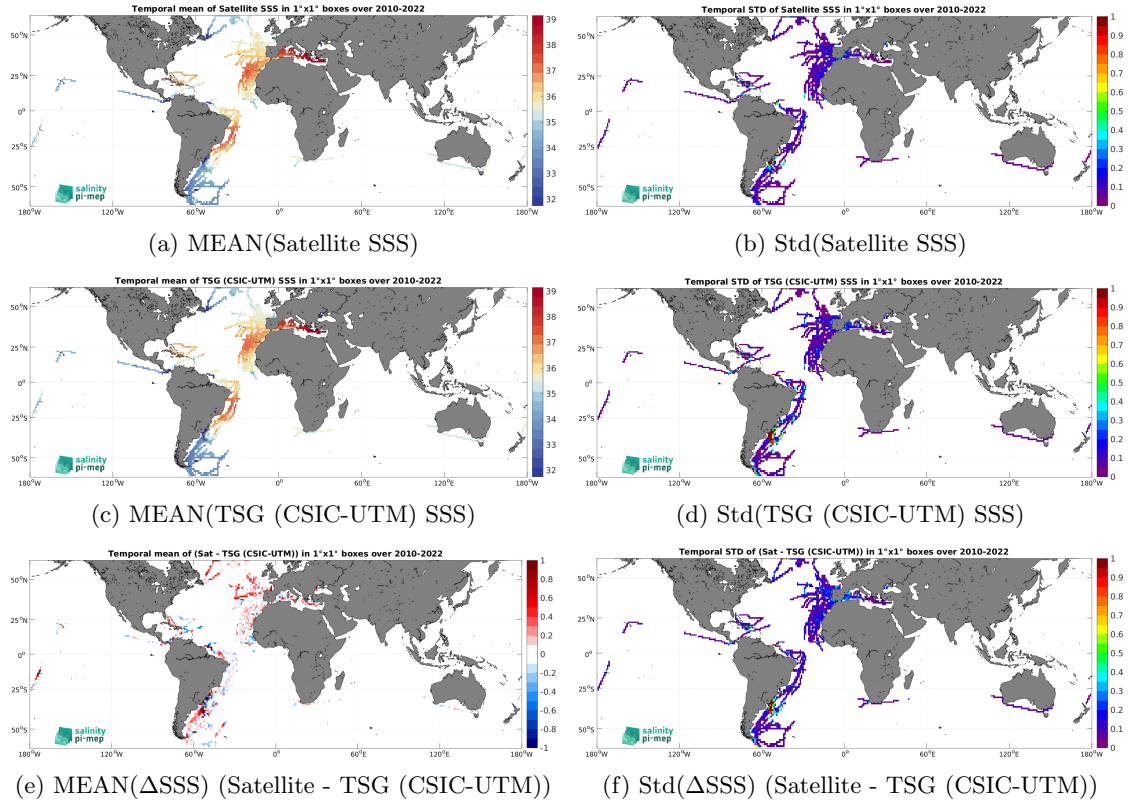
Figure 6: Temporal mean (left) and Std (right) of SSS from SMOS SSS L3 v9 - 18 Days (CATDS-CEC-LOCEAN) (top), TSG (CSIC-UTM) (middle), and of \Delta\text{SSS} (Satellite - TSG (CSIC-UTM)). Only match-up pairs are used to generate these maps.
