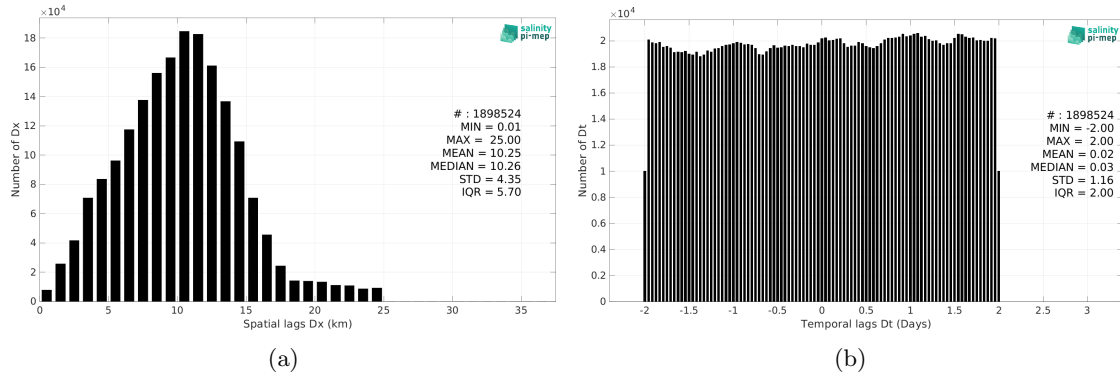
Figure 5: Histograms of the spatial (a) and temporal (b) lags between the location/time of the TSG (CSIC-UTM) measurement and the date of the corresponding SMOS SSS L3 v9 - 18 Days (CATDS-CEC-LOCEAN) SSS pixel.
