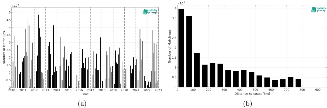
Figure 1: Number of match-ups between TSG (CSIC-UTM) and SMOS SSS L3 v9 - 18 Days (CATDS-CEC-LOCEAN) SSS as a function of time (a) and as function of the distance to coast (b) over the SMOS coastal zone (<800km) 60N-60S Pi-MEP region and for the full satellite product period.
