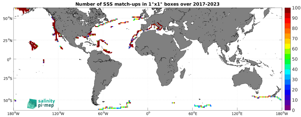
Figure 5: Number of SSS match-ups between Saildrone SSS and the SMOS SSS L3 v9 - 18 Days (CATDS-CEC-LOCEAN) SSS product for the SMOS coastal zone (<800km) 60N-60S Pi-MEP region over 1^{\circ} \times 1^{\circ} boxes and for the full satellite product period.
