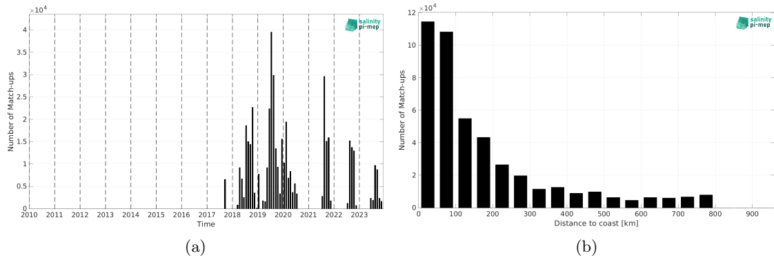
Figure 2: Number of match-ups between Saildrone and SMOS SSS L3 v9 - 18 Days (CATDS-CEC-LOCEAN) SSS as a function of time (a) and as function of the distance to coast (b) over the SMOS coastal zone (<800km) 60N-60S Pi-MEP region and for the full satellite product period.
