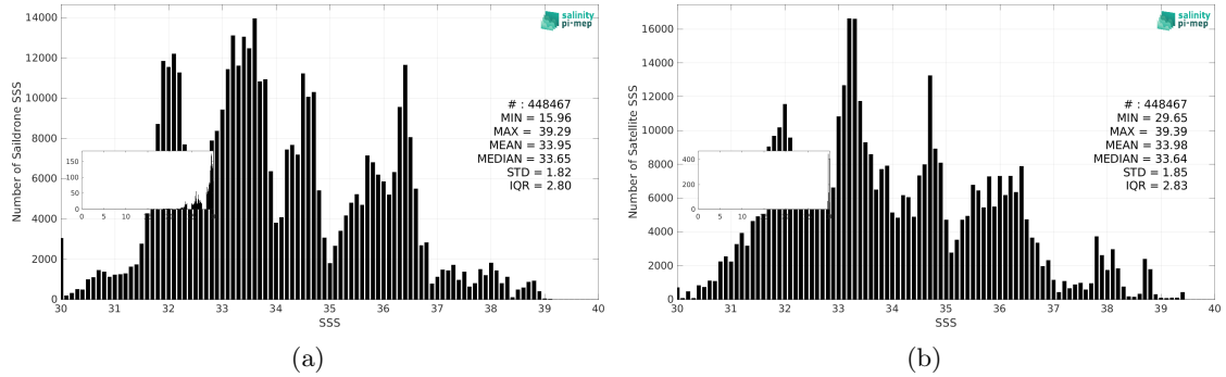
Figure 3: Histograms of SSS from Saildrone (a) and SMOS SSS L3 v9 - 18 Days (CATDS-CEC-LOCEAN) (b) considering all match-up pairs per bins of 0.1 over the SMOS coastal zone (<800km) 60N-60S Pi-MEP region and for the full satellite product period.
