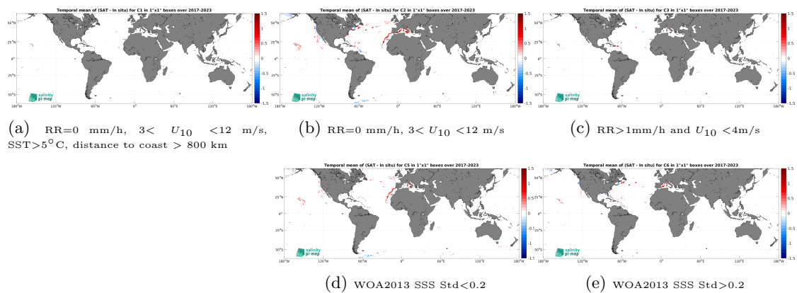
Figure 14: Temporal mean gridded over spatial boxes of size 1^\circ \times 1^\circ of \Delta SSS (SMOS SSS L3 v9 - 18 Days (CATDS-CEC-LOCEAN) - Saildrone) for 5 different subdatasets corresponding to:RR=0 mm/h, 3 < U_{10} < 12 m/s, SST >5^\circ\text{C} , distance to coast > 800 km (a), RR=0 mm/h, 3 < U_{10} < 12 m/s (b), RR >1 mm/h and U_{10} < 4 m/s (c), WOA2013 SSS Std <0.2 (d), WOA2013 SSS Std >0.2 (e).
