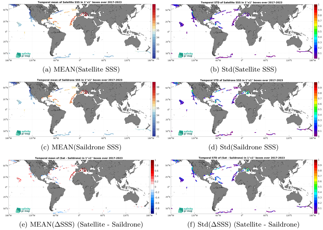
Figure 7: Temporal mean (left) and Std (right) of SSS from SMOS SSS L3 v9 - 18 Days (CATDS-CEC-LOCEAN) (top), Saildrone (middle), and of \Delta SSS (Satellite - Saildrone). Only match-up pairs are used to generate these maps.
