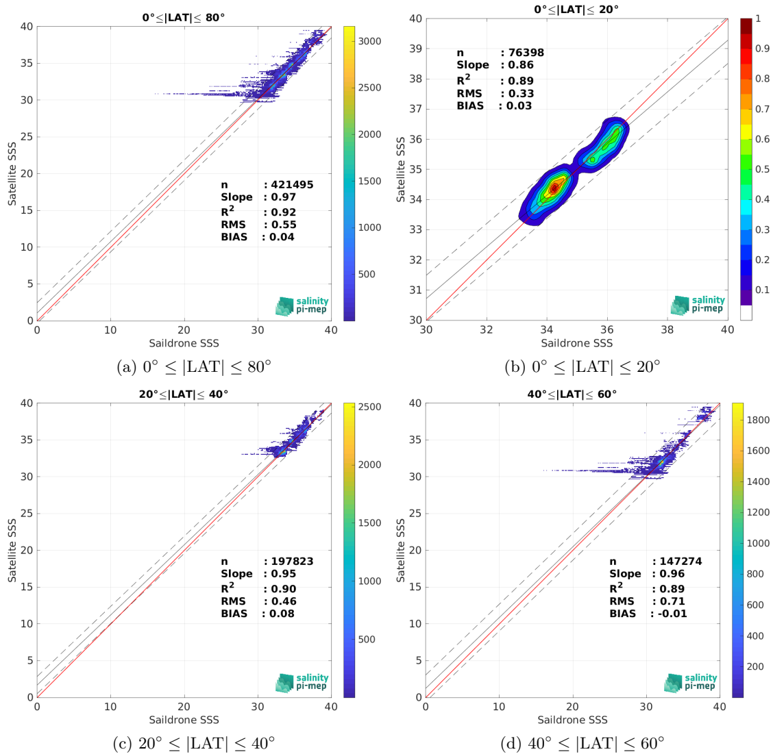
Figure 10: Contour maps of the concentration of SMOS SSS L3 v9 - 18 Days (CATDS-CEC-LOCEAN) SSS (y-axis) versus Sairdron SSS (x-axis) at match-up pairs for different latitude bands. For each plot, the red line shows x=y . The black thin and dashed lines indicate a linear fit through the data cloud and the \pm 95\% confidence levels, respectively. The number match-up pairs n , the slope and R^2 coefficient of the linear fit, the root mean square (RMS) and the mean bias between satellite and in situ data are indicated for each latitude band in each plots.
