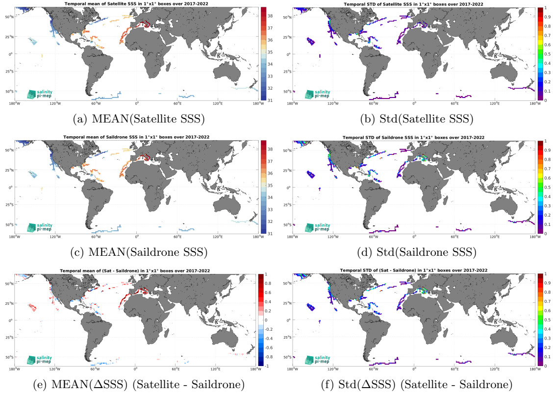
Figure 6: Temporal mean (left) and Std (right) of SSS from SMOS SSS L3 v9 - 18 Days (CATDS-CEC-LOCEAN) (top), Saildrone (middle), and of \Delta SSS (Satellite - Saildrone). Only match-up pairs are used to generate these maps.
