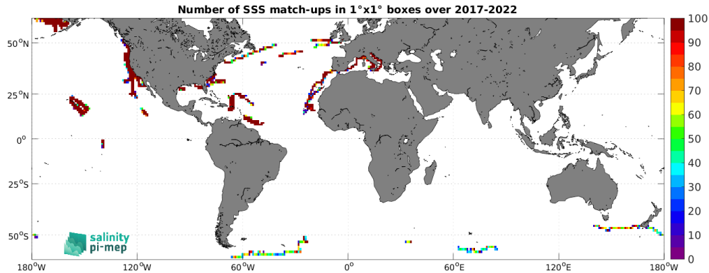
Figure 4: Number of SSS match-ups between Saildrone SSS and the SMOS SSS L3 v9 - 18 Days (CATDS-CEC-LOCEAN) SSS product for the SMOS coastal zone (<800km) 60N-60S Pi-MEP region over 1^\circ \times 1^\circ boxes and for the full satellite product period.
