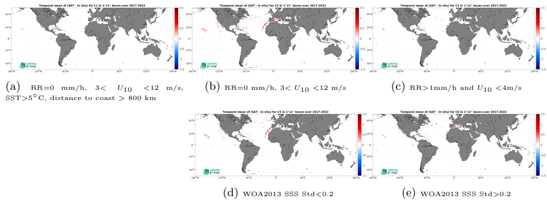
Figure 12: Temporal mean gridded over spatial boxes of size 1^\circ \times 1^\circ of \Delta SSS (SMOS SSS L3 v9 - 18 Days (CATDS-CEC-LOCEAN) - Saildrone) for 5 different subdatasets corresponding to:RR=0 mm/h, 3 < U_{10} < 12 m/s, SST >5^\circ C, distance to coast > 800 km (a), RR=0 mm/h, 3 < U_{10} < 12 m/s (b), RR >1 mm/h and U_{10} < 4 m/s (c), WOA2013 SSS Std <0.2 (d), WOA2013 SSS Std >0.2 (e).
