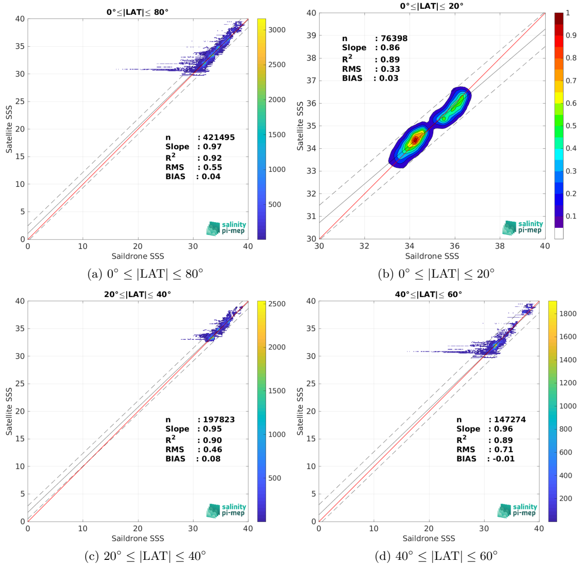
Figure 9: Contour maps of the concentration of SMOS SSS L3 v9 - 18 Days (CATDS-CEC-LOCEAN) SSS (y-axis) versus Sairdron SSS (x-axis) at match-up pairs for different latitude bands. For each plot, the red line shows x=y . The black thin and dashed lines indicate a linear fit through the data cloud and the \pm 95\% confidence levels, respectively. The number match-up pairs n , the slope and R^2 coefficient of the linear fit, the root mean square (RMS) and the mean bias between satellite and in situ data are indicated for each latitude band in each plots.
