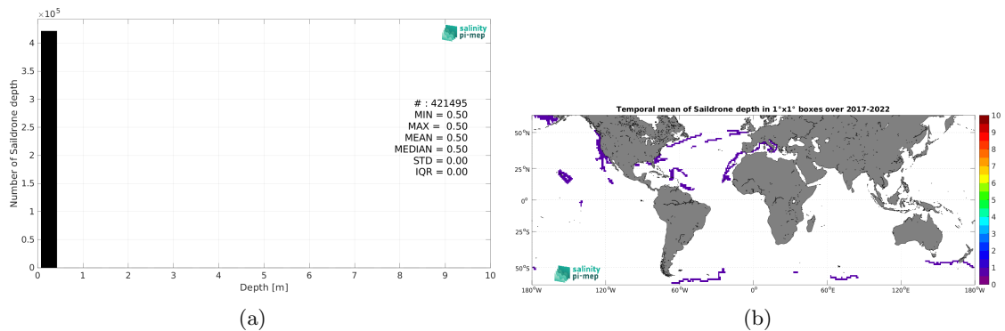
Figure 3: Histograms of the depth of the upper level SSS measurements from Sailldrone in the Match-up DataBase for the SMOS coastal zone (<800km) 60N-60S Pi-MEP region (a) and temporal mean spatial distribution of pressure of the in situ SSS data over 1^\circ \times 1^\circ boxes and for the full satellite product period (b).
