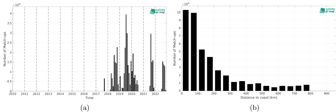
Figure 1: Number of match-ups between Saildrone and SMOS SSS L3 v9 - 18 Days (CATDS-CEC-LOCEAN) SSS as a function of time (a) and as function of the distance to coast (b) over the SMOS coastal zone (<800km) 60N-60S Pi-MEP region and for the full satellite product period.
