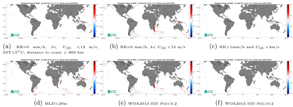
Figure 14: Temporal mean gridded over spatial boxes of size 1^\circ \times 1^\circ of \Delta SSS (SMOS SSS L3 v9 - 18 Days (CATDS-CEC-LOCEAN) - Marine mammals) for 6 different subdatasets corresponding to:RR=0 mm/h, 3 < U_{10} < 12 m/s, SST >5^\circ C, distance to coast > 800 km (a), RR=0 mm/h, 3 < U_{10} < 12 m/s (b), RR >1 mm/h and U_{10} < 4 m/s (c),MLD <20 m (d),WOA2013 SSS Std <0.2 (e),WOA2013 SSS Std >0.2 (f).
