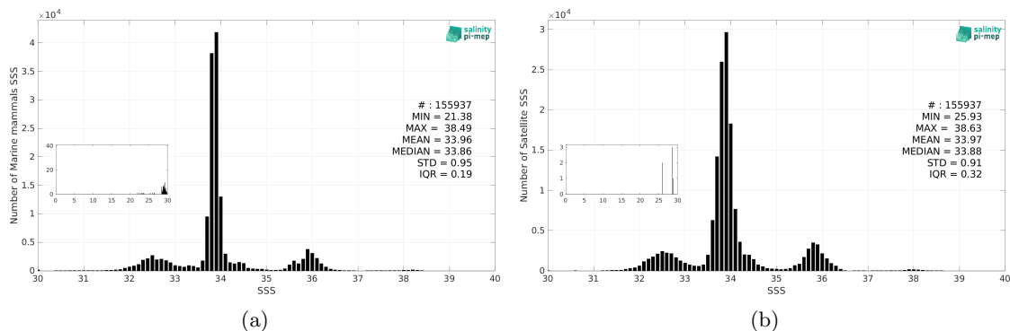
Figure 3: Histograms of SSS from Marine mammals (a) and SMOS SSS L3 v9 - 18 Days (CATDS-CEC-LOCEAN) (b) considering all match-up pairs per bins of 0.1 over the SMOS coastal zone (<800km) 60N-60S Pi-MEP region and for the full satellite product period.
