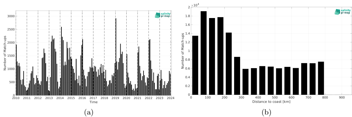
Figure 2: Number of match-ups between Marine mammals and SMOS SSS L3 v9 - 18 Days (CATDS-CEC-LOCEAN) SSS as a function of time (a) and as function of the distance to coast (b) over the SMOS coastal zone (<800km) 60N-60S Pi-MEP region and for the full satellite product period.
