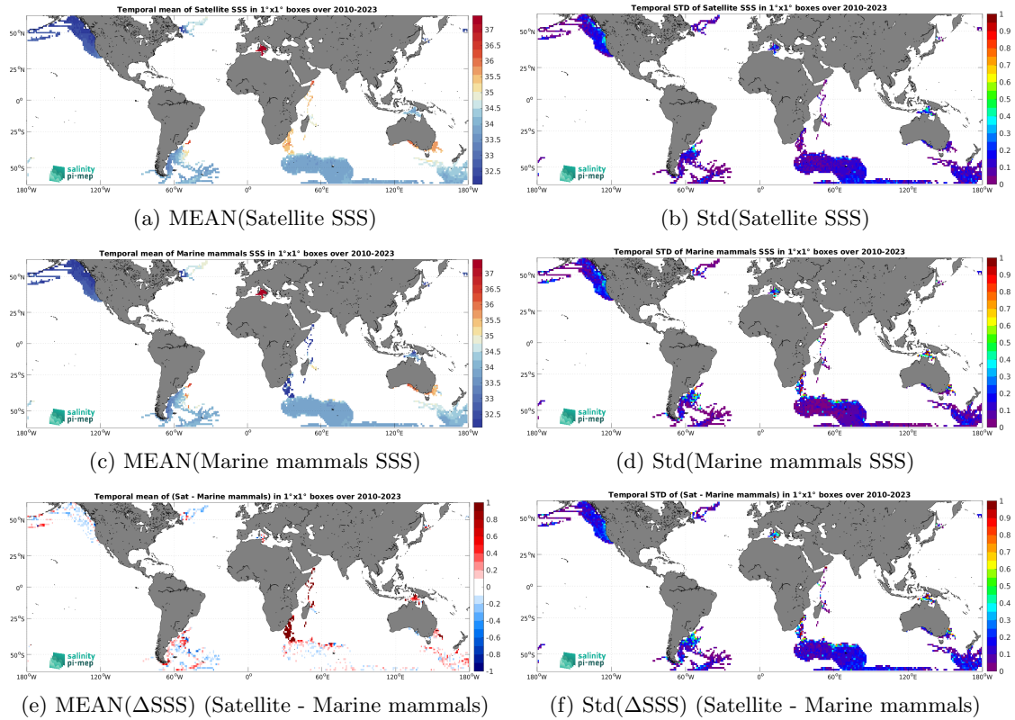
Figure 7: Temporal mean (left) and Std (right) of SSS from SMOS SSS L3 v9 - 18 Days (CATDS-CEC-LOCEAN) (top), Marine mammals (middle), and of \Delta SSS (Satellite - Marine mammals). Only match-up pairs are used to generate these maps.
