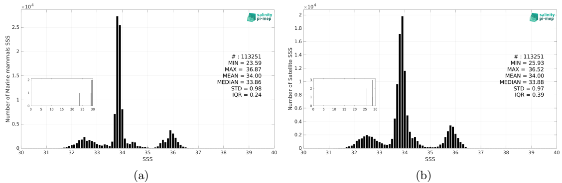
Figure 2: Histograms of SSS from Marine mammals (a) and SMOS SSS L3 v9 - 18 Days (CATDS-CEC-LOCEAN) (b) considering all match-up pairs per bins of 0.1 over the SMOS coastal zone (<800km) 60N-60S Pi-MEP region and for the full satellite product period.
