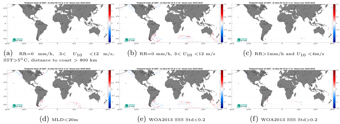
Figure 12: Temporal mean gridded over spatial boxes of size 1^{\circ}\times 1^{\circ} of \Delta\text{SSS} (SMOS SSS L3 v9 - 18 Days (CATDS-CEC-LOCEAN) - Marine mammals) for 6 different subdatasets corresponding to:RR=0 mm/h, 3 < U_{10} < 12 m/s, SST >5^{\circ}\text{C} , distance to coast > 800 km (a), RR=0 mm/h, 3 < U_{10} < 12 m/s (b), RR >1\text{mm/h} and U_{10} < 4\text{m/s} (c),MLD <20\text{m} (d),WOA2013 SSS Std <0.2 (e),WOA2013 SSS Std >0.2 (f).
