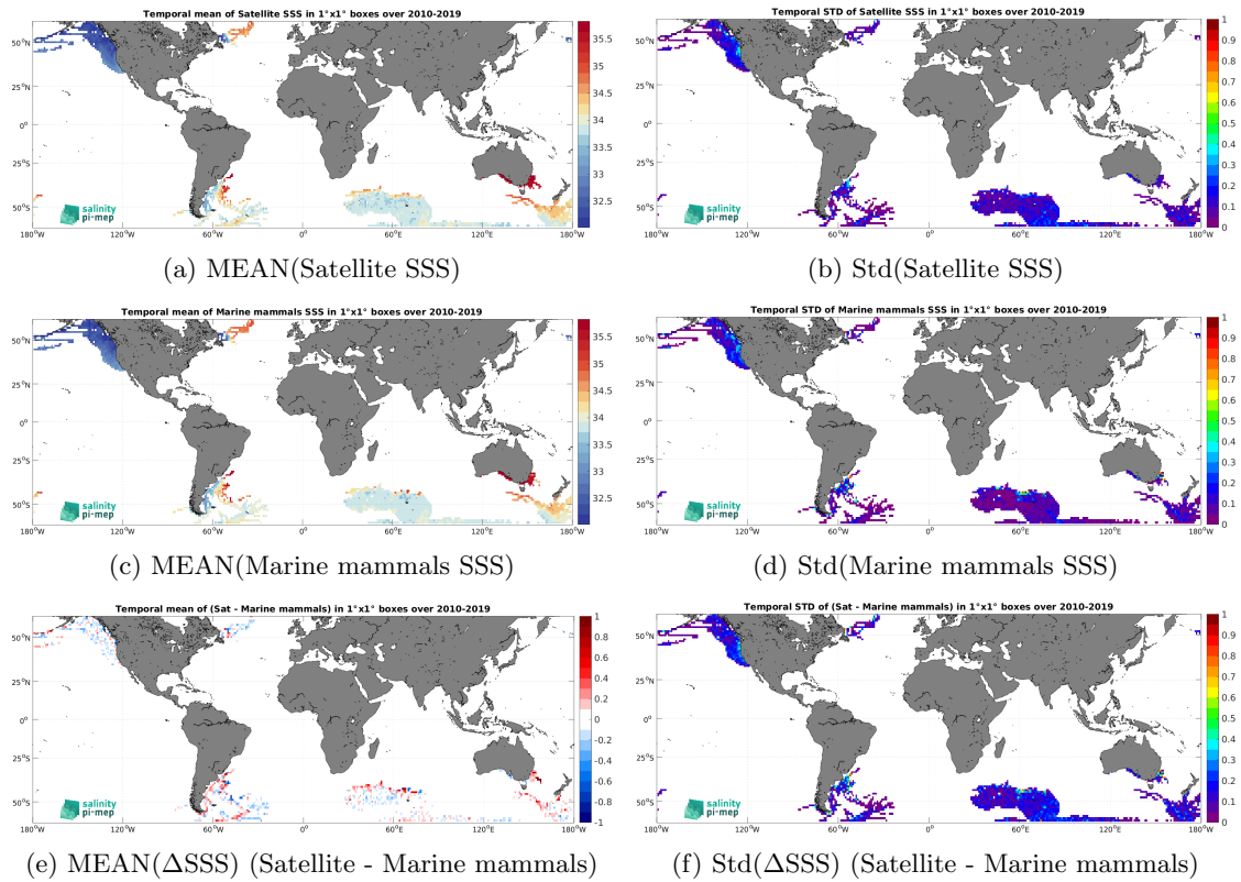
Figure 6: Temporal mean (left) and Std (right) of SSS from SMOS SSS L3 v9 - 18 Days (CATDS-CEC-LOCEAN) (top), Marine mammals (middle), and of \Delta SSS (Satellite - Marine mammals). Only match-up pairs are used to generate these maps.
