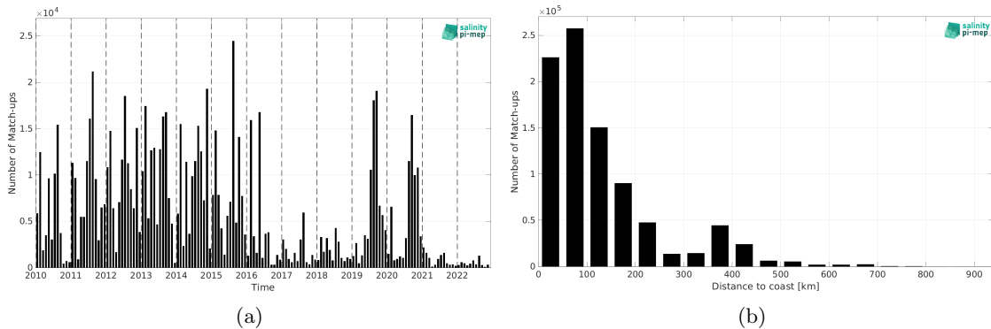
Figure 2: Number of match-ups between ICES and SMOS SSS L3 v9 - 18 Days (CATDS-CEC-LOCEAN) SSS as a function of time (a) and as function of the distance to coast (b) over the SMOS coastal zone (<800km) 60N-60S Pi-MEP region and for the full satellite product period.
