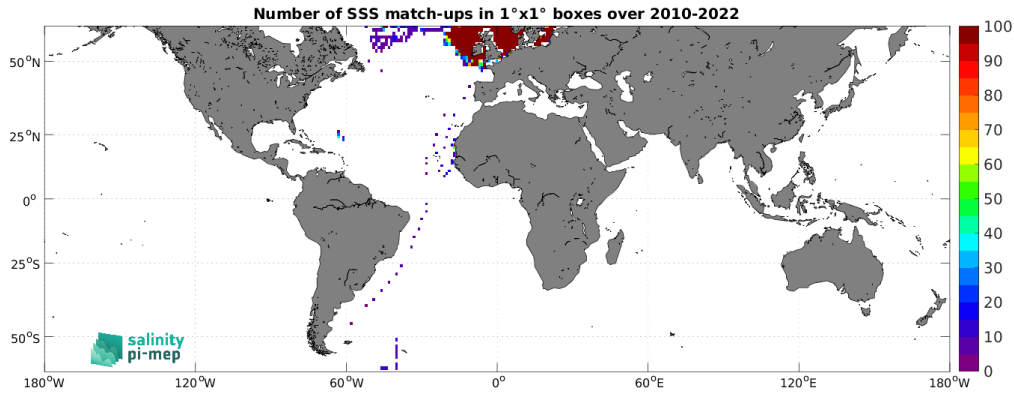
Figure 5: Number of SSS match-ups between ICES SSS and the SMOS SSS L3 v9 - 18 Days (CATDS-CEC-LOCEAN) SSS product for the SMOS coastal zone (<800km) 60N-60S Pi-MEP region over 1^{\circ} \times 1^{\circ} boxes and for the full satellite product period.
