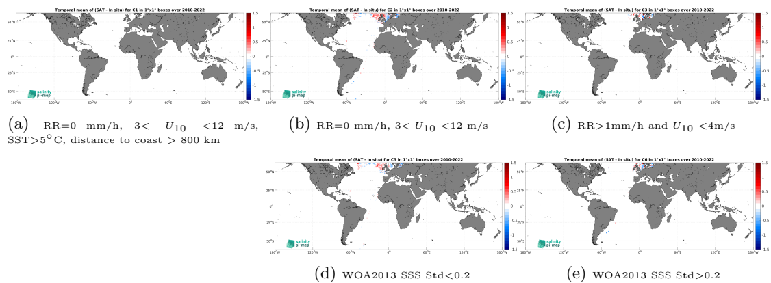
Figure 14: Temporal mean gridded over spatial boxes of size 1^\circ \times 1^\circ of \Delta\text{SSS} (SMOS SSS L3 v9 - 18 Days (CATDS-CEC-LOCEAN) - ICES) for 5 different subdatasets corresponding to:RR=0 mm/h, 3 < U_{10} < 12 m/s, SST >5^\circ\text{C} , distance to coast > 800 km (a), RR=0 mm/h, 3 < U_{10} < 12 m/s (b), RR >1 mm/h and U_{10} < 4 m/s (c), WOA2013 SSS Std <0.2 (d), WOA2013 SSS Std >0.2 (e).
