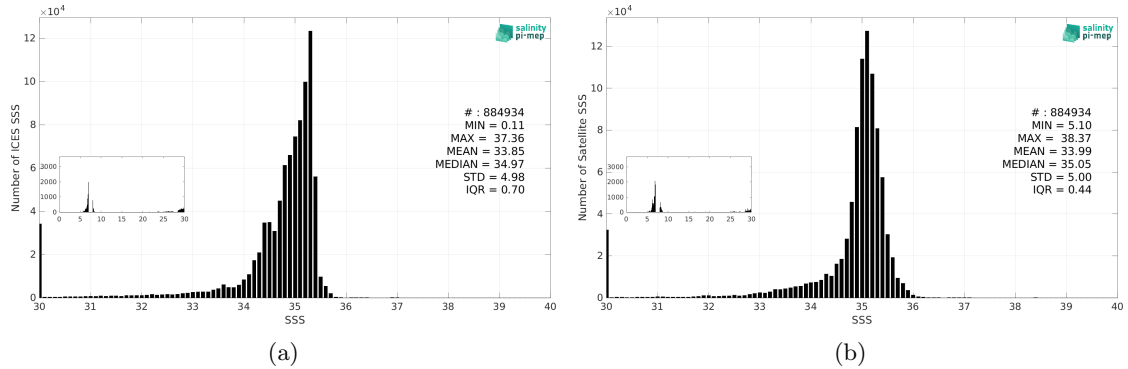
Figure 3: Histograms of SSS from ICES (a) and SMOS SSS L3 v9 - 18 Days (CATDS-CEC-LOCEAN) (b) considering all match-up pairs per bins of 0.1 over the SMOS coastal zone (<800km) 60N-60S Pi-MEP region and for the full satellite product period.
