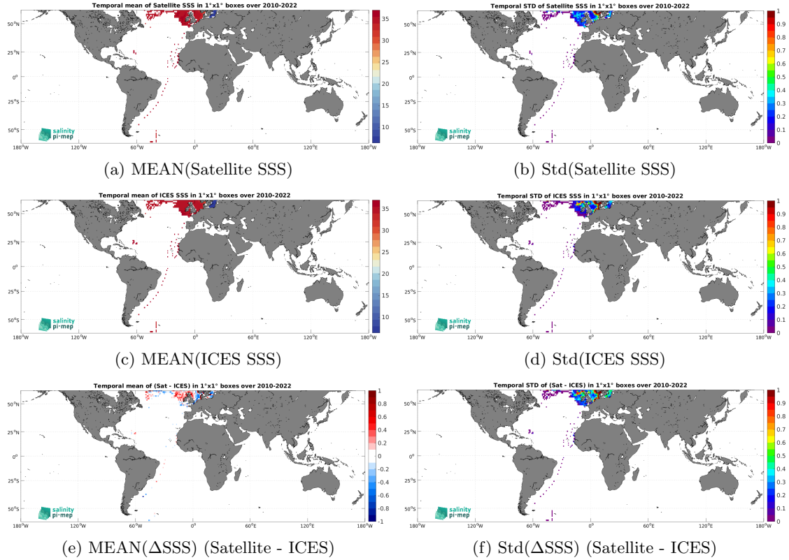
Figure 7: Temporal mean (left) and Std (right) of SSS from SMOS SSS L3 v9 - 18 Days (CATDS-CEC-LOCEAN) (top), ICES (middle), and of \Delta SSS (Satellite - ICES). Only match-up pairs are used to generate these maps.
