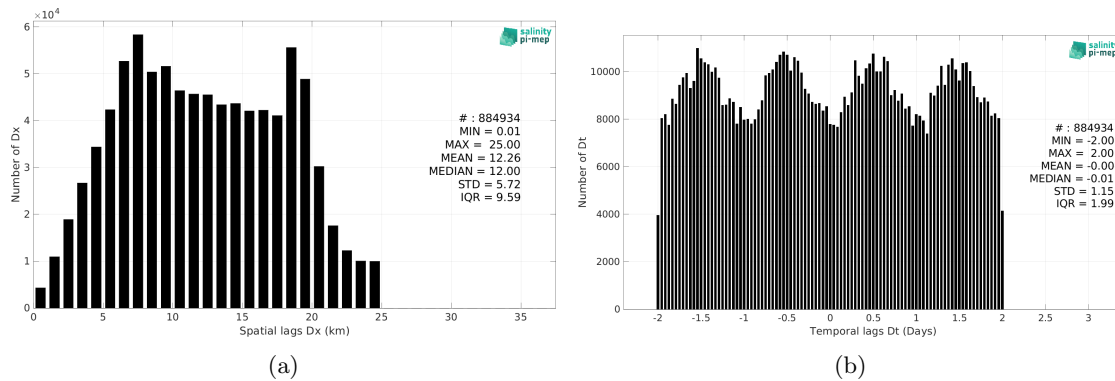
Figure 6: Histograms of the spatial (a) and temporal (b) lags between the location/time of the ICES measurement and the date of the corresponding SMOS SSS L3 v9 - 18 Days (CATDS-CEC-LOCEAN) SSS pixel.
