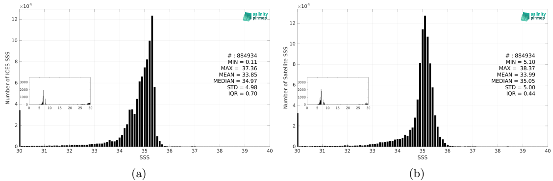
Figure 2: Histograms of SSS from ICES (a) and SMOS SSS L3 v9 - 18 Days (CATDS-CEC-LOCEAN) (b) considering all match-up pairs per bins of 0.1 over the SMOS coastal zone (<800km) 60N-60S Pi-MEP region and for the full satellite product period.
