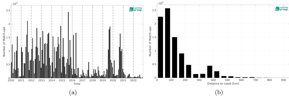
Figure 1: Number of match-ups between ICES and SMOS SSS L3 v9 - 18 Days (CATDS-CEC-LOCEAN) SSS as a function of time (a) and as function of the distance to coast (b) over the SMOS coastal zone (<800km) 60N-60S Pi-MEP region and for the full satellite product period.
