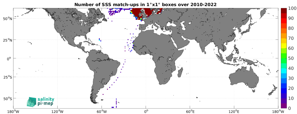
Figure 4: Number of SSS match-ups between ICES SSS and the SMOS SSS L3 v9 - 18 Days (CATDS-CEC-LOCEAN) SSS product for the SMOS coastal zone ( <800\text{km} ) 60N-60S Pi-MEP region over 1^\circ \times 1^\circ boxes and for the full satellite product period.
