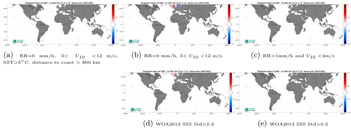
Figure 12: Temporal mean gridded over spatial boxes of size 1^\circ \times 1^\circ of \Delta\text{SSS} (SMOS SSS L3 v9 - 18 Days (CATDS-CEC-LOCEAN) - ICES) for 5 different subdatasets corresponding to:RR=0 mm/h, 3 < U_{10} < 12 m/s, SST >5^\circ\text{C} , distance to coast > 800 km (a), RR=0 mm/h, 3 < U_{10} < 12 m/s (b), RR >1 mm/h and U_{10} < 4 m/s (c), WOA2013 SSS Std <0.2 (d), WOA2013 SSS Std >0.2 (e).
