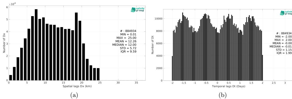
Figure 5: Histograms of the spatial (a) and temporal (b) lags between the location/time of the ICES measurement and the date of the corresponding SMOS SSS L3 v9 - 18 Days (CATDS-CEC-LOCEAN) SSS pixel.
