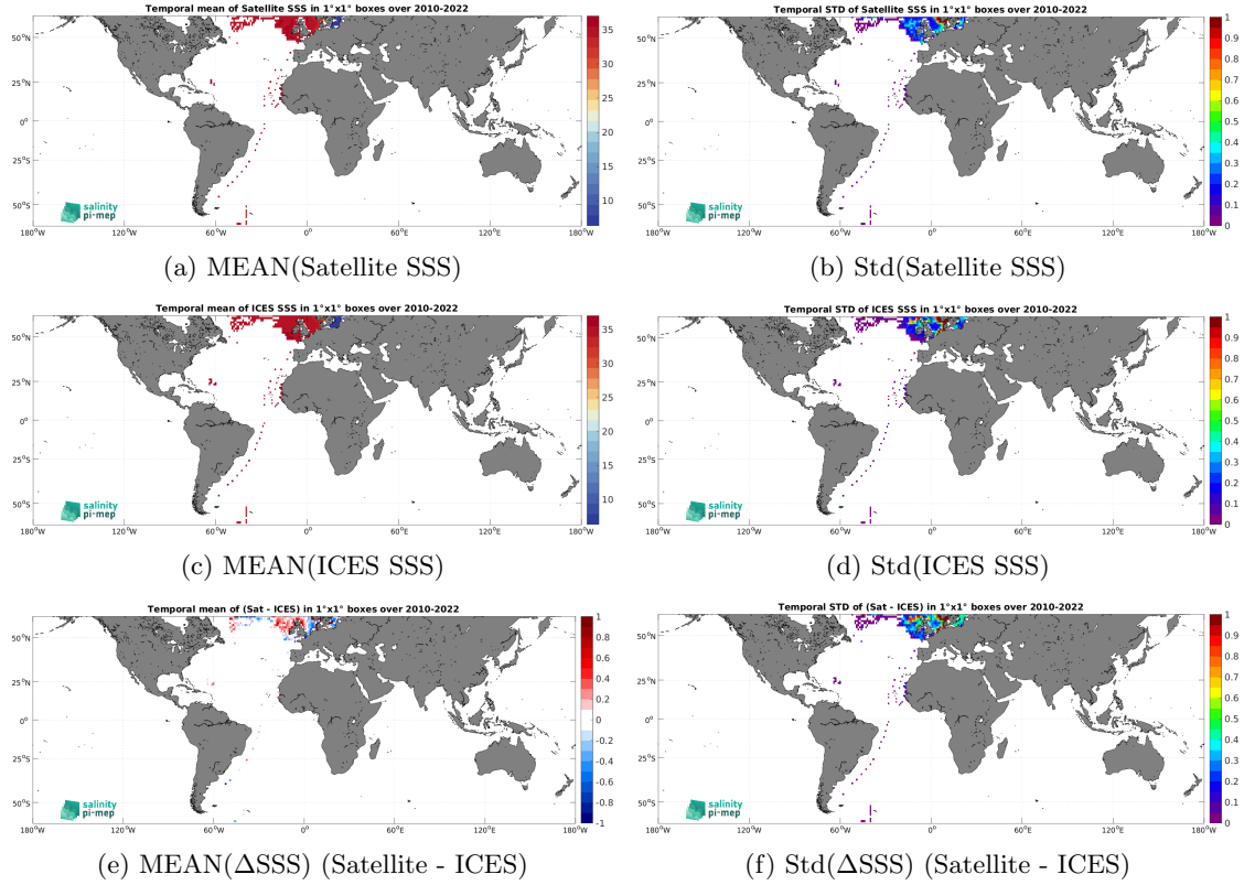
Figure 6: Temporal mean (left) and Std (right) of SSS from SMOS SSS L3 v9 - 18 Days (CATDS-CEC-LOCEAN) (top), ICES (middle), and of \Delta\text{SSS} (Satellite - ICES). Only match-up pairs are used to generate these maps.
