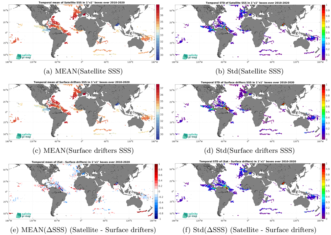
Figure 5: Temporal mean (left) and Std (right) of SSS from SMOS SSS L3 v9 - 18 Days (CATDS-CEC-LOCEAN) (top), Surface drifters (middle), and of \Delta SSS (Satellite - Surface drifters). Only match-up pairs are used to generate these maps.
