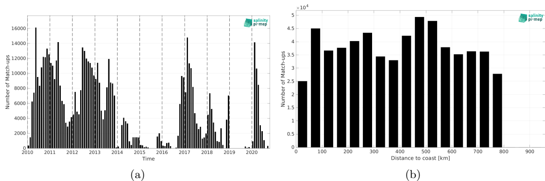
Figure 1: Number of match-ups between Surface drifters and SMOS SSS L3 v9 - 18 Days (CATDS-CEC-LOCEAN) SSS as a function of time (a) and as function of the distance to coast (b) over the SMOS coastal zone (<800km) 60N-60S Pi-MEP region and for the full satellite product period.
