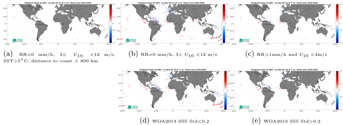
Figure 11: Temporal mean gridded over spatial boxes of size 1^\circ \times 1^\circ of \Delta SSS (SMOS SSS L3 v9 - 18 Days (CATDS-CEC-LOCEAN) - Surface drifters) for 5 different subdatasets corresponding to:RR=0 mm/h, 3 < U_{10} < 12 m/s, SST >5^\circ C, distance to coast > 800 km (a), RR=0 mm/h, 3 < U_{10} < 12 m/s (b), RR >1 mm/h and U_{10} < 4 m/s (c), WOA2013 SSS Std <0.2 (d), WOA2013 SSS Std >0.2 (e).
