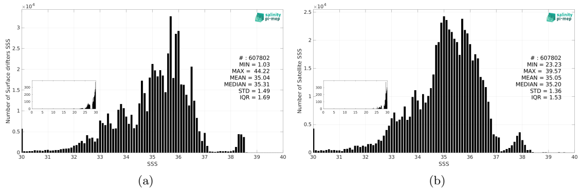
Figure 2: Histograms of SSS from Surface drifters (a) and SMOS SSS L3 v9 - 18 Days (CATDS-CEC-LOCEAN) (b) considering all match-up pairs per bins of 0.1 over the SMOS coastal zone (<800km) 60N-60S Pi-MEP region and for the full satellite product period.
