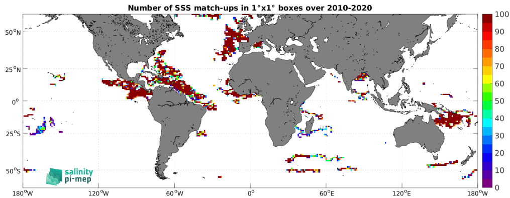
Figure 3: Number of SSS match-ups between Surface drifters SSS and the SMOS SSS L3 v9 - 18 Days (CATDS-CEC-LOCEAN) SSS product for the SMOS coastal zone (<800km) 60N-60S Pi-MEP region over 1^\circ \times 1^\circ boxes and for the full satellite product period.
