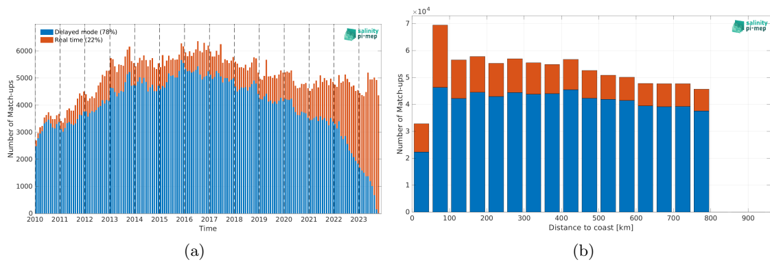
Figure 1: Number of match-ups between Argo and SMOS SSS L3 v9 - 18 Days (CATDS-CEC-LOCEAN) SSS as a function of time (a) and as function of the distance to coast (b) over the SMOS coastal zone (<800km) 60N-60S Pi-MEP region and for the full satellite product period.
