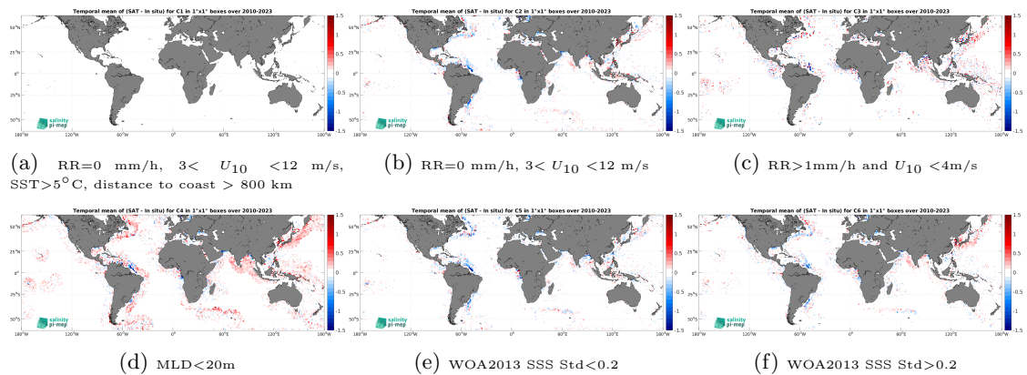
Figure 12: Temporal mean gridded over spatial boxes of size 1^\circ \times 1^\circ of \Delta SSS (SMOS SSS L3 v9 - 18 Days (CATDS-CEC-LOCEAN) - Argo) for 6 different subdatasets corresponding to:RR=0 mm/h, 3 < U_{10} < 12 m/s, SST >5^\circ C, distance to coast > 800 km (a), RR=0 mm/h, 3 < U_{10} < 12 m/s (b), RR >1 mm/h and U_{10} < 4 m/s (c),MLD <20 m (d),WOA2013 SSS Std <0.2 (e),WOA2013 SSS Std >0.2 (f).
