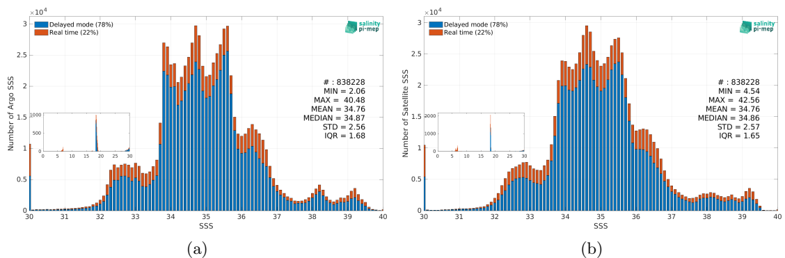
Figure 2: Histograms of SSS from Argo (a) and SMOS SSS L3 v9 - 18 Days (CATDS-CEC-LOCEAN) (b) considering all match-up pairs per bins of 0.1 over the SMOS coastal zone (<800km) 60N-60S Pi-MEP region and for the full satellite product period.
