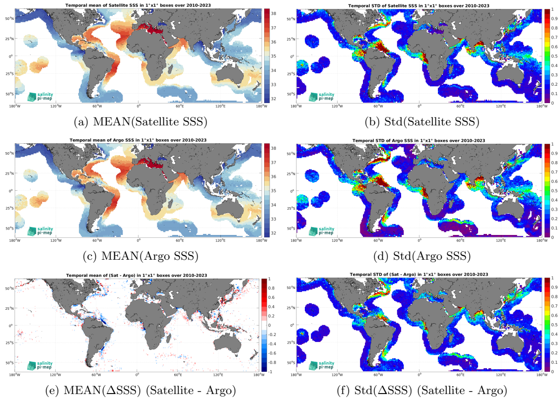
Figure 6: Temporal mean (left) and Std (right) of SSS from SMOS SSS L3 v9 - 18 Days (CATDS-CEC-LOCEAN) (top), Argo (middle), and of \Delta SSS (Satellite - Argo). Only match-up pairs are used to generate these maps.
