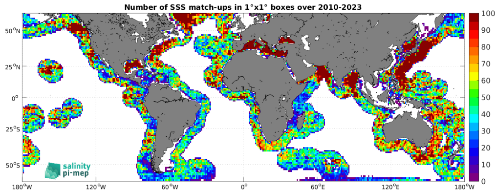
Figure 4: Number of SSS match-ups between Argo SSS and the SMOS SSS L3 v9 - 18 Days (CATDS-CEC-LOCEAN) SSS product for the SMOS coastal zone ( <800\text{km} ) 60N-60S Pi-MEP region over 1^\circ \times 1^\circ boxes and for the full satellite product period.
