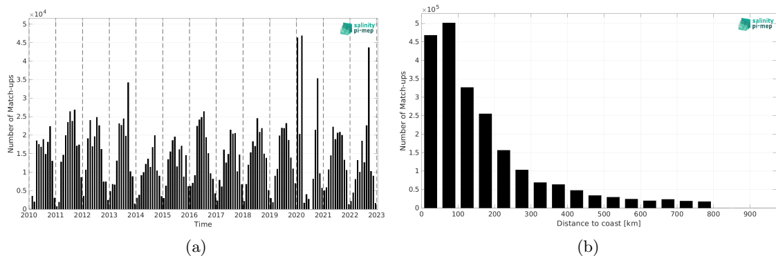
Figure 1: Number of match-ups between TSG (SAMOS) and SMOS SSS L3 v8 - 9 Days (CATDS-CEC-LOCEAN) SSS as a function of time (a) and as function of the distance to coast (b) over the SMOS coastal zone (<800km) 60N-60S Pi-MEP region and for the full satellite product period.
