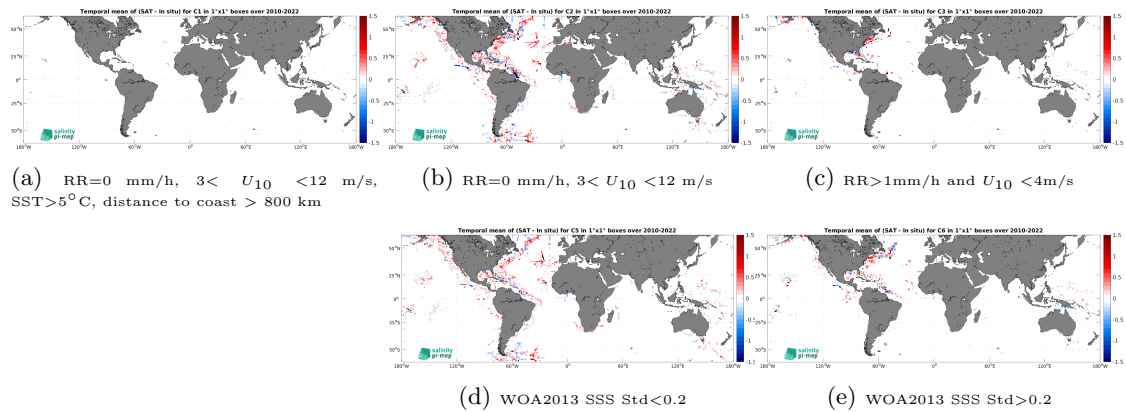
Figure 12: Temporal mean gridded over spatial boxes of size 1^\circ \times 1^\circ of \Delta SSS (SMOS SSS L3 v8 - 9 Days (CATDS-CEC-LOCEAN) - TSG (SAMOS)) for 5 different subdatasets corresponding to:RR=0 mm/h, 3 < U_{10} < 12 m/s, SST >5^\circ C, distance to coast > 800 km (a), RR=0 mm/h, 3 < U_{10} < 12 m/s (b), RR >1 mm/h and U_{10} < 4 m/s (c), WOA2013 SSS Std <0.2 (d), WOA2013 SSS Std >0.2 (e).
