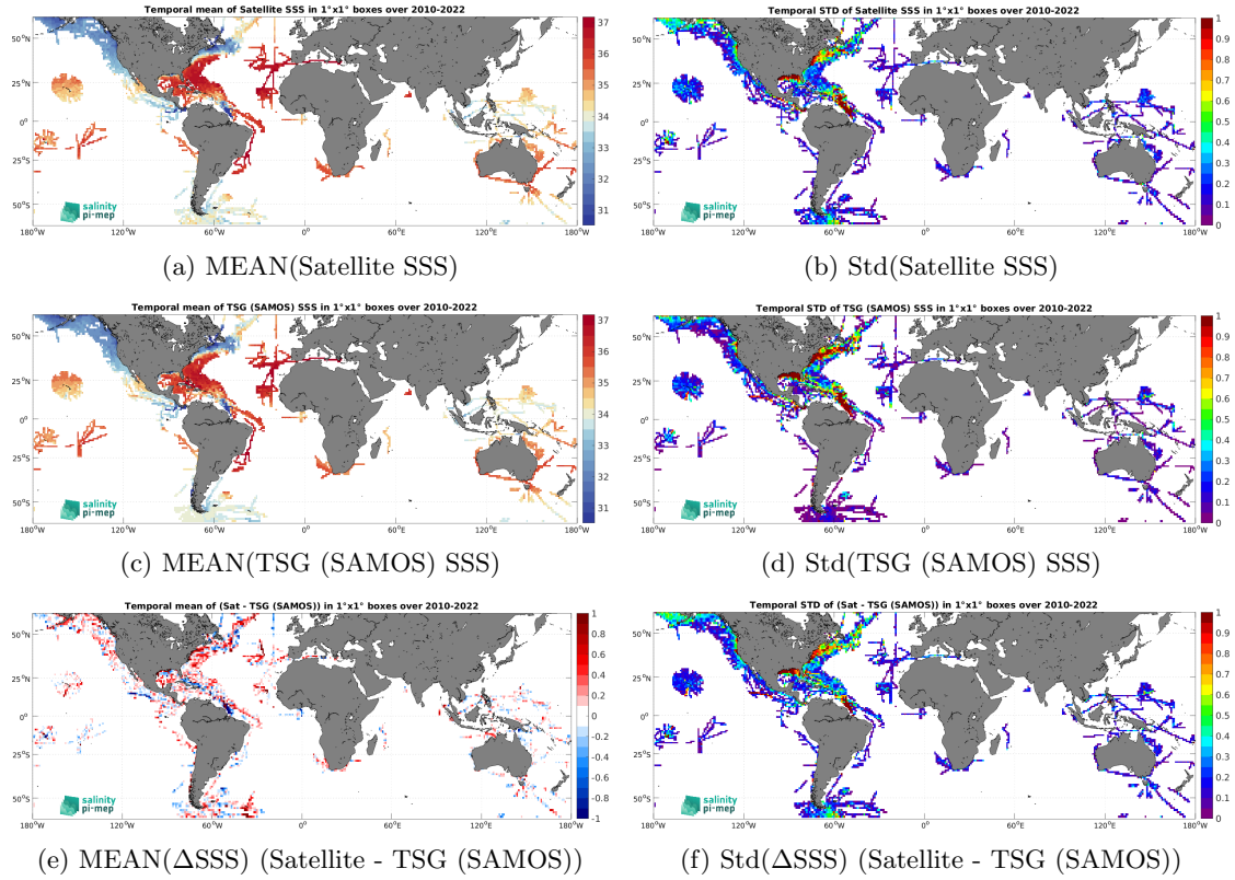
Figure 6: Temporal mean (left) and Std (right) of SSS from SMOS SSS L3 v8 - 9 Days (CATDS-CEC-LOCEAN) (top), TSG (SAMOS) (middle), and of \Delta SSS (Satellite - TSG (SAMOS)). Only match-up pairs are used to generate these maps.
