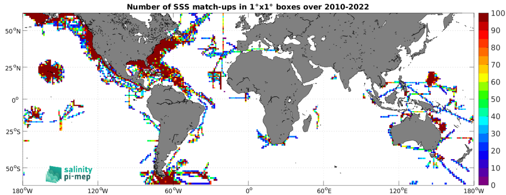
Figure 4: Number of SSS match-ups between TSG (SAMOS) SSS and the SMOS SSS L3 v8 - 9 Days (CATDS-CEC-LOCEAN) SSS product for the SMOS coastal zone (<800km) 60N-60S Pi-MEP region over 1^\circ \times 1^\circ boxes and for the full satellite product period.
