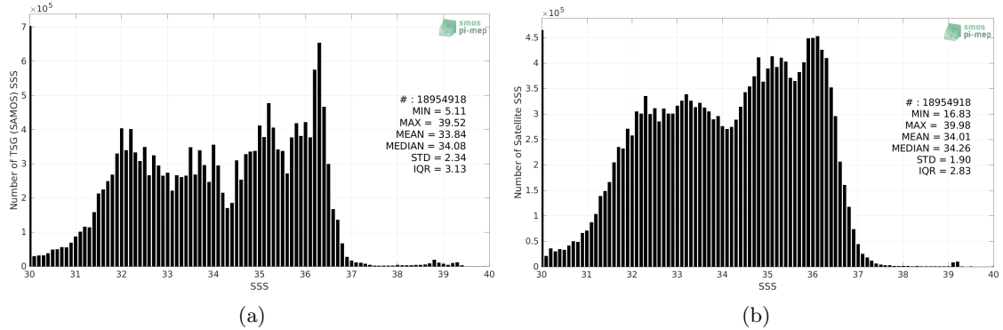
Figure 2: Histograms of SSS from TSG (SAMOS) (a) and SMOS SSS L3 v8 - 9 Days (CATDS-CECOS-LOCEAN) (b) considering all match-up pairs per bins of 0.1 over the SMOS coastal zone (<800km) 60N-60S Pi-MEP region and for the full satellite product period.
