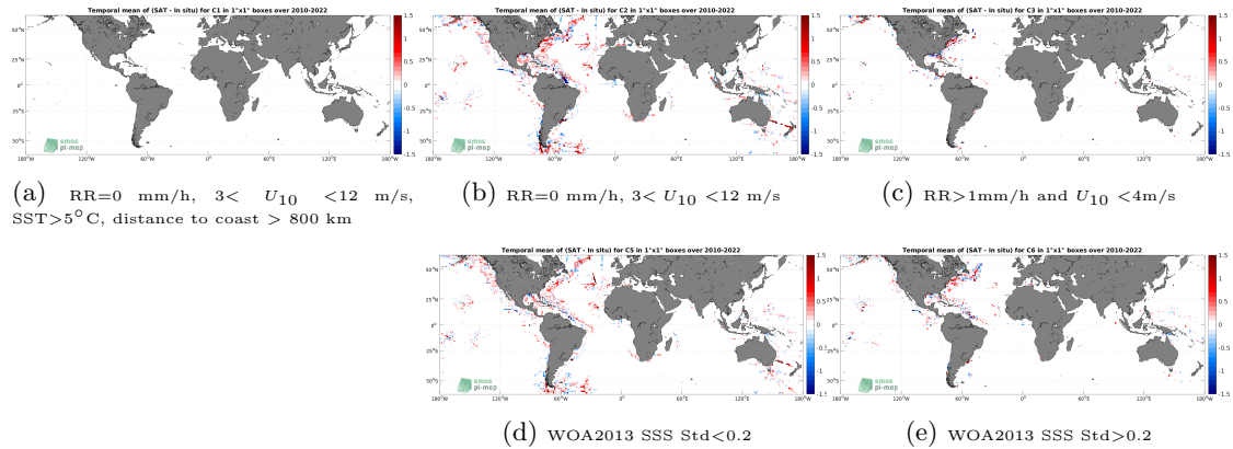
Figure 12: Temporal mean gridded over spatial boxes of size 1^\circ \times 1^\circ of \Delta SSS (SMOS SSS L3 v8 - 9 Days (CATDS-CECOS-LOCEAN) - TSG (SAMOS)) for 5 different subdatasets corresponding to:RR=0 mm/h, 3 < U_{10} < 12 m/s, SST >5^\circ\text{C} , distance to coast > 800 km (a), RR=0 mm/h, 3 < U_{10} < 12 m/s (b), RR >1 mm/h and U_{10} < 4 m/s (c), WOA2013 SSS Std <0.2 (d), WOA2013 SSS Std >0.2 (e).
