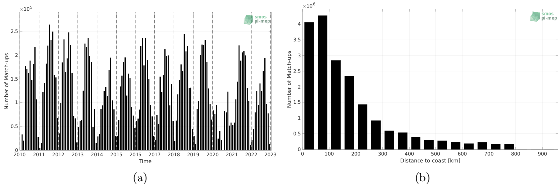
Figure 1: Number of match-ups between TSG (SAMOS) and SMOS SSS L3 v8 - 9 Days (CATDS-CECOS-LOCEAN) SSS as a function of time (a) and as function of the distance to coast (b) over the SMOS coastal zone (<800km) 60N-60S Pi-MEP region and for the full satellite product period.
