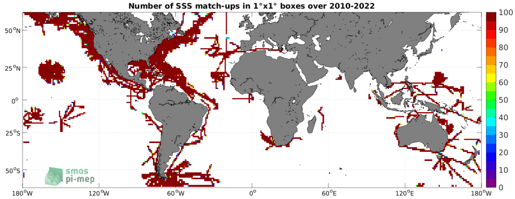
Figure 4: Number of SSS match-ups between TSG (SAMOS) SSS and the SMOS SSS L3 v8 - 9 Days (CATDS-CECOS-LOCEAN) SSS product for the SMOS coastal zone (<800km) 60N-60S Pi-MEP region over 1^\circ \times 1^\circ boxes and for the full satellite product period.
