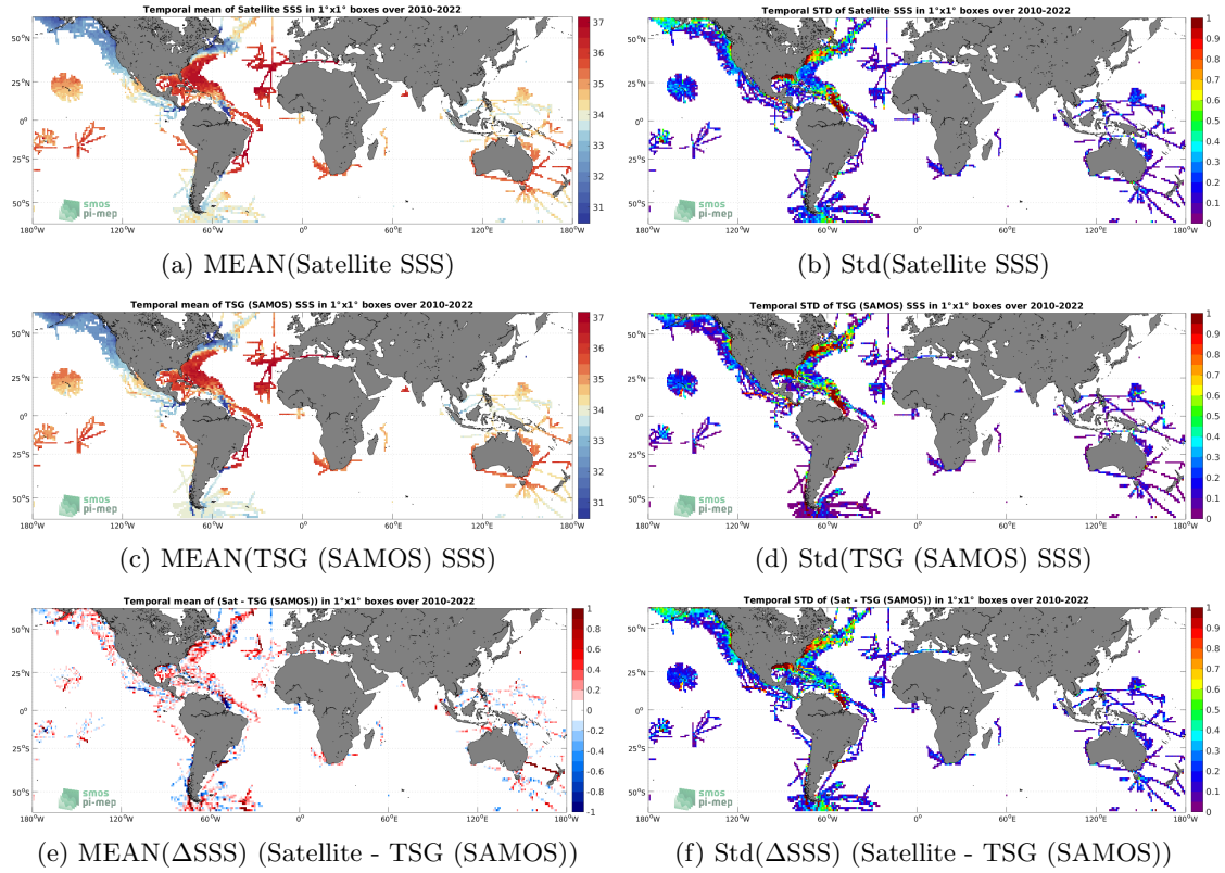
Figure 6: Temporal mean (left) and Std (right) of SSS from SMOS SSS L3 v8 - 9 Days (CATDS-CECOS-LOCEAN) (top), TSG (SAMOS) (middle), and of \Delta SSS (Satellite - TSG (SAMOS)). Only match-up pairs are used to generate these maps.
