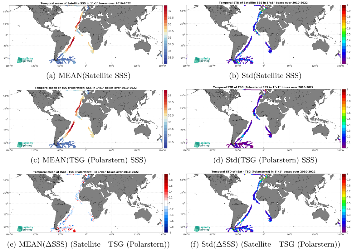
Figure 6: Temporal mean (left) and Std (right) of SSS from SMOS SSS L3 v8 - 9 Days (CATDS-CEC-LOCEAN) (top), TSG (Polarstern) (middle), and of \Delta SSS (Satellite - TSG (Polarstern)). Only match-up pairs are used to generate these maps.
