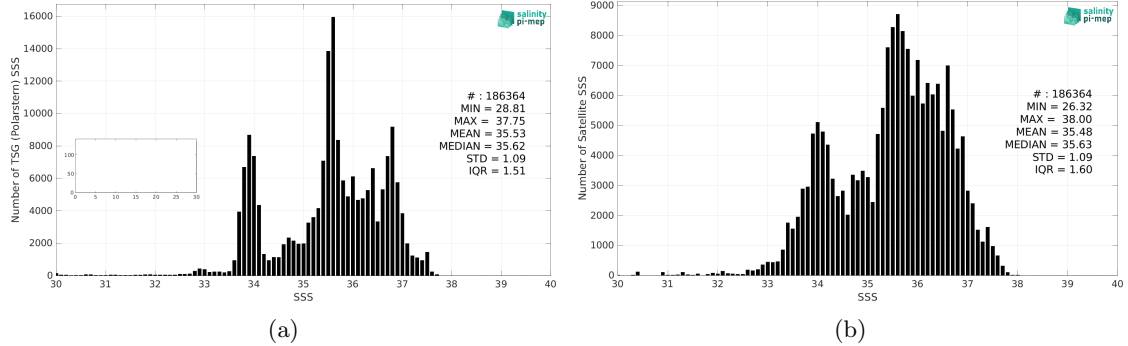
Figure 2: Histograms of SSS from TSG (Polarstern) (a) and SMOS SSS L3 v8 - 9 Days (CATDS-CEC-LOCEAN) (b) considering all match-up pairs per bins of 0.1 over the SMOS coastal zone (<800km) 60N-60S Pi-MEP region and for the full satellite product period.
