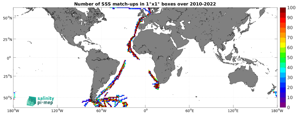
Figure 4: Number of SSS match-ups between TSG (Polarstern) SSS and the SMOS SSS L3 v8 - 9 Days (CATDS-CEC-LOCEAN) SSS product for the SMOS coastal zone (<800km) 60N-60S Pi-MEP region over 1^\circ \times 1^\circ boxes and for the full satellite product period.
