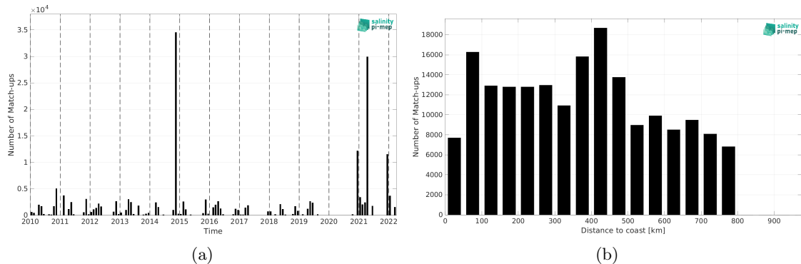
Figure 1: Number of match-ups between TSG (Polarstern) and SMOS SSS L3 v8 - 9 Days (CATDS-CEC-LOCEAN) SSS as a function of time (a) and as function of the distance to coast (b) over the SMOS coastal zone (<800km) 60N-60S Pi-MEP region and for the full satellite product period.
