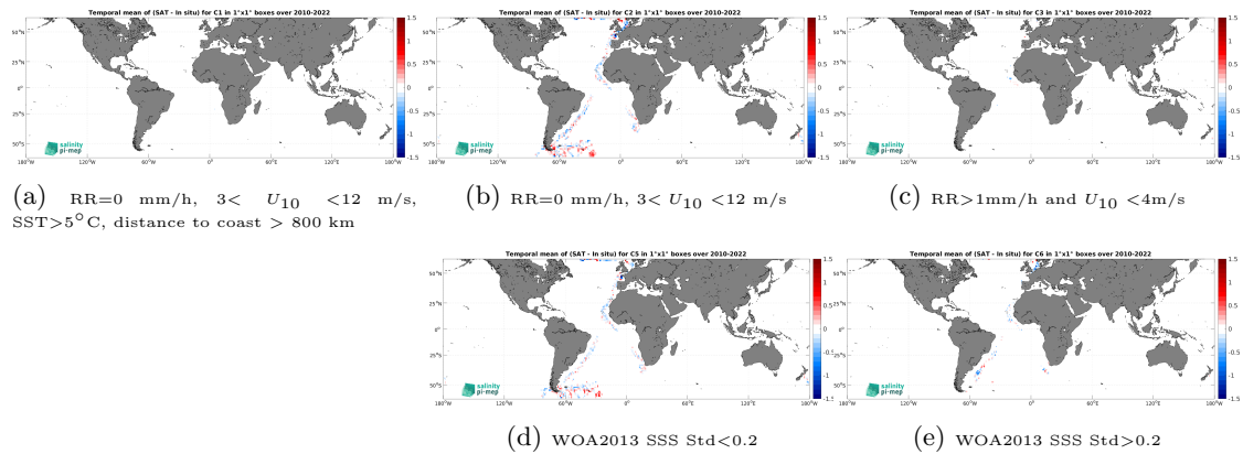
Figure 12: Temporal mean gridded over spatial boxes of size 1^\circ \times 1^\circ of \Delta\text{SSS} (SMOS SSS L3 v8 - 9 Days (CATDS-CEC-LOCEAN) - TSG (Polarstern)) for 5 different subdatasets corresponding to:RR=0 mm/h, 3 < U_{10} < 12 m/s, SST >5^\circ\text{C} , distance to coast > 800 km (a), RR=0 mm/h, 3 < U_{10} < 12 m/s (b), RR >1 mm/h and U_{10} < 4 m/s (c), WOA2013 SSS Std <0.2 (d), WOA2013 SSS Std >0.2 (e).
