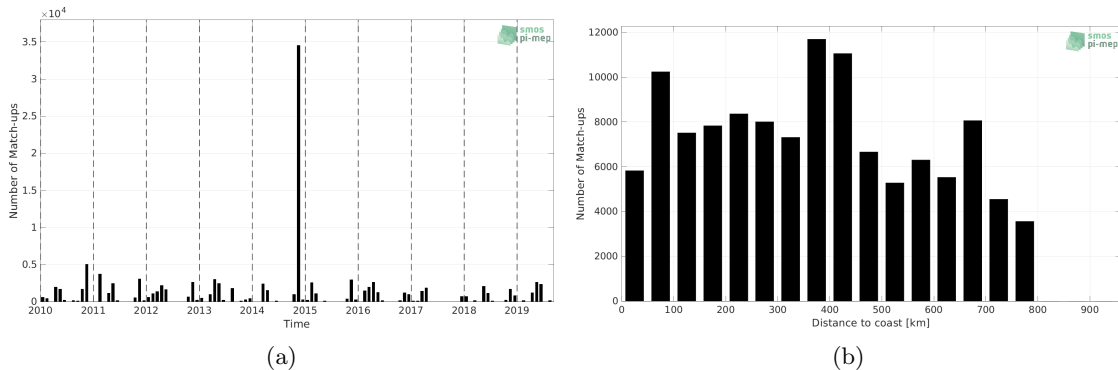
Figure 1: Number of match-ups between TSG (Polarstern) and SMOS SSS L3 v8 - 9 Days (CATDS-CECOS-LOCEAN) SSS as a function of time (a) and as function of the distance to coast (b) over the SMOS coastal zone (<800km) 60N-60S Pi-MEP region and for the full satellite product period.
