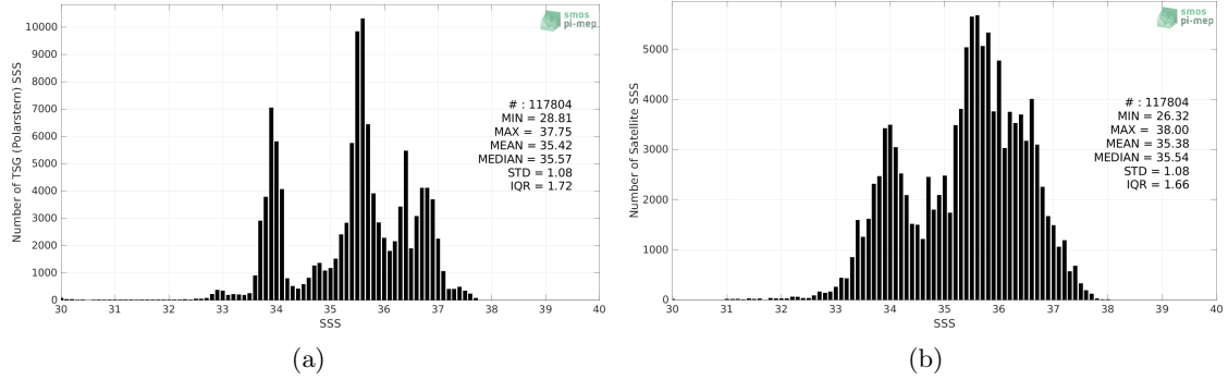
Figure 2: Histograms of SSS from TSG (Polarstern) (a) and SMOS SSS L3 v8 - 9 Days (CATDS-CECOS-LOCEAN) (b) considering all match-up pairs per bins of 0.1 over the SMOS coastal zone (<800km) 60N-60S Pi-MEP region and for the full satellite product period.
