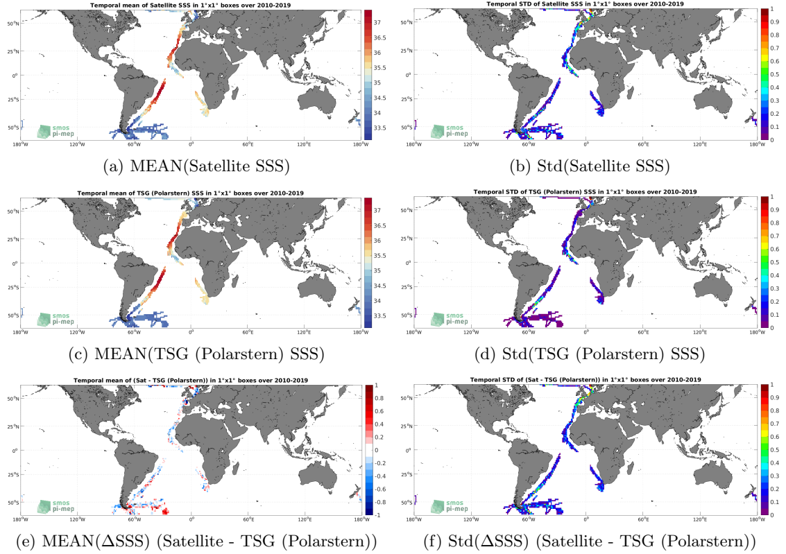
Figure 6: Temporal mean (left) and Std (right) of SSS from SMOS SSS L3 v8 - 9 Days (CATDS-CECOS-LOCEAN) (top), TSG (Polarstern) (middle), and of \Delta SSS (Satellite - TSG (Polarstern)). Only match-up pairs are used to generate these maps.
