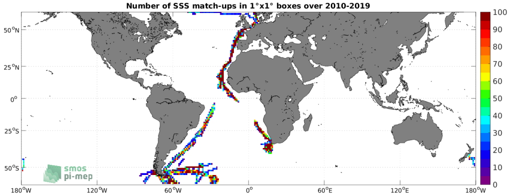
Figure 4: Number of SSS match-ups between TSG (Polarstern) SSS and the SMOS SSS L3 v8 - 9 Days (CATDS-CECOS-LOCEAN) SSS product for the SMOS coastal zone (<800km) 60N-60S Pi-MEP region over 1^\circ \times 1^\circ boxes and for the full satellite product period.
