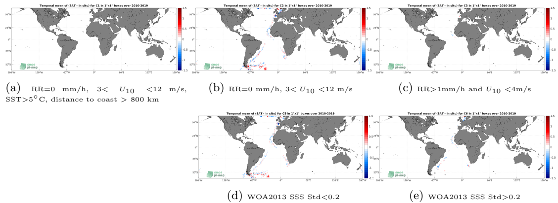
Figure 12: Temporal mean gridded over spatial boxes of size 1^\circ \times 1^\circ of \Delta\text{SSS} (SMOS SSS L3 v8 - 9 Days (CATDS-CECOS-LOCEAN) - TSG (Polarstern)) for 5 different subdatasets corresponding to:RR=0 mm/h, 3 < U_{10} < 12 m/s, SST >5^\circ\text{C} , distance to coast > 800 km (a), RR=0 mm/h, 3 < U_{10} < 12 m/s (b), RR >1 mm/h and U_{10} < 4 m/s (c), WOA2013 SSS Std <0.2 (d), WOA2013 SSS Std >0.2 (e).
