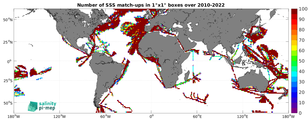
Figure 4: Number of SSS match-ups between TSG (LEGOS-DM) SSS and the SMOS SSS L3 v8 - 9 Days (CATDS-CEC-LOCEAN) SSS product for the SMOS coastal zone (<800km) 60N-60S Pi-MEP region over 1^\circ \times 1^\circ boxes and for the full satellite product period.
