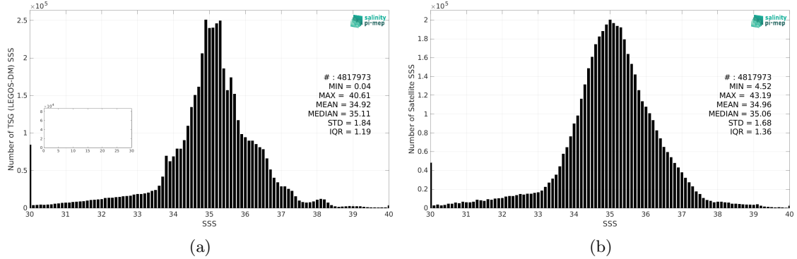
Figure 2: Histograms of SSS from TSG (LEGOS-DM) (a) and SMOS SSS L3 v8 - 9 Days (CATDS-CEC-LOCEAN) (b) considering all match-up pairs per bins of 0.1 over the SMOS coastal zone (<800km) 60N-60S Pi-MEP region and for the full satellite product period.
