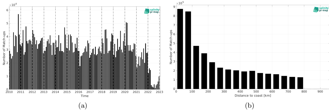
Figure 1: Number of match-ups between TSG (LEGOS-DM) and SMOS SSS L3 v8 - 9 Days (CATDS-CEC-LOCEAN) SSS as a function of time (a) and as function of the distance to coast (b) over the SMOS coastal zone (<800km) 60N-60S Pi-MEP region and for the full satellite product period.
