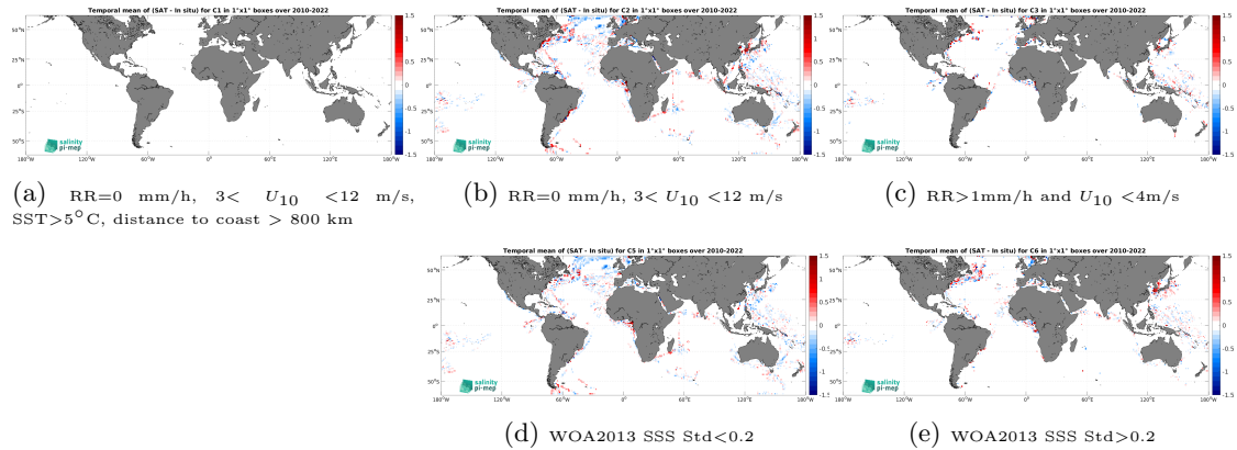
Figure 12: Temporal mean gridded over spatial boxes of size 1^\circ \times 1^\circ of \Delta SSS (SMOS SSS L3 v8 - 9 Days (CATDS-CEC-LOCEAN) - TSG (LEGOS-DM)) for 5 different subdatasets corresponding to:RR=0 mm/h, 3 < U_{10} < 12 m/s, SST >5^\circ\text{C} , distance to coast > 800 km (a), RR=0 mm/h, 3 < U_{10} < 12 m/s (b), RR >1 mm/h and U_{10} < 4 m/s (c), WOA2013 SSS Std <0.2 (d), WOA2013 SSS Std >0.2 (e).
