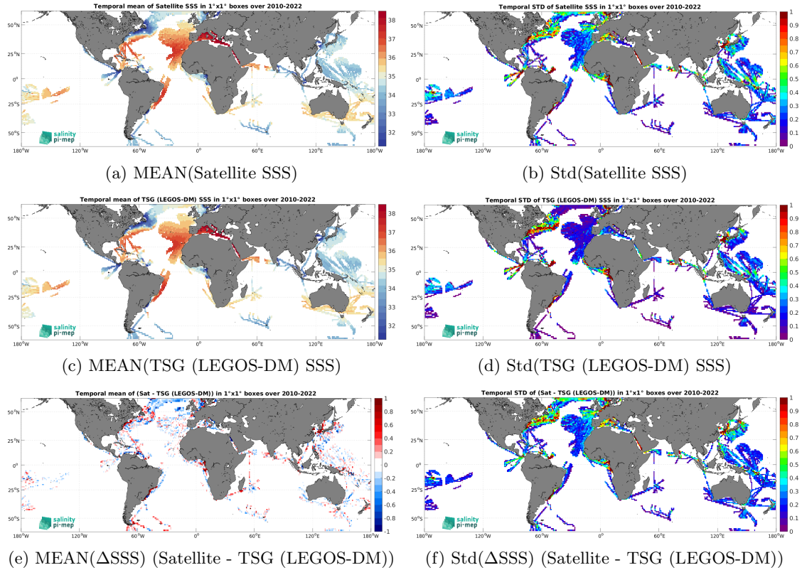
Figure 6: Temporal mean (left) and Std (right) of SSS from SMOS SSS L3 v8 - 9 Days (CATDS-CEC-LOCEAN) (top), TSG (LEGOS-DM) (middle), and of \Delta SSS (Satellite - TSG (LEGOS-DM)). Only match-up pairs are used to generate these maps.
