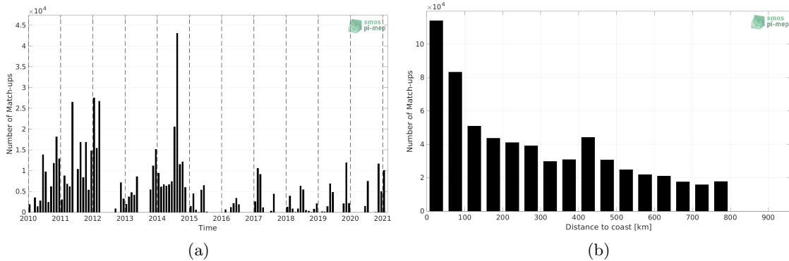
Figure 1: Number of match-ups between TSG (GOSUD-Sailing-ship) and SMOS SSS L3 v8 - 9 Days (CATDS-CECOS-LOCEAN) SSS as a function of time (a) and as function of the distance to coast (b) over the SMOS coastal zone (<800km) 60N-60S Pi-MEP region and for the full satellite product period.
