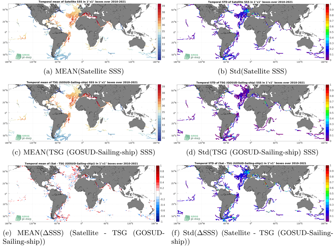
Figure 6: Temporal mean (left) and Std (right) of SSS from SMOS SSS L3 v8 - 9 Days (CATDS-CECOS-LOCEAN) (top), TSG (GOSUD-Sailing-ship) (middle), and of \Delta\text{SSS} (Satellite - TSG (GOSUD-Sailing-ship)). Only match-up pairs are used to generate these maps.
