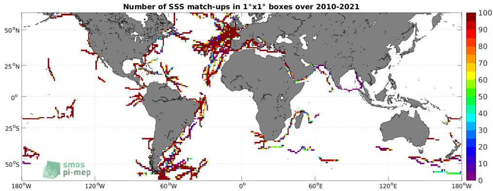
Figure 4: Number of SSS match-ups between TSG (GOSUD-Sailing-ship) SSS and the SMOS SSS L3 v8 - 9 Days (CATDS-CECOS-LOCEAN) SSS product for the SMOS coastal zone ( <800\text{km} ) 60N-60S Pi-MEP region over 1^\circ \times 1^\circ boxes and for the full satellite product period.
