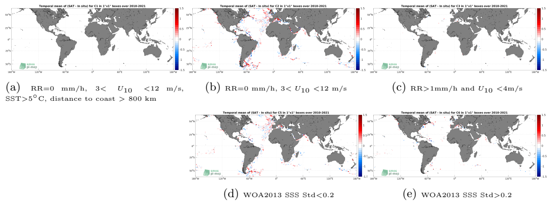
Figure 12: Temporal mean gridded over spatial boxes of size 1^\circ \times 1^\circ of \Delta SSS (SMOS SSS L3 v8 - 9 Days (CATDS-CECOS-LOCEAN) - TSG (GOSUD-Sailing-ship)) for 5 different subdatasets corresponding to:RR=0 mm/h, 3 < U_{10} < 12 m/s, SST >5^\circ C, distance to coast > 800 km (a), RR=0 mm/h, 3 < U_{10} < 12 m/s (b), RR >1 mm/h and U_{10} < 4 m/s (c), WOA2013 SSS Std <0.2 (d), WOA2013 SSS Std >0.2 (e).
