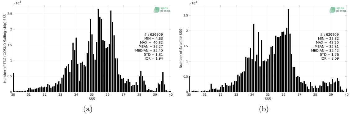
Figure 2: Histograms of SSS from TSG (GOSUD-Sailing-ship) (a) and SMOS SSS L3 v8 - 9 Days (CATDS-CECOS-LOCEAN) (b) considering all match-up pairs per bins of 0.1 over the SMOS coastal zone (<800km) 60N-60S Pi-MEP region and for the full satellite product period.
