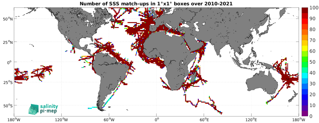
Figure 4: Number of SSS match-ups between TSG (GOSUD-Research-vessel) SSS and the SMOS SSS L3 v8 - 9 Days (CATDS-CEC-LOCEAN) SSS product for the SMOS coastal zone ( <800\text{km} ) 60N-60S Pi-MEP region over 1^\circ \times 1^\circ boxes and for the full satellite product period.
