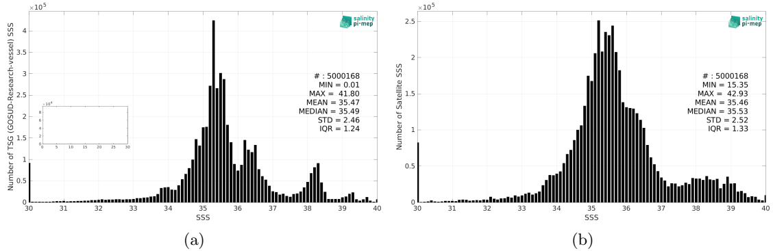
Figure 2: Histograms of SSS from TSG (GOSUD-Research-vessel) (a) and SMOS SSS L3 v8 - 9 Days (CATDS-CEC-LOCEAN) (b) considering all match-up pairs per bins of 0.1 over the SMOS coastal zone (<800km) 60N-60S Pi-MEP region and for the full satellite product period.
