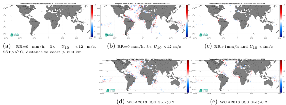
Figure 12: Temporal mean gridded over spatial boxes of size 1^\circ \times 1^\circ of \Delta\text{SSS} (SMOS SSS L3 v8 - 9 Days (CATDS-CEC-LOCEAN) - TSG (GOSUD-Research-vessel)) for 5 different subdatasets corresponding to: RR=0 mm/h, 3 < U_{10} < 12 m/s, SST > 5^\circ\text{C} , distance to coast > 800 km (a), RR=0 mm/h, 3 < U_{10} < 12 m/s (b), RR > 1 mm/h and U_{10} < 4 m/s (c), WOA2013 SSS Std < 0.2 (d), WOA2013 SSS Std > 0.2 (e).
