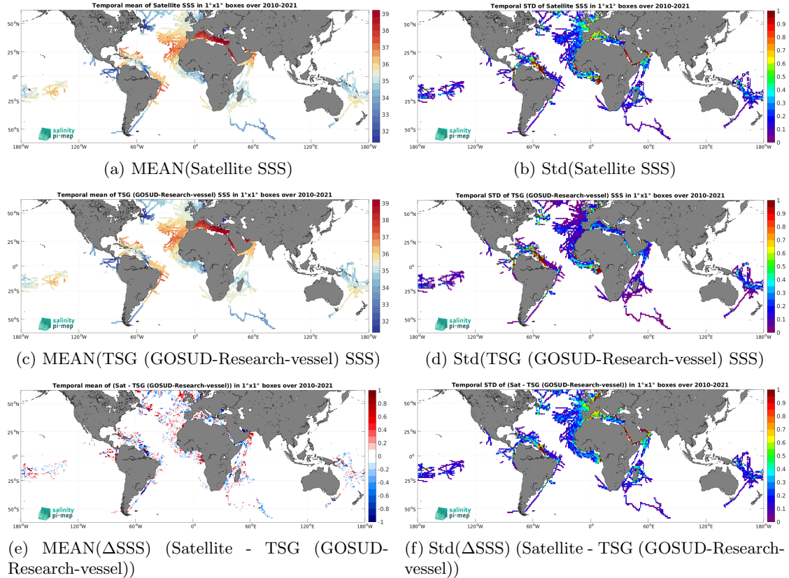
Figure 6: Temporal mean (left) and Std (right) of SSS from SMOS SSS L3 v8 - 9 Days (CATDS-CEC-LOCEAN) (top), TSG (GOSUD-Research-vessel) (middle), and of \Delta\text{SSS} (Satellite - TSG (GOSUD-Research-vessel)). Only match-up pairs are used to generate these maps.
