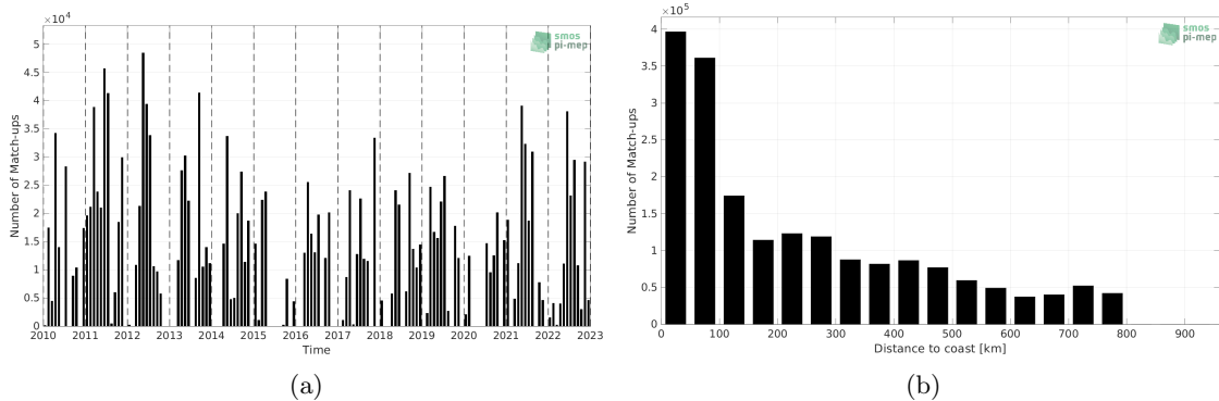
Figure 1: Number of match-ups between TSG (CSIC-UTM) and SMOS SSS L3 v8 - 9 Days (CATDS-CECOS-LOCEAN) SSS as a function of time (a) and as function of the distance to coast (b) over the SMOS coastal zone (<800km) 60N-60S Pi-MEP region and for the full satellite product period.
