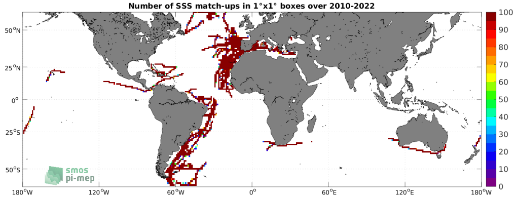
Figure 4: Number of SSS match-ups between TSG (CSIC-UTM) SSS and the SMOS SSS L3 v8 - 9 Days (CATDS-CECOS-LOCEAN) SSS product for the SMOS coastal zone (<800km) 60N-60S Pi-MEP region over 1^\circ \times 1^\circ boxes and for the full satellite product period.
