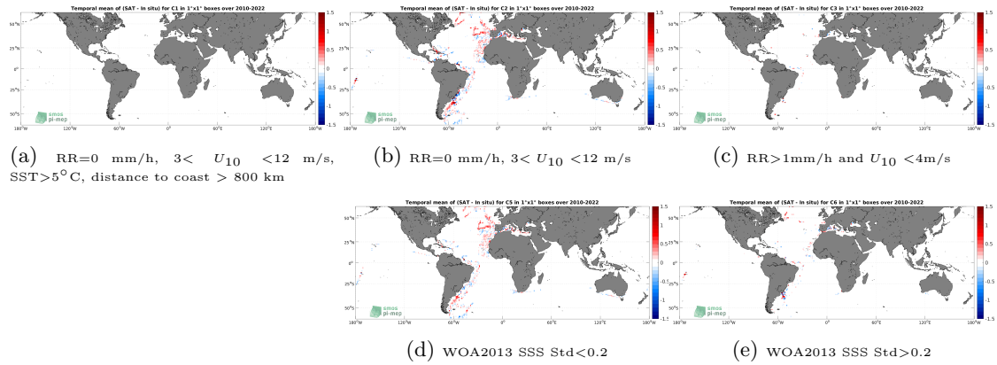
Figure 12: Temporal mean gridded over spatial boxes of size 1^\circ \times 1^\circ of \Delta\text{SSS} (SMOS SSS L3 v8 - 9 Days (CATDS-CECOS-LOCEAN) - TSG (CSIC-UTM)) for 5 different subdatasets corresponding to:RR=0 mm/h, 3 < U_{10} < 12 m/s, SST >5^\circ\text{C} , distance to coast > 800 km (a), RR=0 mm/h, 3 < U_{10} < 12 m/s (b), RR >1 mm/h and U_{10} < 4 m/s (c), WOA2013 SSS Std <0.2 (d), WOA2013 SSS Std >0.2 (e).
