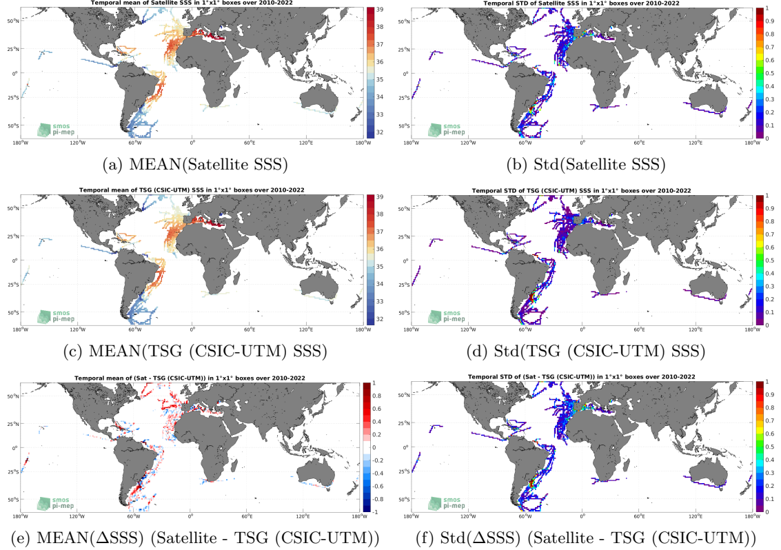
Figure 6: Temporal mean (left) and Std (right) of SSS from SMOS SSS L3 v8 - 9 Days (CATDS-CECOS-LOCEAN) (top), TSG (CSIC-UTM) (middle), and of \Delta\text{SSS} (Satellite - TSG (CSIC-UTM)). Only match-up pairs are used to generate these maps.
