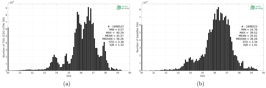
Figure 2: Histograms of SSS from TSG (CSIC-UTM) (a) and SMOS SSS L3 v8 - 9 Days (CATDS-CECOS-LOCEAN) (b) considering all match-up pairs per bins of 0.1 over the SMOS coastal zone (<800km) 60N-60S Pi-MEP region and for the full satellite product period.
