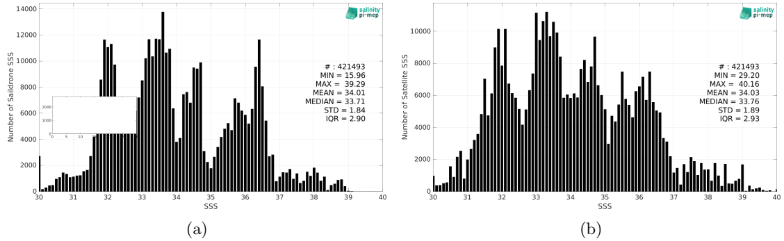
Figure 2: Histograms of SSS from Sairdrone (a) and SMOS SSS L3 v8 - 9 Days (CATDS-CEC-LOCEAN) (b) considering all match-up pairs per bins of 0.1 over the SMOS coastal zone (<800km) 60N-60S Pi-MEP region and for the full satellite product period.
