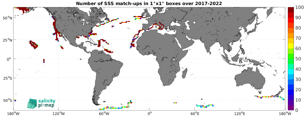
Figure 4: Number of SSS match-ups between Sairdrone SSS and the SMOS SSS L3 v8 - 9 Days (CATDS-CEC-LOCEAN) SSS product for the SMOS coastal zone (<800km) 60N-60S Pi-MEP region over 1^\circ \times 1^\circ boxes and for the full satellite product period.
