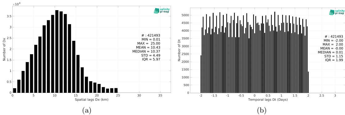
Figure 5: Histograms of the spatial (a) and temporal (b) lags between the location/time of the Sairdrone measurement and the date of the corresponding SMOS SSS L3 v8 - 9 Days (CATDS-CEC-LOCEAN) SSS pixel.
