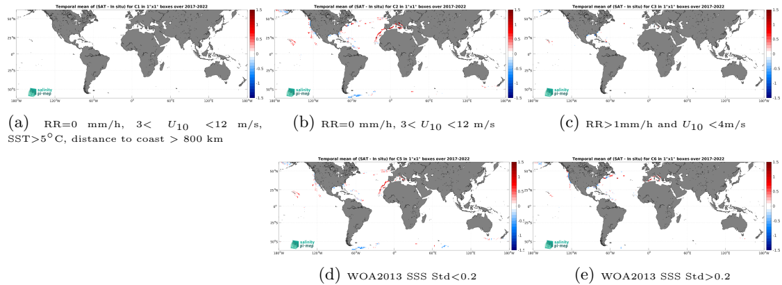
Figure 12: Temporal mean gridded over spatial boxes of size 1^\circ \times 1^\circ of \Delta SSS (SMOS SSS L3 v8 - 9 Days (CATDS-CEC-LOCEAN) - Saildrone) for 5 different subdatasets corresponding to:RR=0 mm/h, 3 < U_{10} < 12 m/s, SST >5^\circ\text{C} , distance to coast > 800 km (a), RR=0 mm/h, 3 < U_{10} < 12 m/s (b), RR >1 mm/h and U_{10} < 4 m/s (c), WOA2013 SSS Std <0.2 (d), WOA2013 SSS Std >0.2 (e).
