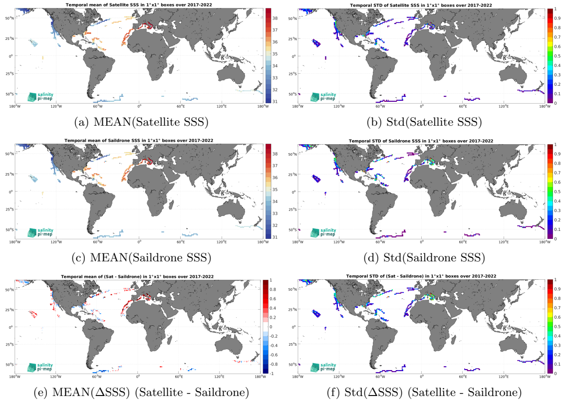
Figure 6: Temporal mean (left) and Std (right) of SSS from SMOS SSS L3 v8 - 9 Days (CATDS-CEC-LOCEAN) (top), Saildrone (middle), and of \Delta SSS (Satellite - Saildrone). Only match-up pairs are used to generate these maps.
