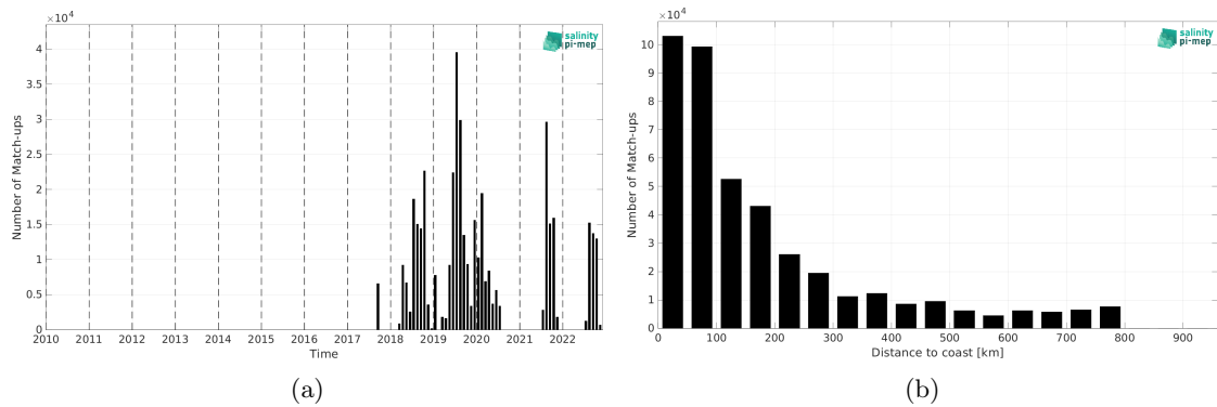
Figure 1: Number of match-ups between Saildrone and SMOS SSS L3 v8 - 9 Days (CATDS-CEC-LOCEAN) SSS as a function of time (a) and as function of the distance to coast (b) over the SMOS coastal zone (<800km) 60N-60S Pi-MEP region and for the full satellite product period.
