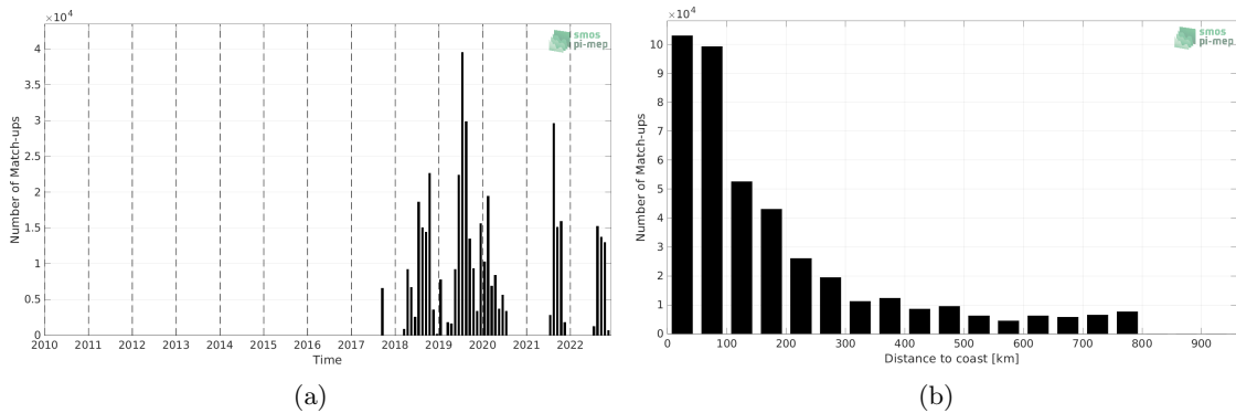
Figure 1: Number of match-ups between Saildrone and SMOS SSS L3 v8 - 9 Days (CATDS-CECOS-LOCEAN) SSS as a function of time (a) and as function of the distance to coast (b) over the SMOS coastal zone (<800km) 60N-60S Pi-MEP region and for the full satellite product period.
