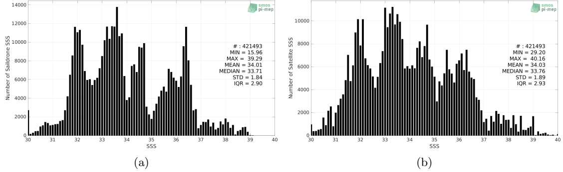
Figure 2: Histograms of SSS from Sairdrone (a) and SMOS SSS L3 v8 - 9 Days (CATDS-CECOS-LOCEAN) (b) considering all match-up pairs per bins of 0.1 over the SMOS coastal zone (<800km) 60N-60S Pi-MEP region and for the full satellite product period.
