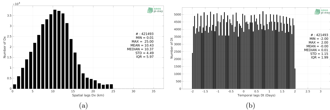
Figure 5: Histograms of the spatial (a) and temporal (b) lags between the location/time of the Sairdrone measurement and the date of the corresponding SMOS SSS L3 v8 - 9 Days (CATDS-CECOS-LOCEAN) SSS pixel.
