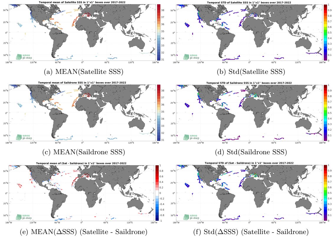
Figure 6: Temporal mean (left) and Std (right) of SSS from SMOS SSS L3 v8 - 9 Days (CATDS-CECOS-LOCEAN) (top), Saildrone (middle), and of \Delta SSS (Satellite - Saildrone). Only match-up pairs are used to generate these maps.
