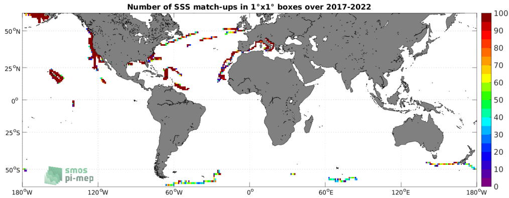
Figure 4: Number of SSS match-ups between Sairdrone SSS and the SMOS SSS L3 v8 - 9 Days (CATDS-CECOS-LOCEAN) SSS product for the SMOS coastal zone (<800km) 60N-60S Pi-MEP region over 1^\circ \times 1^\circ boxes and for the full satellite product period.
