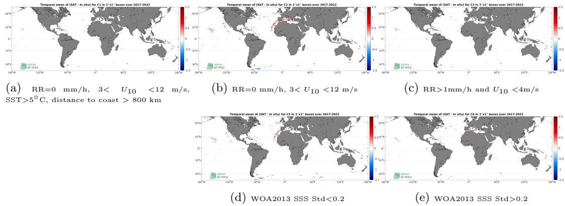
Figure 12: Temporal mean gridded over spatial boxes of size 1^\circ \times 1^\circ of \Delta\text{SSS} (SMOS SSS L3 v8 - 9 Days (CATDS-CECOS-LOCEAN) - Saildrone) for 5 different subdatasets corresponding to:RR=0 mm/h, 3 < U_{10} < 12 m/s, SST >5^\circ\text{C} , distance to coast > 800 km (a), RR=0 mm/h, 3 < U_{10} < 12 m/s (b), RR >1 mm/h and U_{10} < 4 m/s (c), WOA2013 SSS Std <0.2 (d), WOA2013 SSS Std >0.2 (e).
