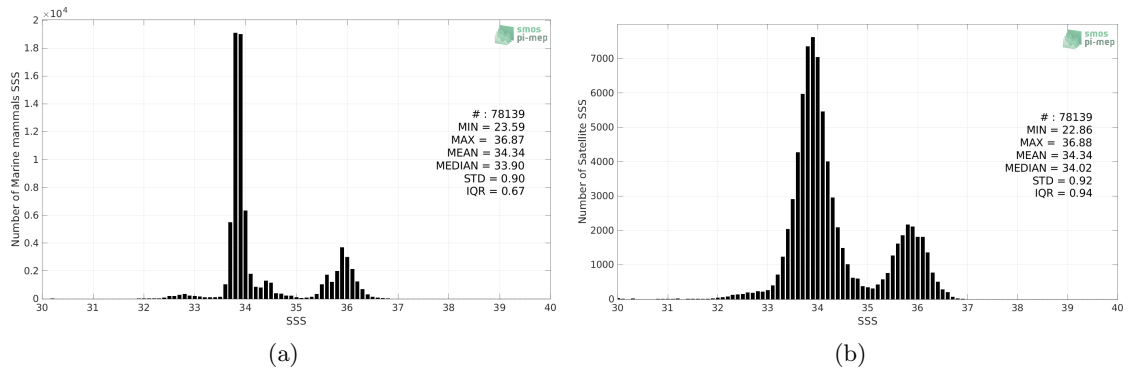
Figure 2: Histograms of SSS from Marine mammals (a) and SMOS SSS L3 v8 - 9 Days (CATDS-CECOS-LOCEAN) (b) considering all match-up pairs per bins of 0.1 over the SMOS coastal zone (<800km) 60N-60S Pi-MEP region and for the full satellite product period.
