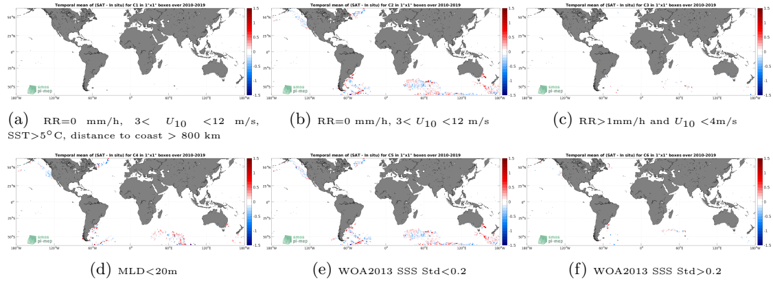
Figure 12: Temporal mean gridded over spatial boxes of size 1^{\circ}\times 1^{\circ} of \Delta\text{SSS} (SMOS SSS L3 v8 - 9 Days (CATDS-CECOS-LOCEAN) - Marine mammals) for 6 different subdatasets corresponding to:RR=0 mm/h, 3 < U_{10} < 12 m/s, SST > 5^{\circ}\text{C} , distance to coast > 800 km (a), RR=0 mm/h, 3 < U_{10} < 12 m/s (b), RR > 1\text{mm/h} and U_{10} < 4\text{m/s} (c),MLD < 20\text{m} (d),WOA2013 SSS Std < 0.2 (e),WOA2013 SSS Std > 0.2 (f).
