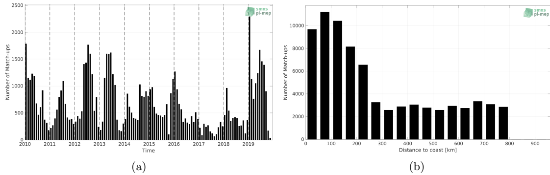
Figure 1: Number of match-ups between Marine mammals and SMOS SSS L3 v8 - 9 Days (CATDS-CECOS-LOCEAN) SSS as a function of time (a) and as function of the distance to coast (b) over the SMOS coastal zone (<800km) 60N-60S Pi-MEP region and for the full satellite product period.
