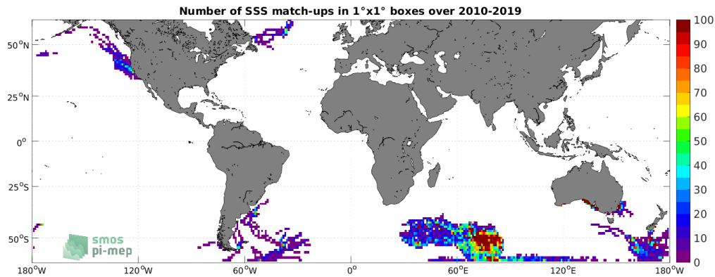
Figure 4: Number of SSS match-ups between Marine mammals SSS and the SMOS SSS L3 v8 - 9 Days (CATDS-CECOS-LOCEAN) SSS product for the SMOS coastal zone (<800km) 60N-60S Pi-MEP region over 1^\circ \times 1^\circ boxes and for the full satellite product period.
