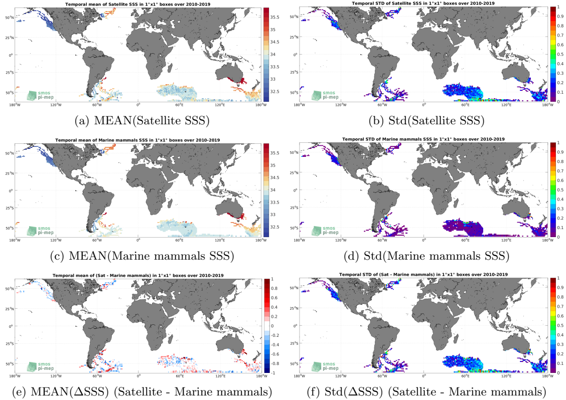
Figure 6: Temporal mean (left) and Std (right) of SSS from SMOS SSS L3 v8 - 9 Days (CATDS-CECOS-LOCEAN) (top), Marine mammals (middle), and of \Delta SSS (Satellite - Marine mammals). Only match-up pairs are used to generate these maps.
