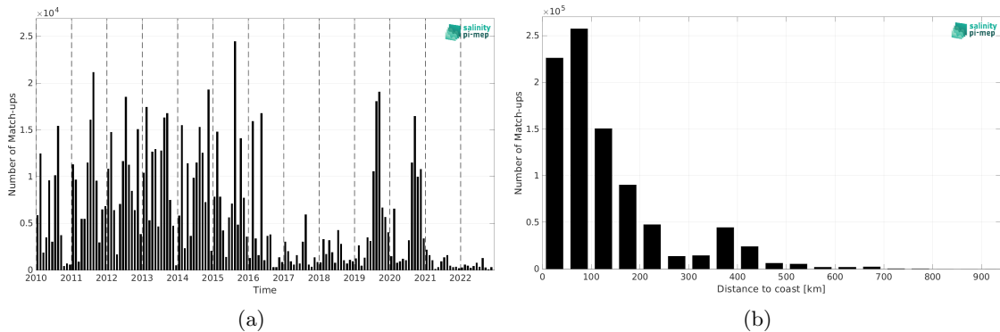
Figure 1: Number of match-ups between ICES and SMOS SSS L3 v8 - 9 Days (CATDS-CEC-LOCEAN) SSS as a function of time (a) and as function of the distance to coast (b) over the SMOS coastal zone (<800km) 60N-60S Pi-MEP region and for the full satellite product period.
