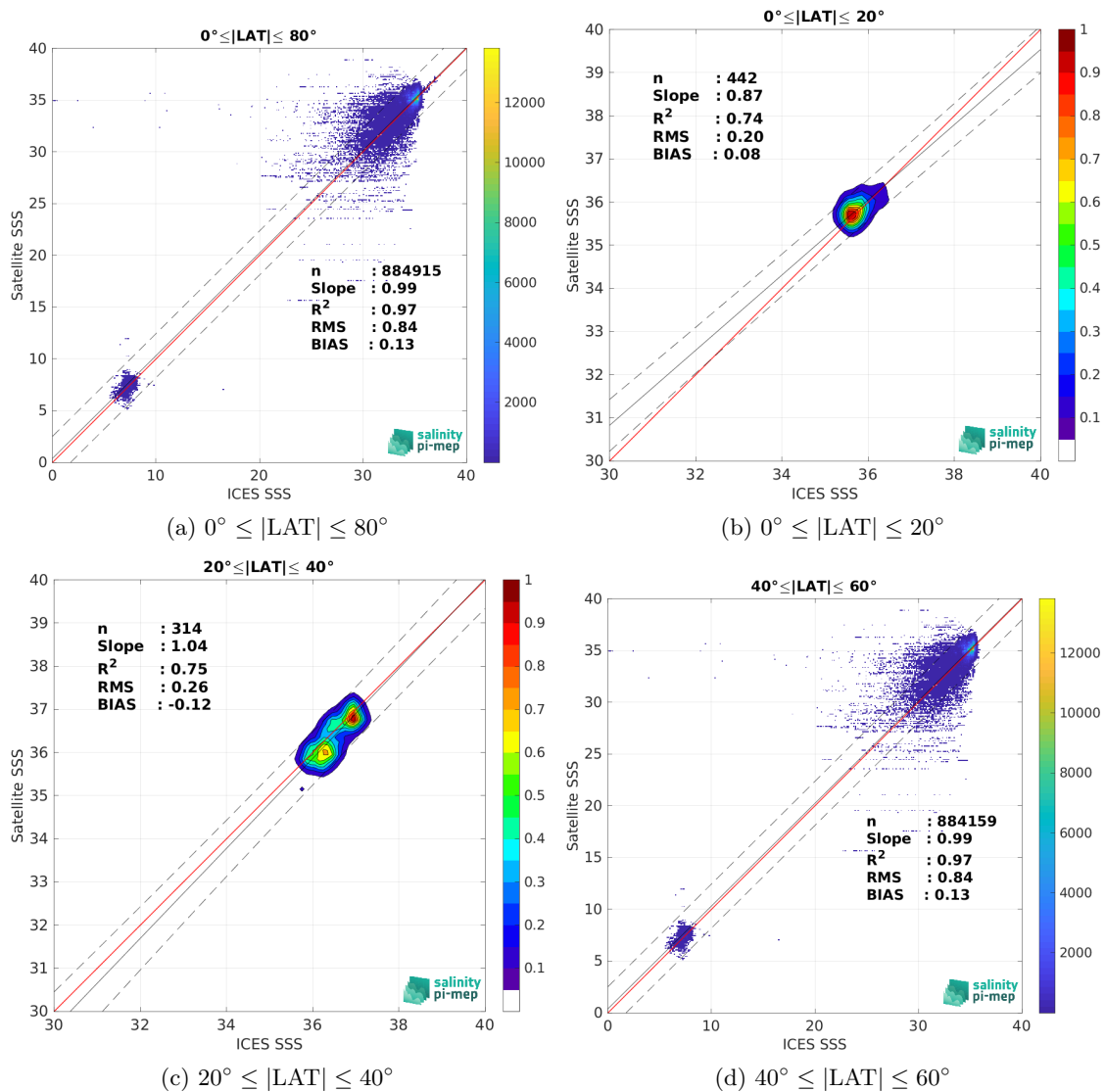
Figure 9: Contour maps of the concentration of SMOS SSS L3 v8 - 9 Days (CATDS-CEC-LOCEAN) SSS (y-axis) versus ICES SSS (x-axis) at match-up pairs for different latitude bands. For each plot, the red line shows x=y . The black thin and dashed lines indicate a linear fit through the data cloud and the \pm 95\% confidence levels, respectively. The number match-up pairs n , the slope and R^2 coefficient of the linear fit, the root mean square (RMS) and the mean bias between satellite and in situ data are indicated for each latitude band in each plots.
