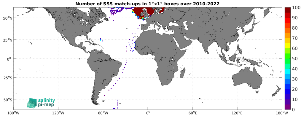
Figure 4: Number of SSS match-ups between ICES SSS and the SMOS SSS L3 v8 - 9 Days (CATDS-CEC-LOCEAN) SSS product for the SMOS coastal zone ( <800\text{km} ) 60N-60S Pi-MEP region over 1^\circ \times 1^\circ boxes and for the full satellite product period.
