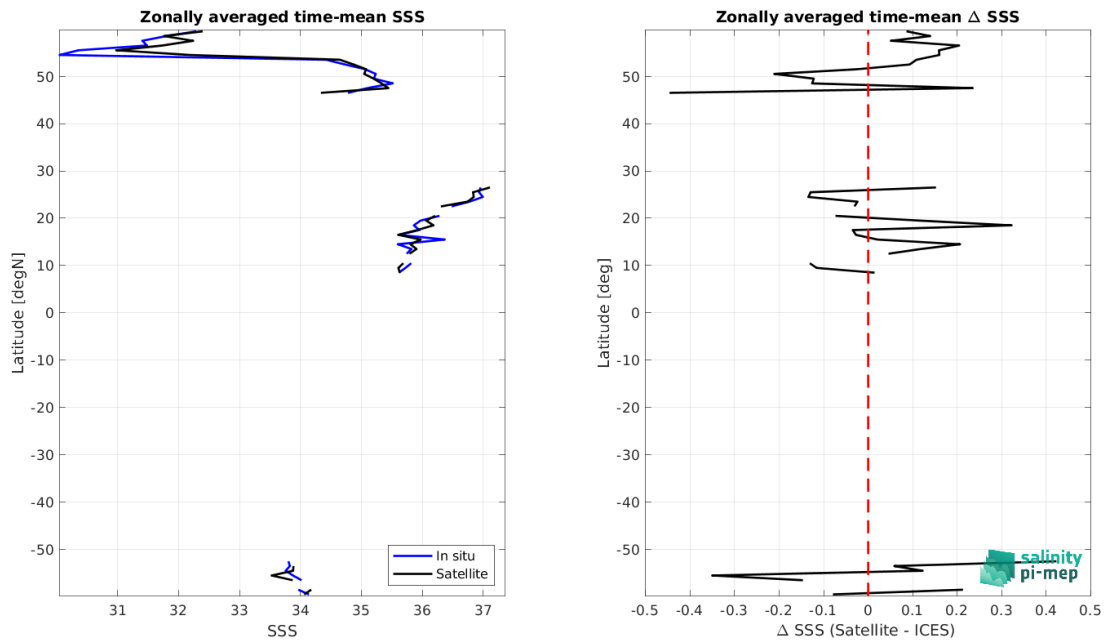
Figure 8: Left panel: Zonal mean SSS from SMOS SSS L3 v8 - 9 Days (CATDS-CEC-LOCEAN) satellite product (black) and from ICES (blue). Right panel: Zonal mean of \Delta SSS (Satellite - ICES) for all the collected Pi-MEP match-up pairs estimated over the full satellite product period.
