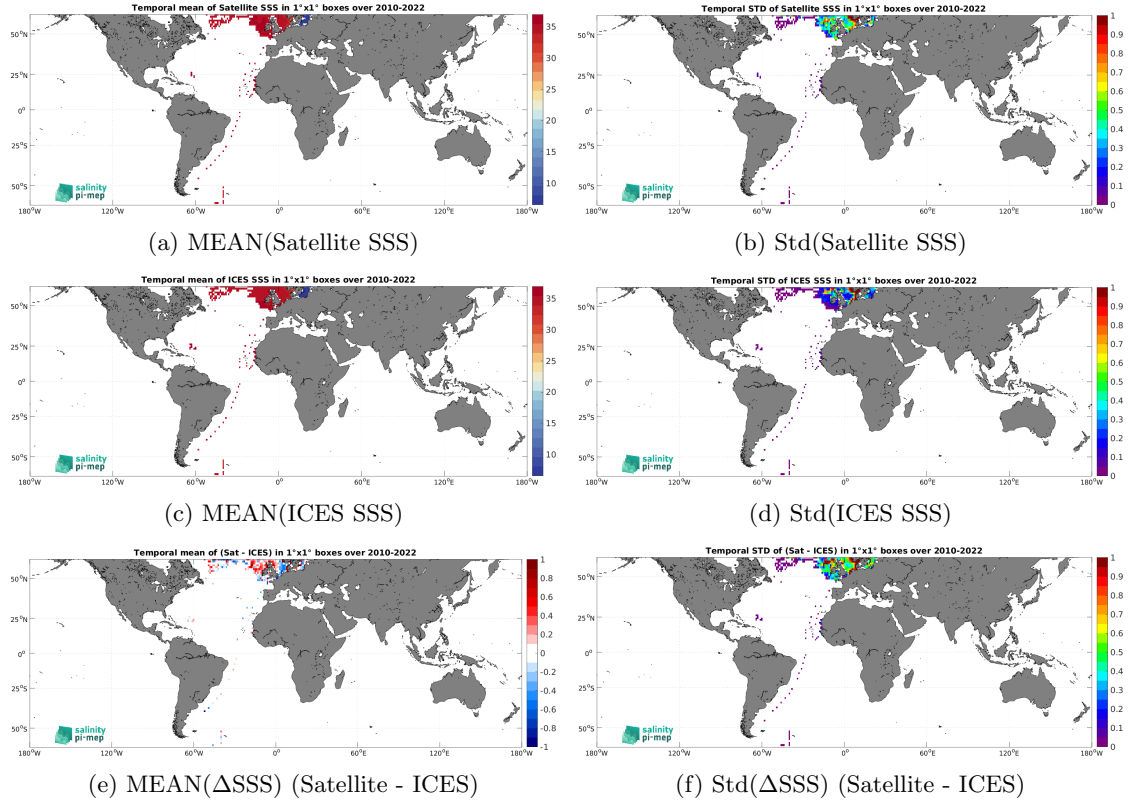
Figure 6: Temporal mean (left) and Std (right) of SSS from SMOS SSS L3 v8 - 9 Days (CATDS-CEC-LOCEAN) (top), ICES (middle), and of \Delta\text{SSS} (Satellite - ICES). Only match-up pairs are used to generate these maps.
