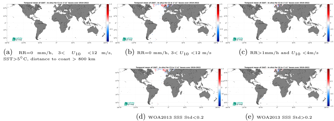
Figure 12: Temporal mean gridded over spatial boxes of size 1^\circ \times 1^\circ of \Delta SSS (SMOS SSS L3 v8 - 9 Days (CATDS-CEC-LOCEAN) - ICES) for 5 different subdatasets corresponding to:RR=0 mm/h, 3 < U_{10} < 12 m/s, SST >5^\circ C, distance to coast > 800 km (a), RR=0 mm/h, 3 < U_{10} < 12 m/s (b), RR >1 mm/h and U_{10} < 4 m/s (c), WOA2013 SSS Std <0.2 (d), WOA2013 SSS Std >0.2 (e).
