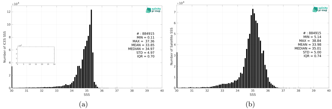
Figure 2: Histograms of SSS from ICES (a) and SMOS SSS L3 v8 - 9 Days (CATDS-CEC-LOCEAN) (b) considering all match-up pairs per bins of 0.1 over the SMOS coastal zone (<800km) 60N-60S Pi-MEP region and for the full satellite product period.
