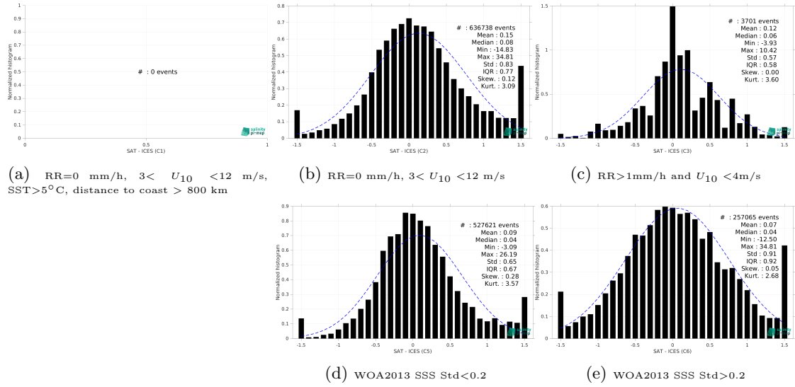
Figure 13: Normalized histogram of \Delta SSS (SMOS SSS L3 v8 - 9 Days (CATDS-CEC-LOCEAN) - ICES) for 5 different subdatasets corresponding to: RR=0 mm/h, 3 < U_{10} < 12 m/s, SST > 5°C, distance to coast > 800 km (a), RR=0 mm/h, 3 < U_{10} < 12 m/s (b), RR > 1mm/h and U_{10} < 4 m/s (c), WOA2013 SSS Std < 0.2 (d), WOA2013 SSS Std > 0.2 (e).
