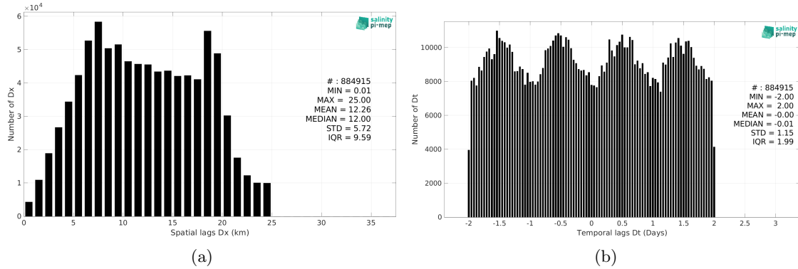
Figure 5: Histograms of the spatial (a) and temporal (b) lags between the location/time of the ICES measurement and the date of the corresponding SMOS SSS L3 v8 - 9 Days (CATDS-CEC-LOCEAN) SSS pixel.
