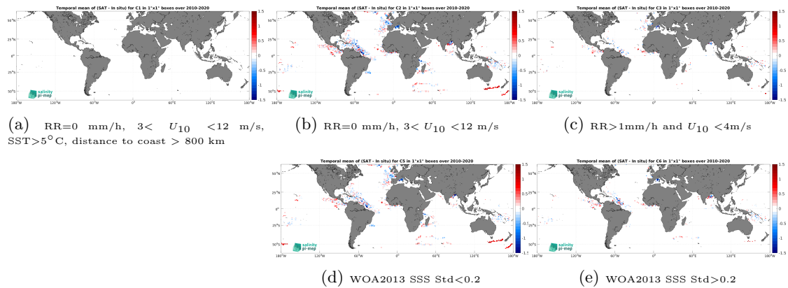
Figure 11: Temporal mean gridded over spatial boxes of size 1^\circ \times 1^\circ of \Delta SSS (SMOS SSS L3 v8 - 9 Days (CATDS-CEC-LOCEAN) - Surface drifters) for 5 different subdatasets corresponding to:RR=0 mm/h, 3 < U_{10} < 12 m/s, SST >5^\circ C, distance to coast > 800 km (a), RR=0 mm/h, 3 < U_{10} < 12 m/s (b), RR >1 mm/h and U_{10} < 4 m/s (c), WOA2013 SSS Std <0.2 (d), WOA2013 SSS Std >0.2 (e).
