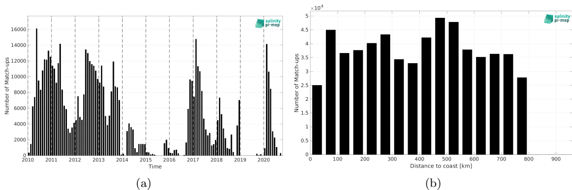
Figure 1: Number of match-ups between Surface drifters and SMOS SSS L3 v8 - 9 Days (CATDS-CEC-LOCEAN) SSS as a function of time (a) and as function of the distance to coast (b) over the SMOS coastal zone (<800km) 60N-60S Pi-MEP region and for the full satellite product period.
