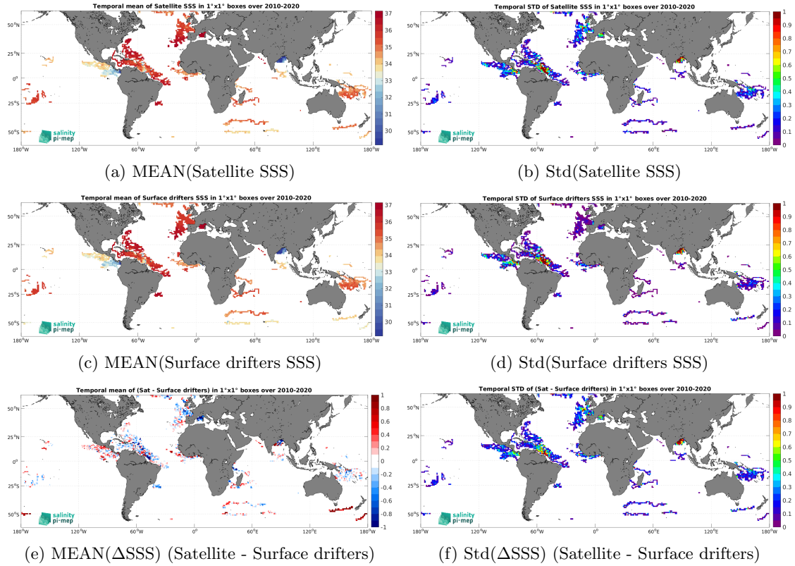
Figure 5: Temporal mean (left) and Std (right) of SSS from SMOS SSS L3 v8 - 9 Days (CATDS-CEC-LOCEAN) (top), Surface drifters (middle), and of \Delta SSS (Satellite - Surface drifters). Only match-up pairs are used to generate these maps.
