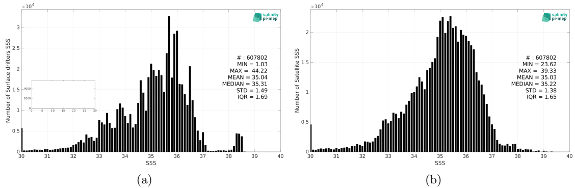
Figure 2: Histograms of SSS from Surface drifters (a) and SMOS SSS L3 v8 - 9 Days (CATDS-CEC-LOCEAN) (b) considering all match-up pairs per bins of 0.1 over the SMOS coastal zone (<800km) 60N-60S Pi-MEP region and for the full satellite product period.
