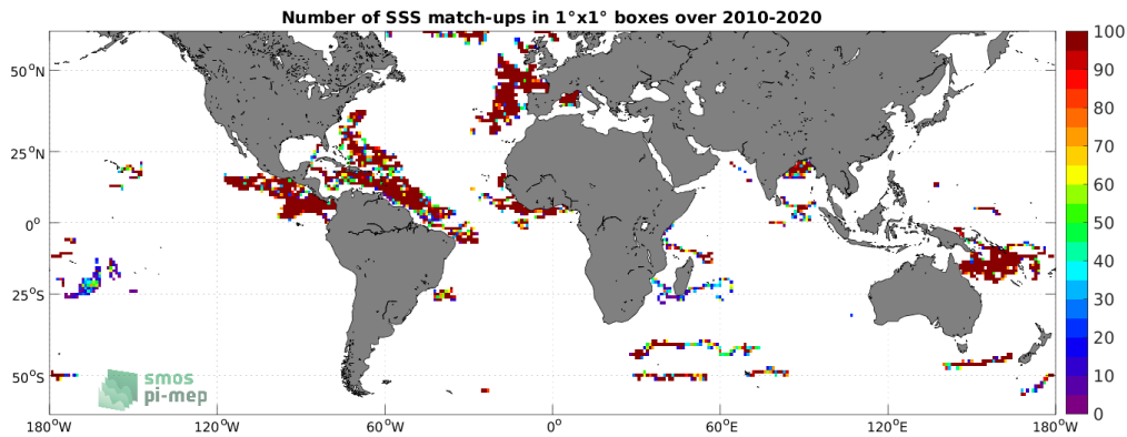
Figure 3: Number of SSS match-ups between Surface drifters SSS and the SMOS SSS L3 v8 - 9 Days (CATDS-CECOS-LOCEAN) SSS product for the SMOS coastal zone (<800km) 60N-60S Pi-MEP region over 1^\circ \times 1^\circ boxes and for the full satellite product period.
