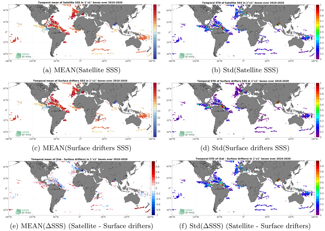
Figure 5: Temporal mean (left) and Std (right) of SSS from SMOS SSS L3 v8 - 9 Days (CATDS-CECOS-LOCEAN) (top), Surface drifters (middle), and of \Delta SSS (Satellite - Surface drifters). Only match-up pairs are used to generate these maps.
