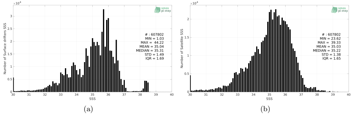
Figure 2: Histograms of SSS from Surface drifters (a) and SMOS SSS L3 v8 - 9 Days (CATDS-CECOS-LOCEAN) (b) considering all match-up pairs per bins of 0.1 over the SMOS coastal zone (<800km) 60N-60S Pi-MEP region and for the full satellite product period.
