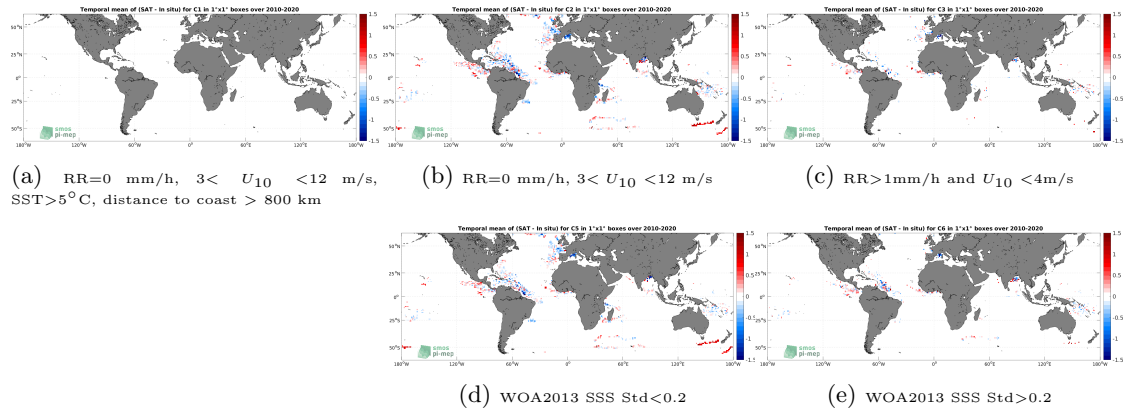
Figure 11: Temporal mean gridded over spatial boxes of size 1^\circ \times 1^\circ of \Delta SSS (SMOS SSS L3 v8 - 9 Days (CATDS-CECOS-LOCEAN) - Surface drifters) for 5 different subdatasets corresponding to:RR=0 mm/h, 3 < U_{10} < 12 m/s, SST >5^\circ C, distance to coast > 800 km (a), RR=0 mm/h, 3 < U_{10} < 12 m/s (b), RR >1 mm/h and U_{10} < 4 m/s (c), WOA2013 SSS Std <0.2 (d), WOA2013 SSS Std >0.2 (e).
