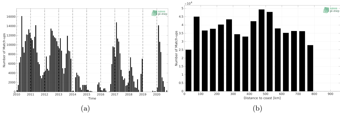
Figure 1: Number of match-ups between Surface drifters and SMOS SSS L3 v8 - 9 Days (CATDS-CECOS-LOCEAN) SSS as a function of time (a) and as function of the distance to coast (b) over the SMOS coastal zone (<800km) 60N-60S Pi-MEP region and for the full satellite product period.
